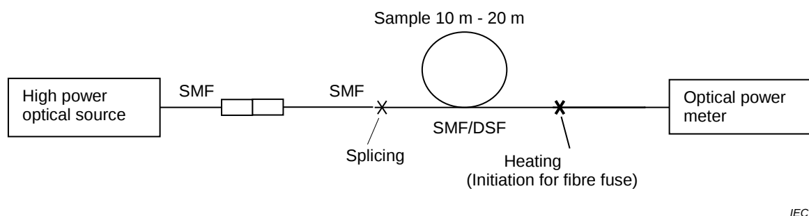
Figure 1 – Experimental set-up for fibre fuse propagation
