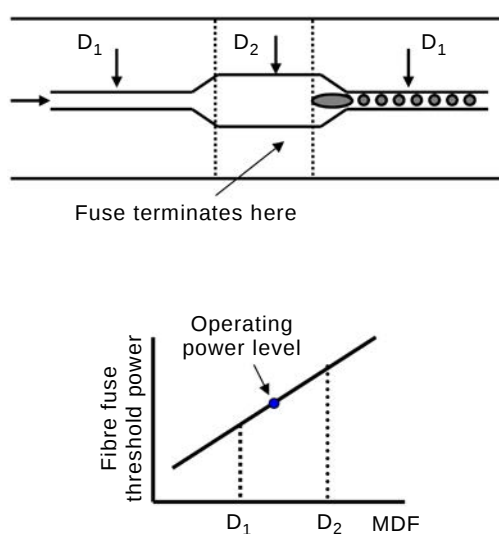
Figure A.8a – Principle of the optical fibre fuse passive termination method
