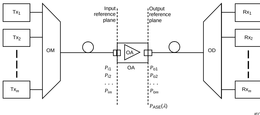
Figure 2 – Optical amplifier in a multichannel application
