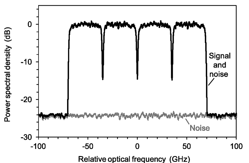
Figure 4 – Optical power spectrum of a 400 Gbit/s optical "superchannel" comprised of four very densely spaced 100 Gbit/s PM-QPSK signals
