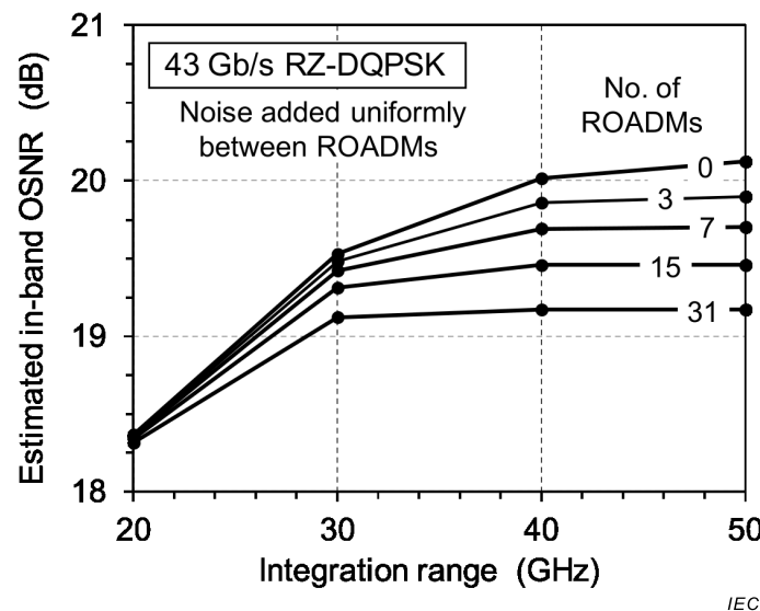
Figure 10 – Impact of integration range on R_{\text{int}} for 43 Gbit/s RZ-DPSK signals in a ROADM network
