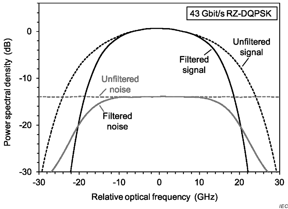
Figure 8 – Optical power density spectra of signal and ASE noise after filtering in a ROADM network with intermediate amplification
