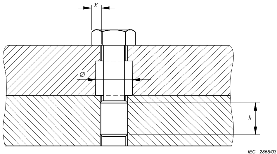
Figure 2 – Tolerances and clearance for threaded fasteners
