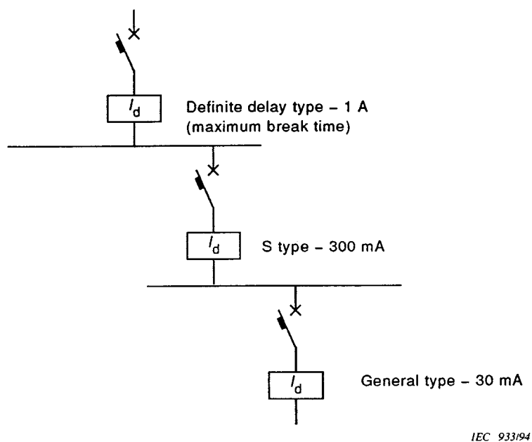
Figure 4 – Example of circuits with three levels of discrimination
