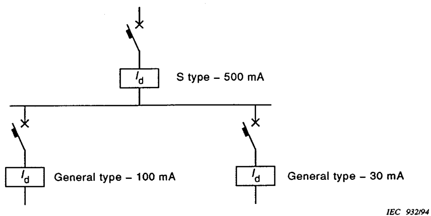
Figure 3 – Example of circuits with two levels of discrimination
