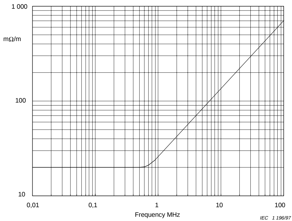
Figure 1 – Maximum transfer impedance
