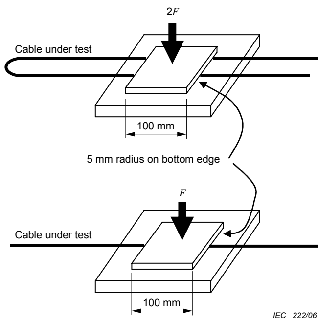
Figure 1 – Crush test equipment
