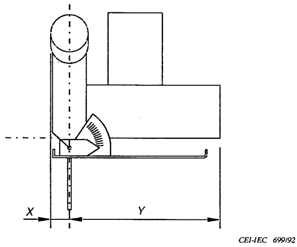
Figure 5 – Aptitude à scier le long d'un mur Ability to cut along walls
