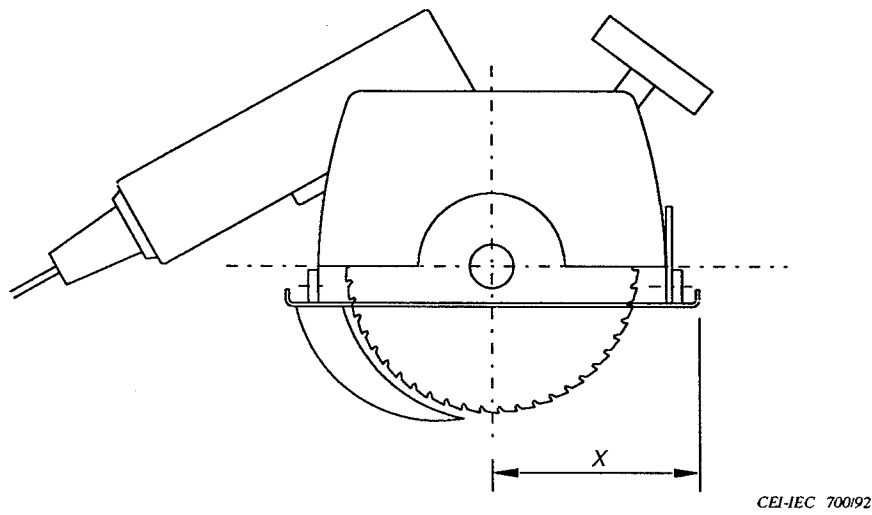
Figure 6 – Aptitude à scier vers un mur Ability to cut towards walls
