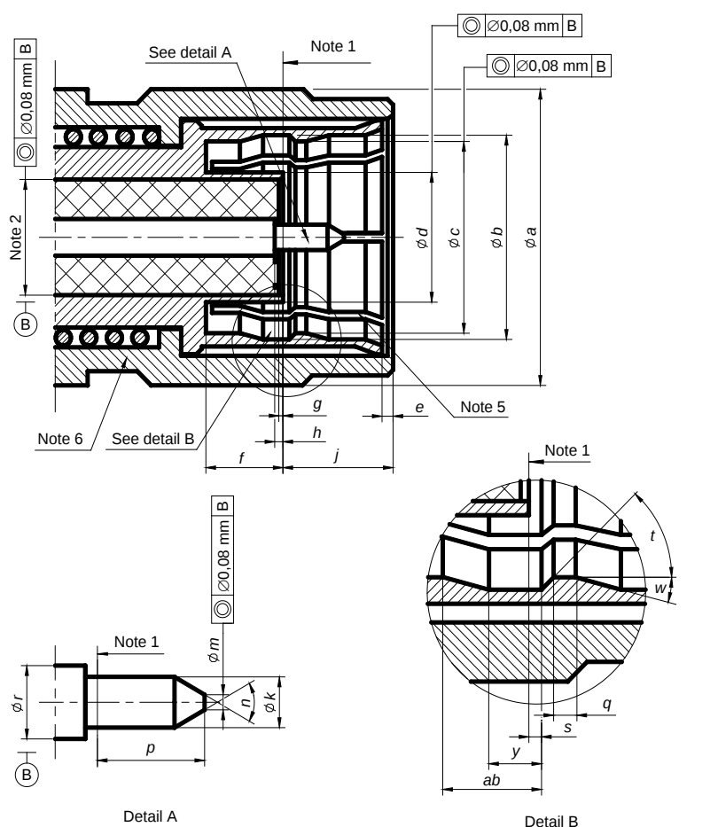
Figure 5 – Connector with pin-centre contact (for dimensions and notes, see Table 5)
