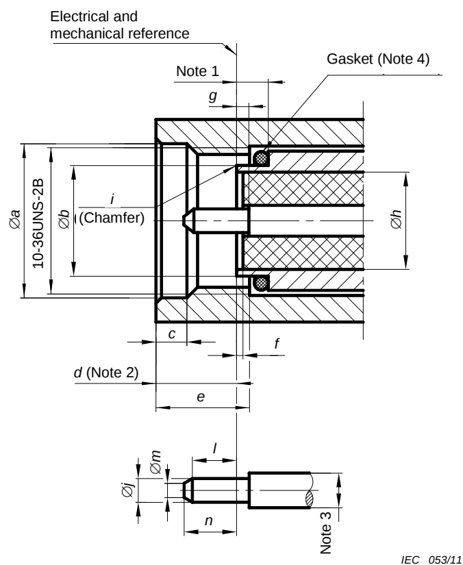
Figure 1 – Connector with pin-centre contact (for dimensions and notes, see Table 1)
