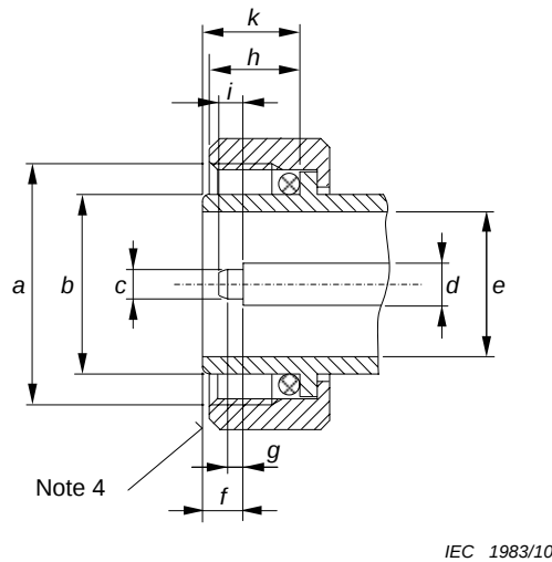
Figure 1 – Connector with pin centre contact (for dimensions, see Table 1)
