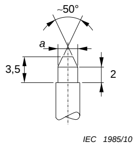
Figure 3 – Gauge pins for centre contact of socket connector
