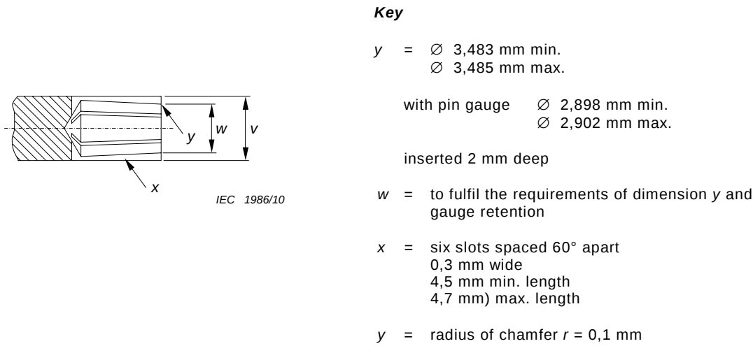
Figure 4 – Slotted centre contact
