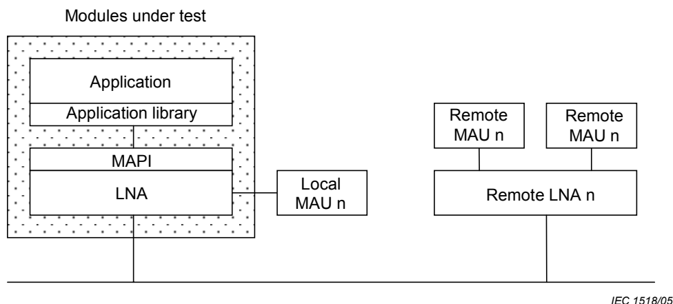
Figure 3 – Test topology
