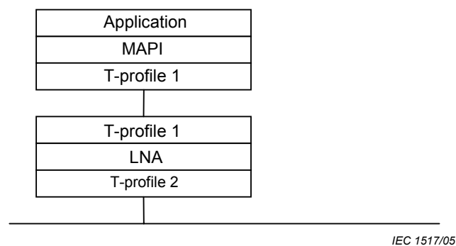
Figure 2 – Message flow in IEC 61162-4 system
