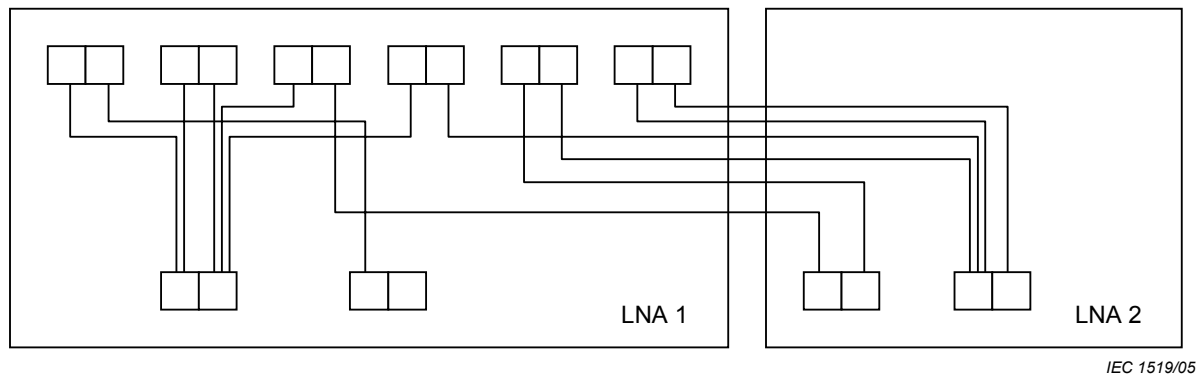
Figure 4 – Multiple client/server connections
