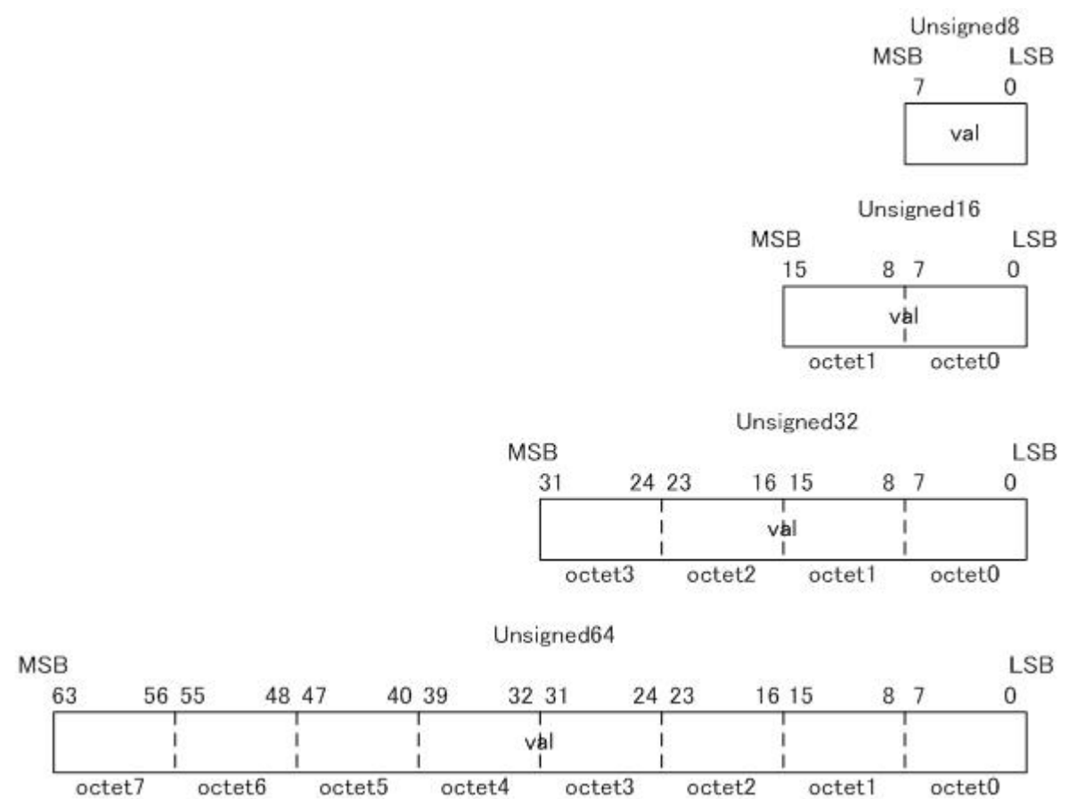
Figure 4 – Encode of Unsigned subtypes
