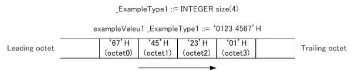
Figure 3 – Example of transfer of INTEGER value
