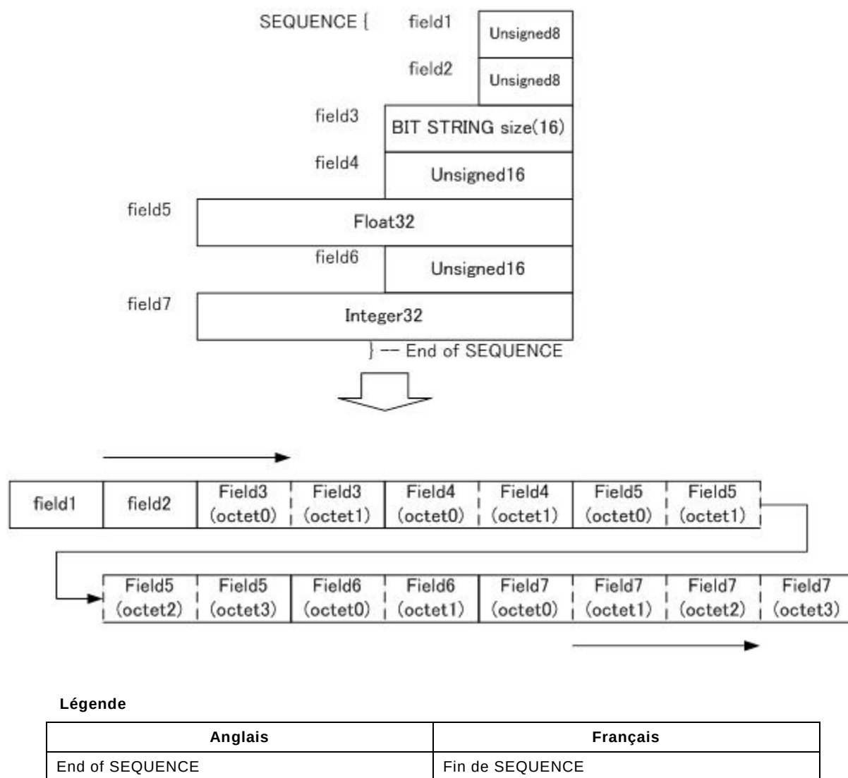
Figure 9 – Codage du type SEQUENCE
