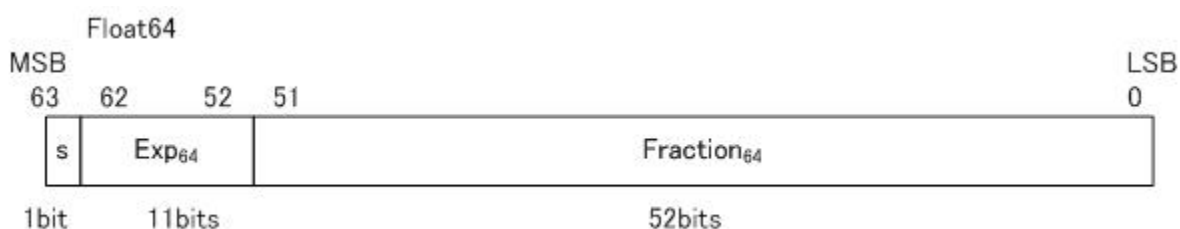
Figure 6 – Codage du type Float64
