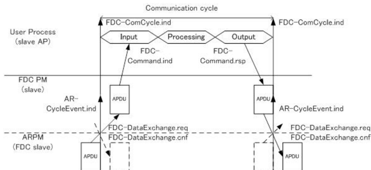
Figure 13 – Example communication cycle of FDC slave AP
