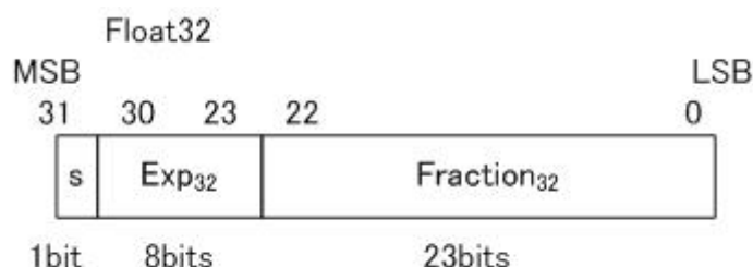
Figure 5 – Codage du type Float32
