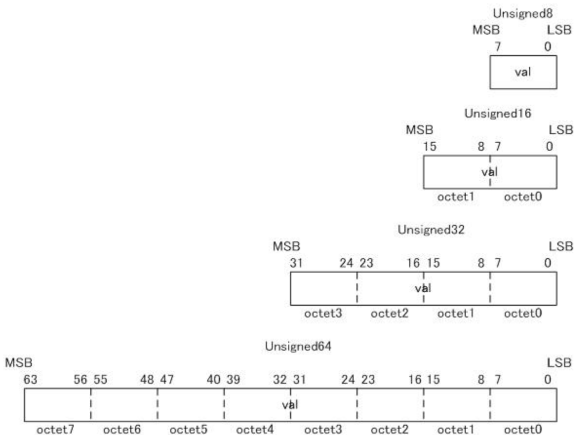
Figure 4 – Codage des sous-types Unsigned
