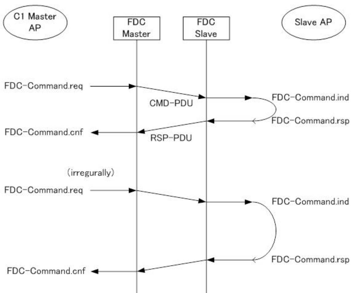
Figure 17 – Event-driven communication
