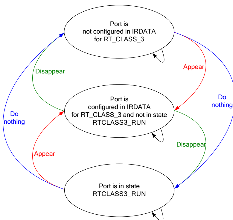
Figure 68 – State transition diagram for generating events
