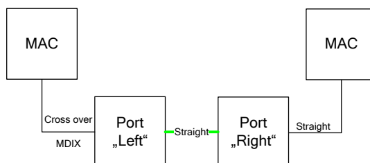
Figure R.2 – Scheme of 2-ports
