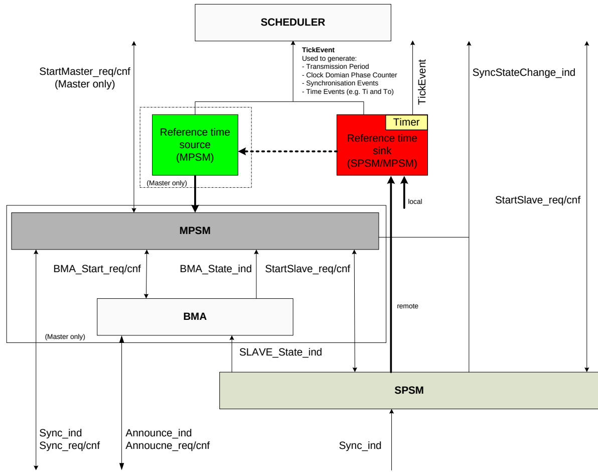
Figure 42 – Overview of PTCP
