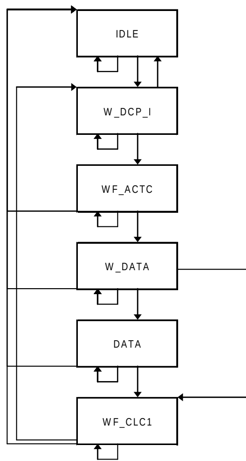
Figure 109 – State transition diagram of CMDMC
