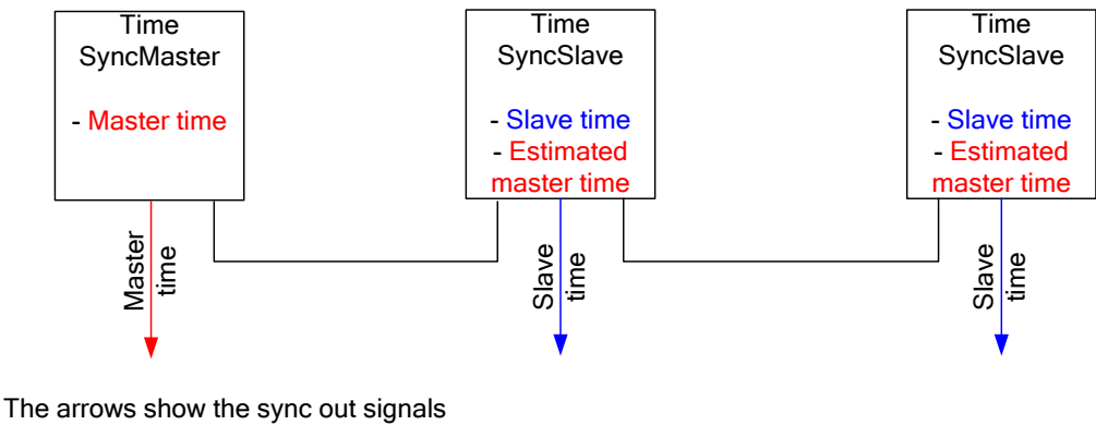
Figure 89 – Toplevel view to the time PLL window
