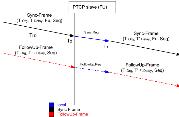
Figure 37 – FU Sync Slave Forwarding Sync- and FollowUp-Frame
