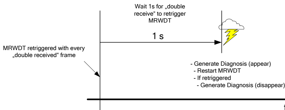
Figure 94 – MediaRedundancyWatchDog expired — appear and disappear
