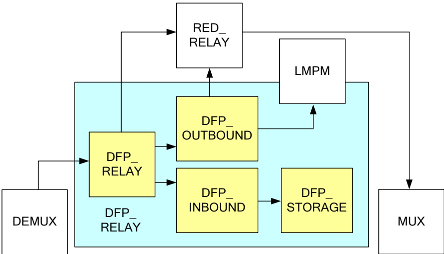
Figure 70 – Diagramme de DFP_RELAY
