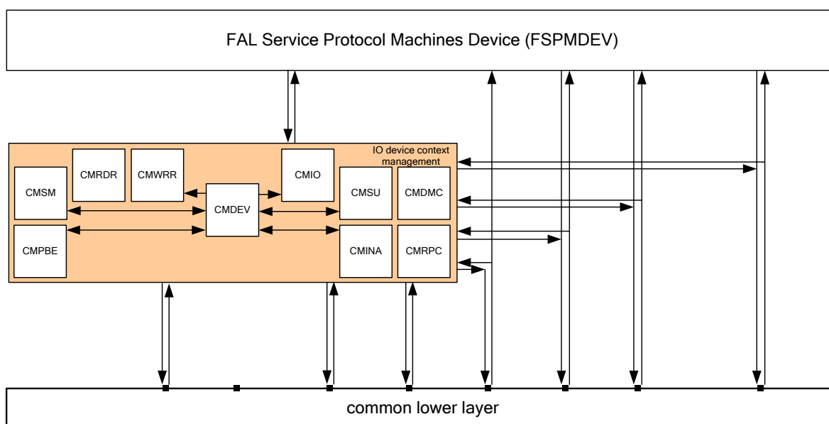
Figure H.2 – Overview of the IO device state machines
