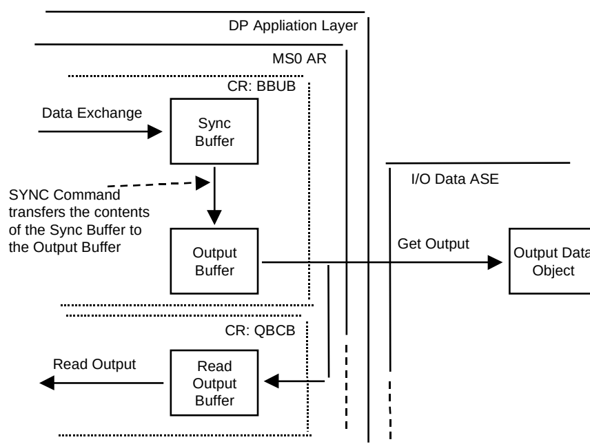
Figure 32 – Output buffer model of a DP-slave with sync functionality
