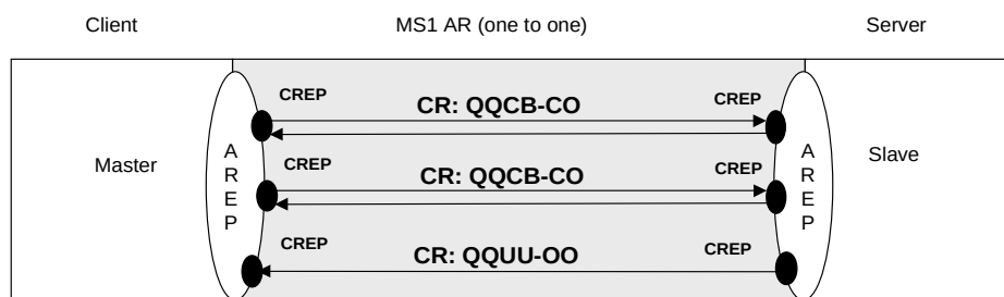
Figure 35 – MS1 application relationship
