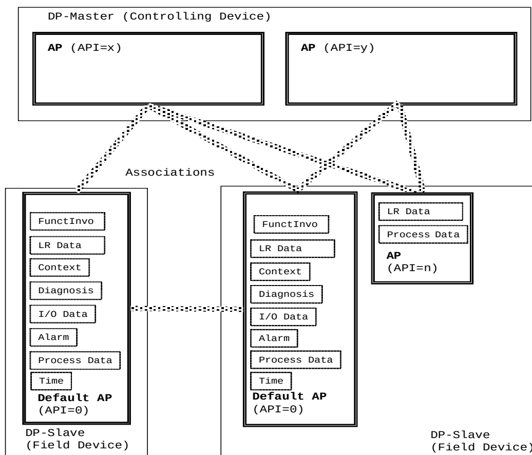
Figure 6 – Overview of application processes
