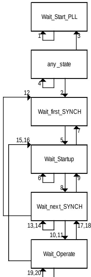
Figure 21 – PLL state diagram
