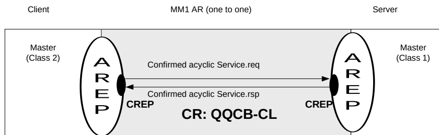
Figure 42 – MM1 application relationship
