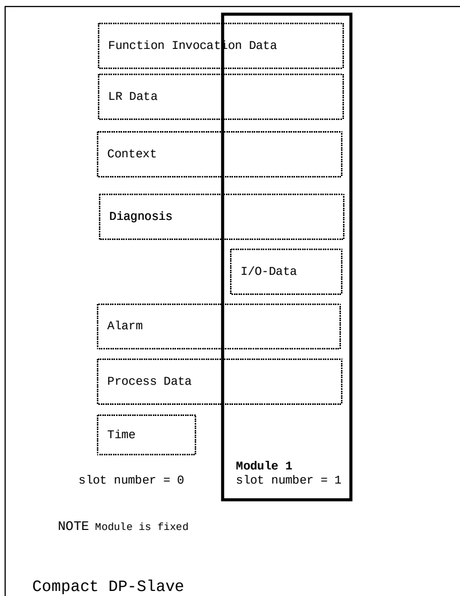
Figure 5 – DP-slave model (compact DP-slave)
