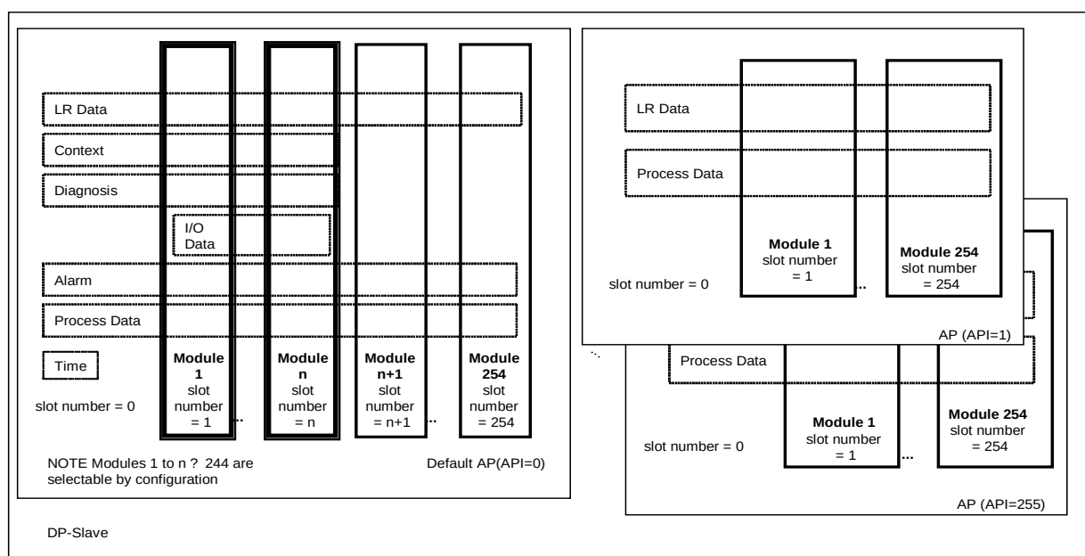
Figure 7 – DP-slave model (modular DP-slave)
