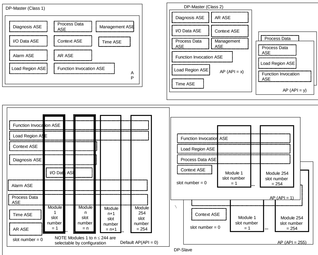
Figure 8 – Application Service Elements (ASEs)
