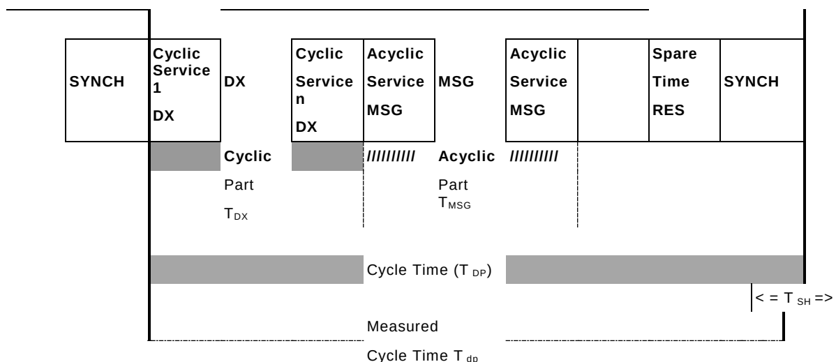
Figure 15 – Sequence of an isochronous DP cycle with one DP-master (class 1)
