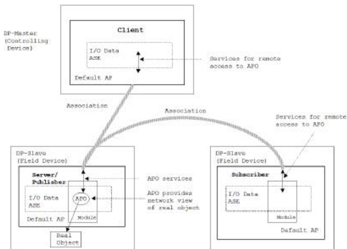
Figure 11 – Access to a remote APO for publisher/subscriber association
