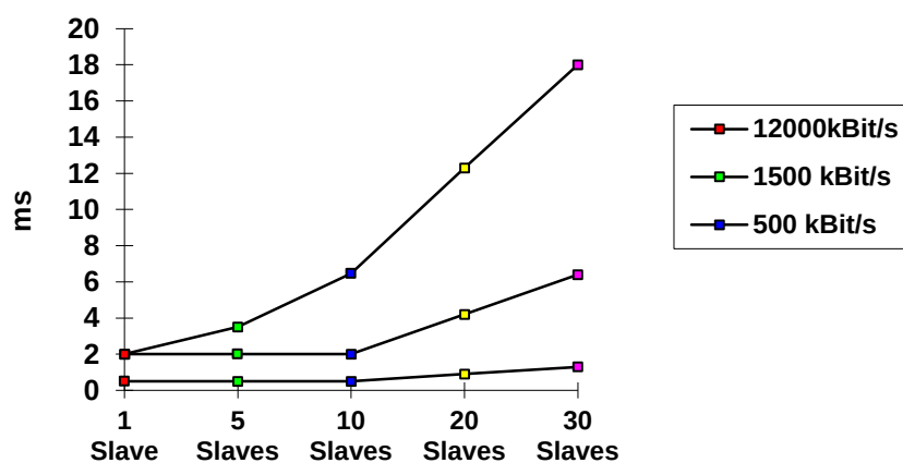
Figure 44 – Cycle time of the DP system
