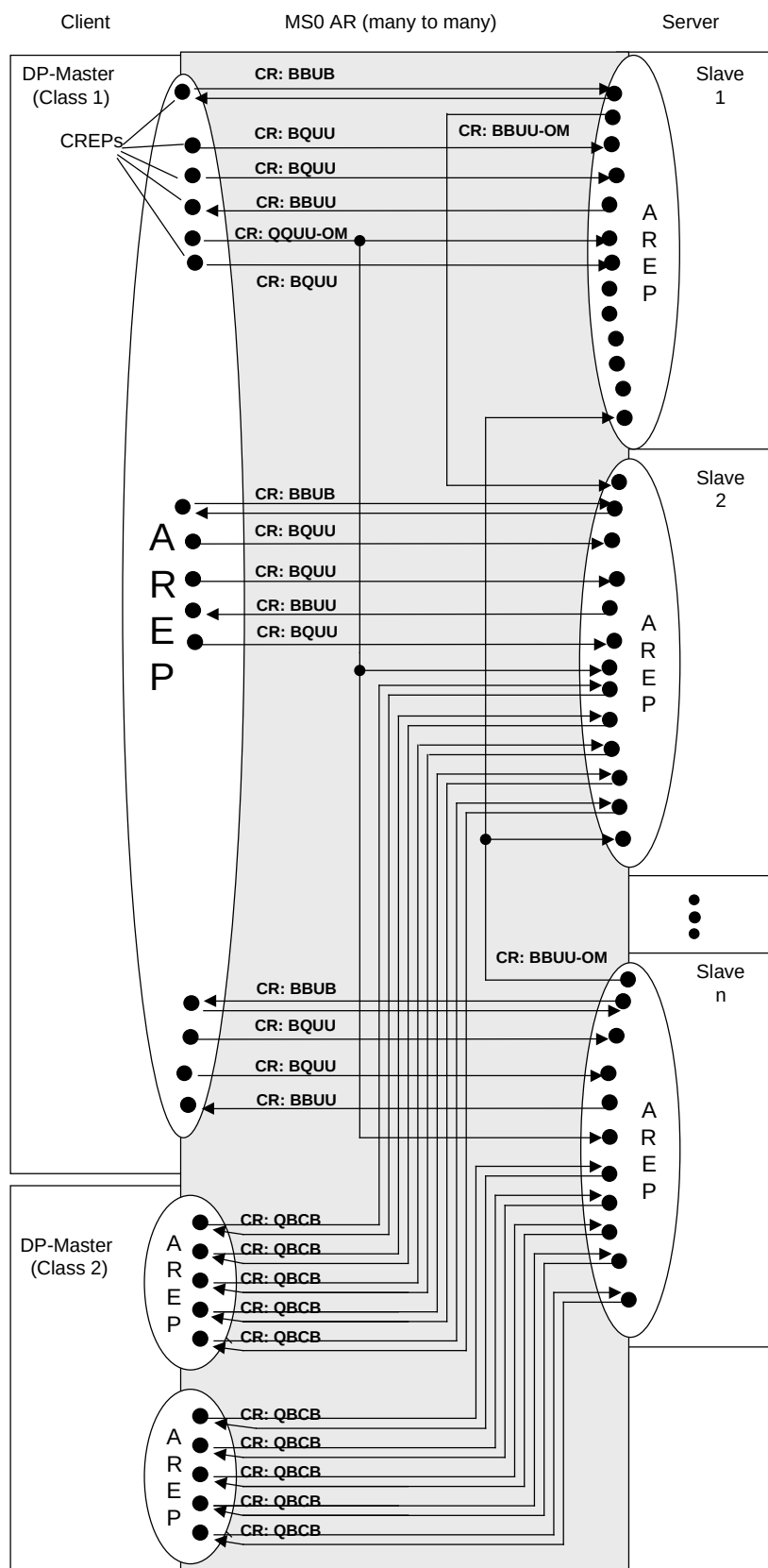
Figure 30 – MS0 application relationship
