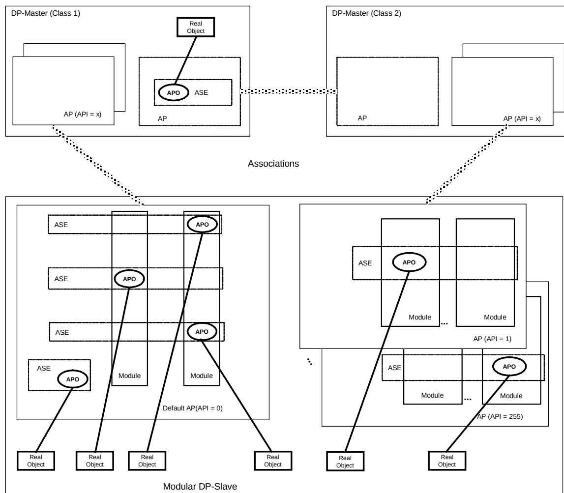
Figure 9 – Application Process with application Objects (APOs)
