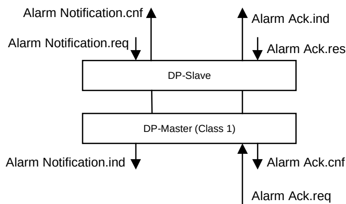
Figure 24 – Treatment of an alarm in the DP system
