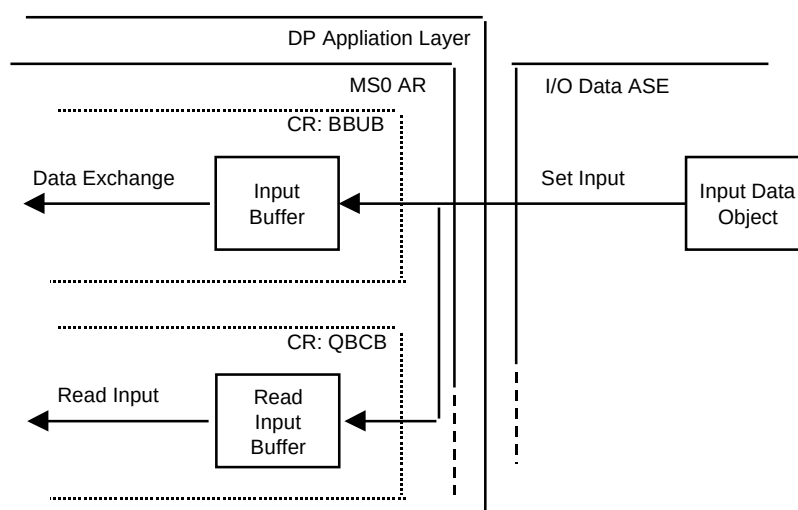
Figure 33 – Input buffer model of a DP-slave without freeze functionality
