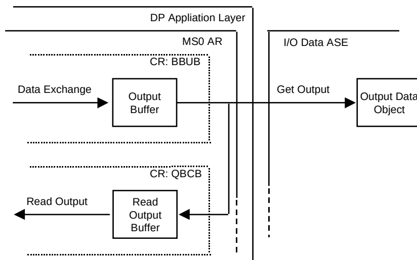
Figure 31 – Output buffer model of a DP-slave without sync functionality
