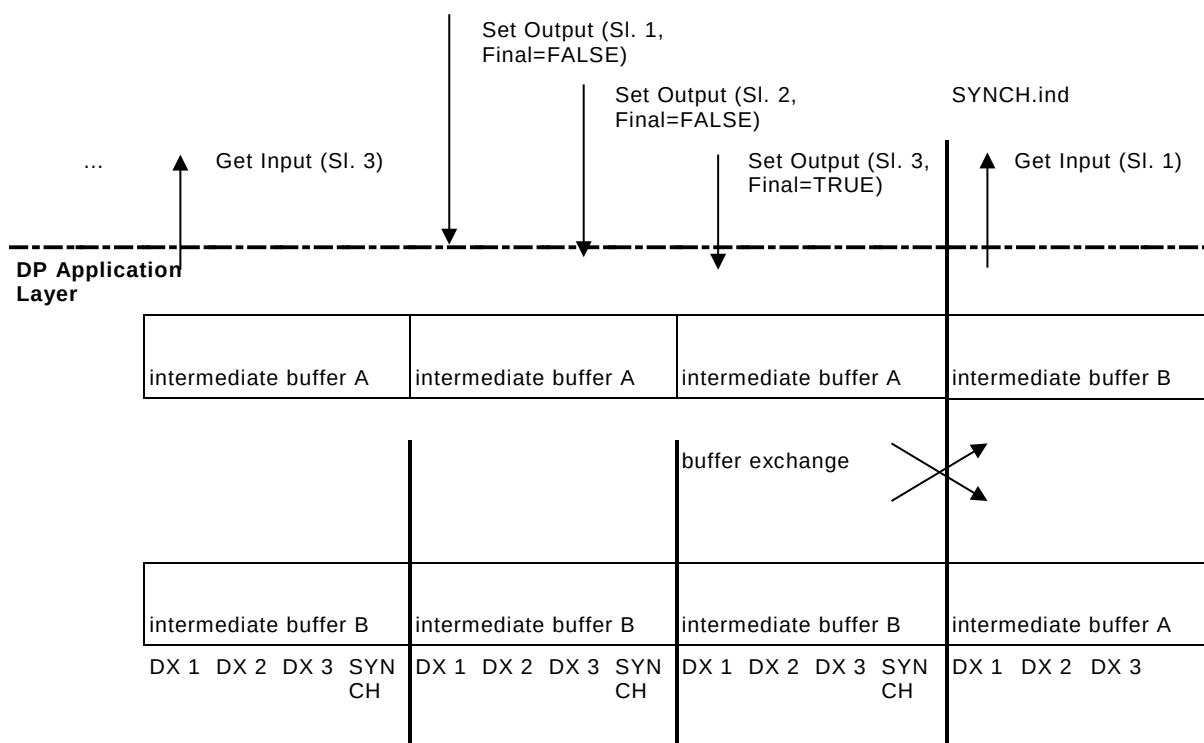
Figure 18 – Buffered synchronized isochronous mode at the DP-master (class 1)
