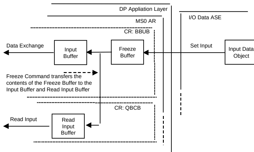
Figure 34 – Input buffer model of a DP-slave with freeze functionality
