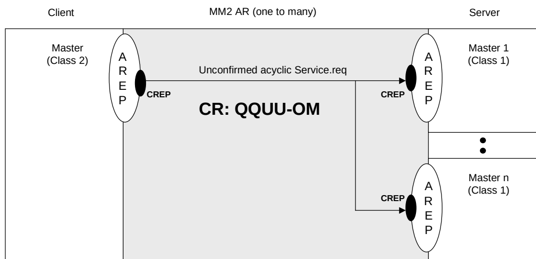
Figure 43 – MM2 application relationship
