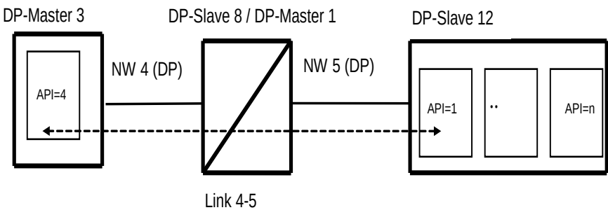
Figure 39 – First example with inter-network addressing
