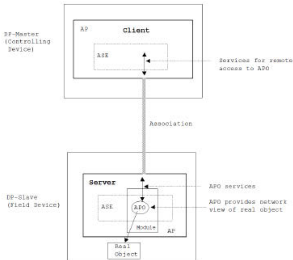
Figure 10 – Access to a remote APO
