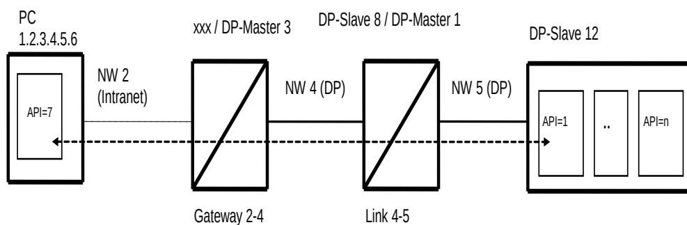
Figure 40 – Second example with inter-network addressing
