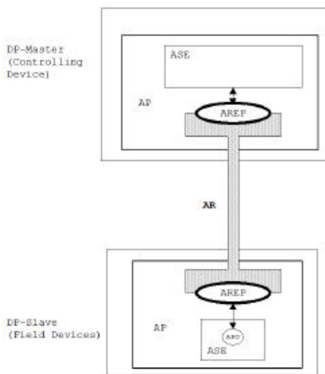
Figure 12 – Example of one AR with two AREPs
