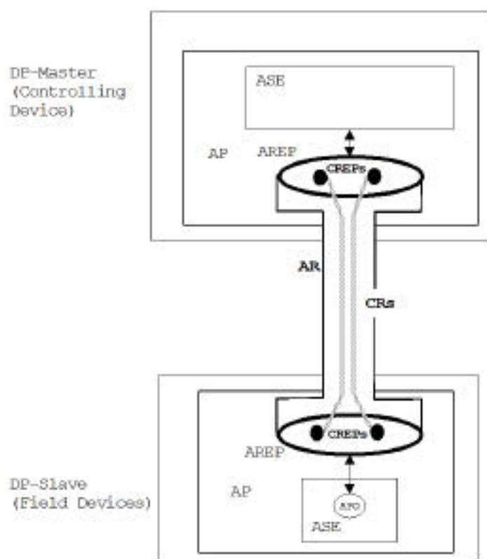
Figure 29 – Assignment of communication relationship to application relationship
