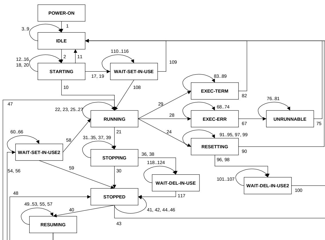
Figure 27 – Function invocation state diagram
