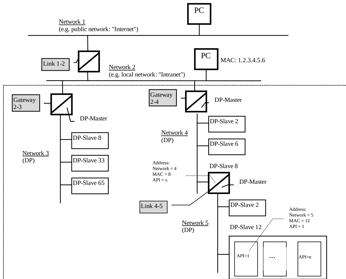
Figure 37 – Example of inter-network communication
