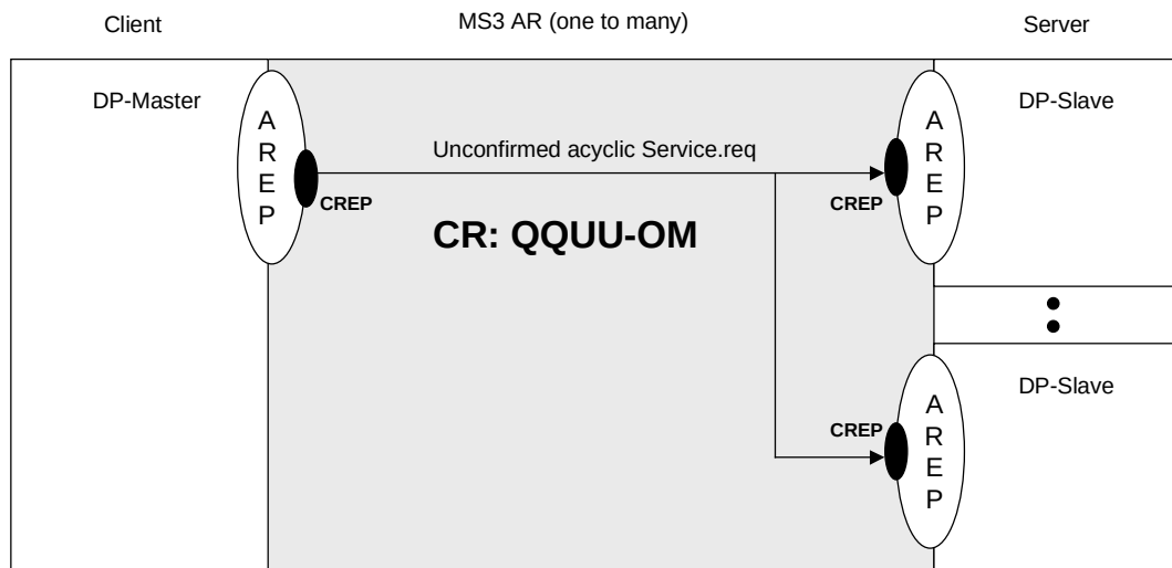
Figure 41 – MS3 application relationship
