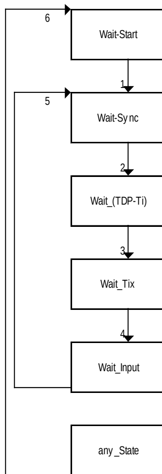
Figure 23 – INPUT state diagram
