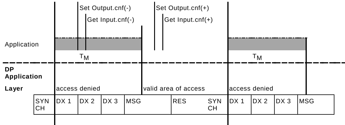
Figure 19 – Enhanced synchronized isochronous mode at the DP-master (class 1)
