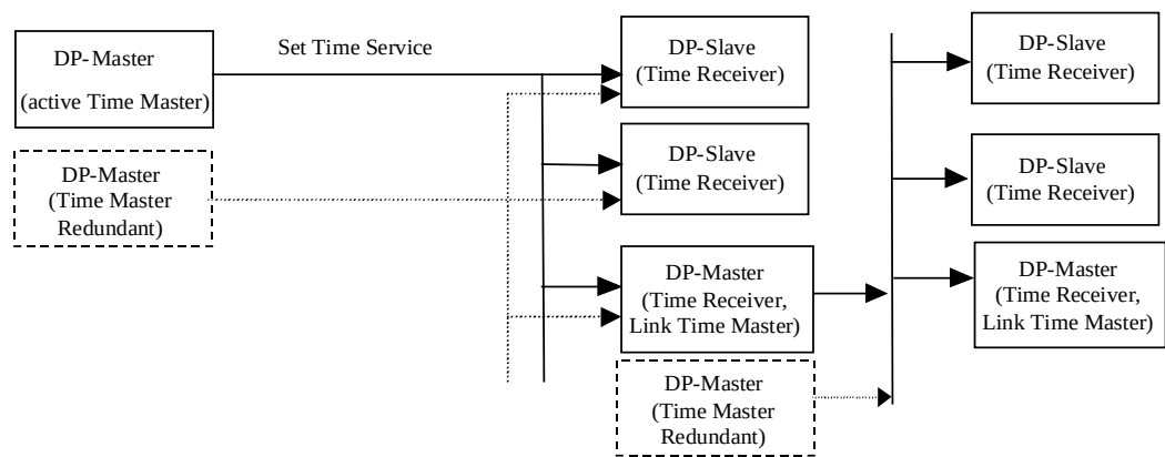
Figure 28 – System architecture
