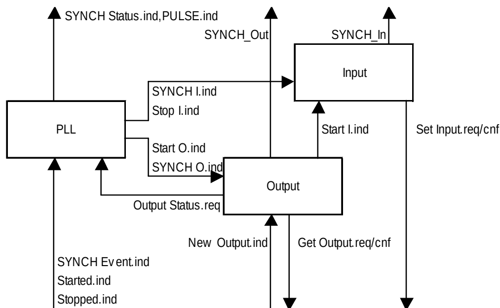
Figure 20 – Input, output and PLL state machine interaction
