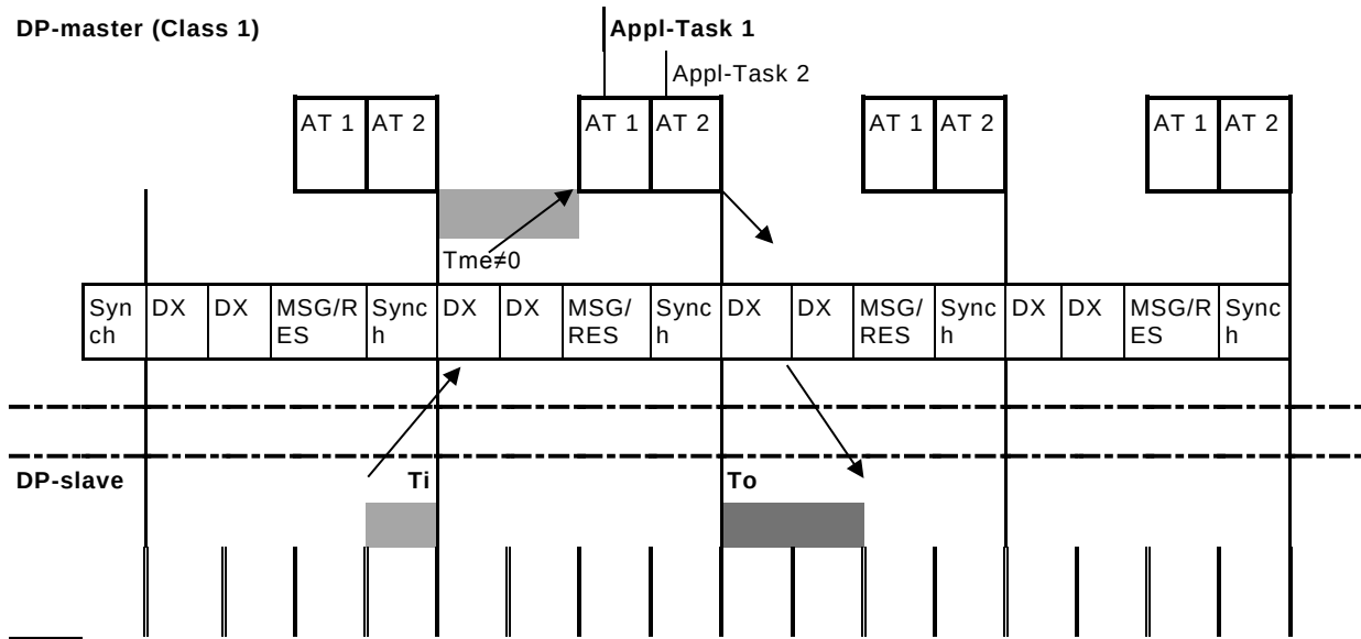
Figure 17 – DP system with optimized isochronous DP cycle
