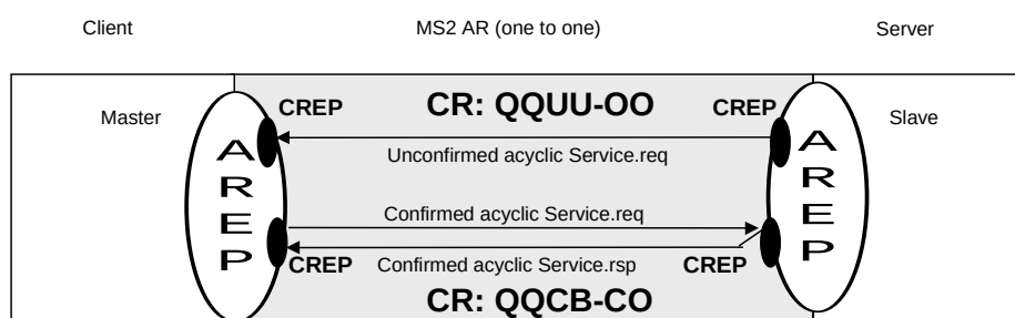
Figure 36 – MS2 application relationship
