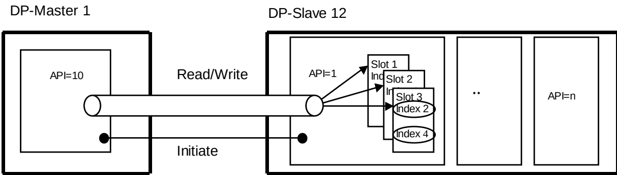
Figure 38 – Example without inter-network addressing
