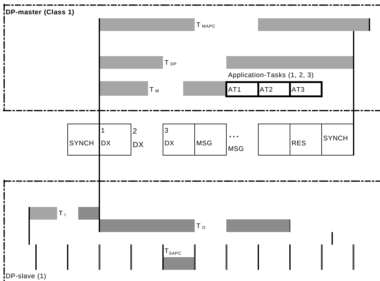
Figure 16 – Additional time relationships in a DP system operating in isochronous mode
