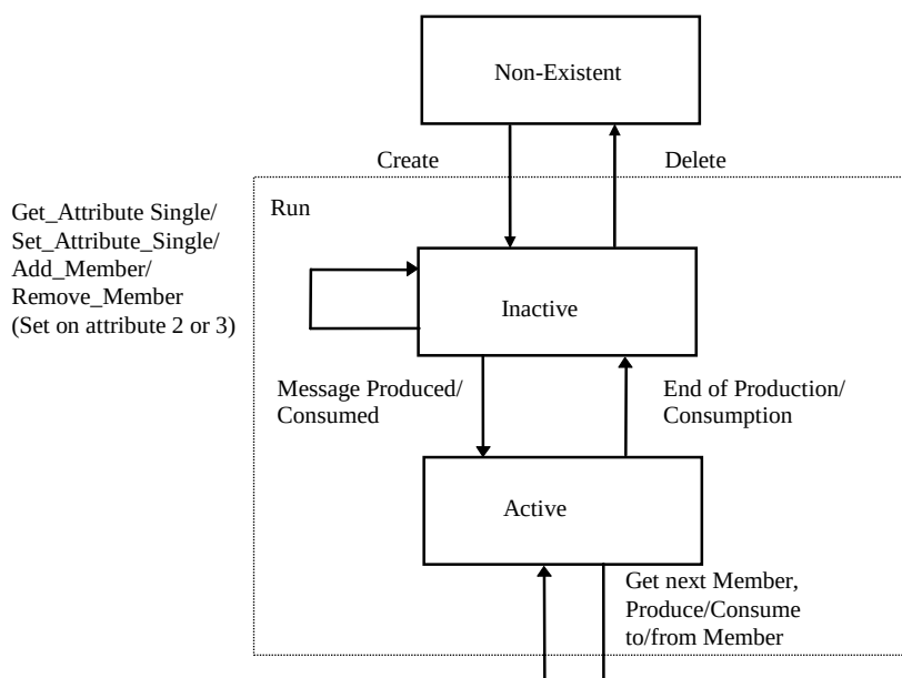
Figure 5 – Dynamic Assembly state transition diagram
