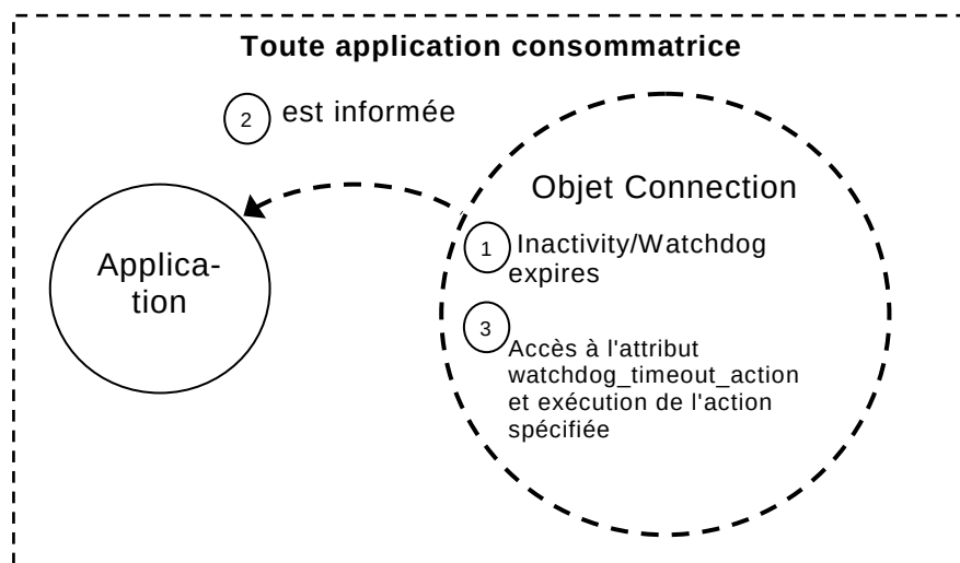
Figure 17 – Inactivity/Watchdog Timer
