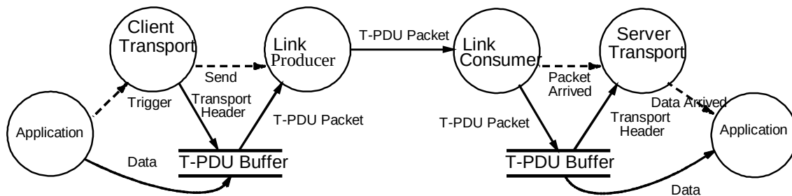
Figure 23 – Data flow diagram for a link consumer
