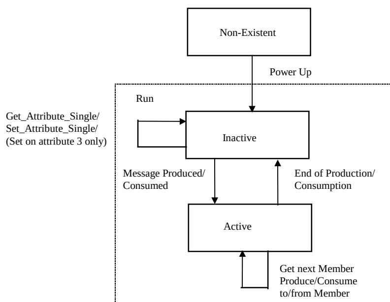
Figure 4 – Static Assembly state transition diagram
