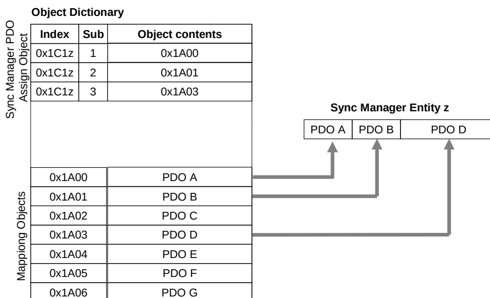
Figure 21 – Sync manager PDO assignment
