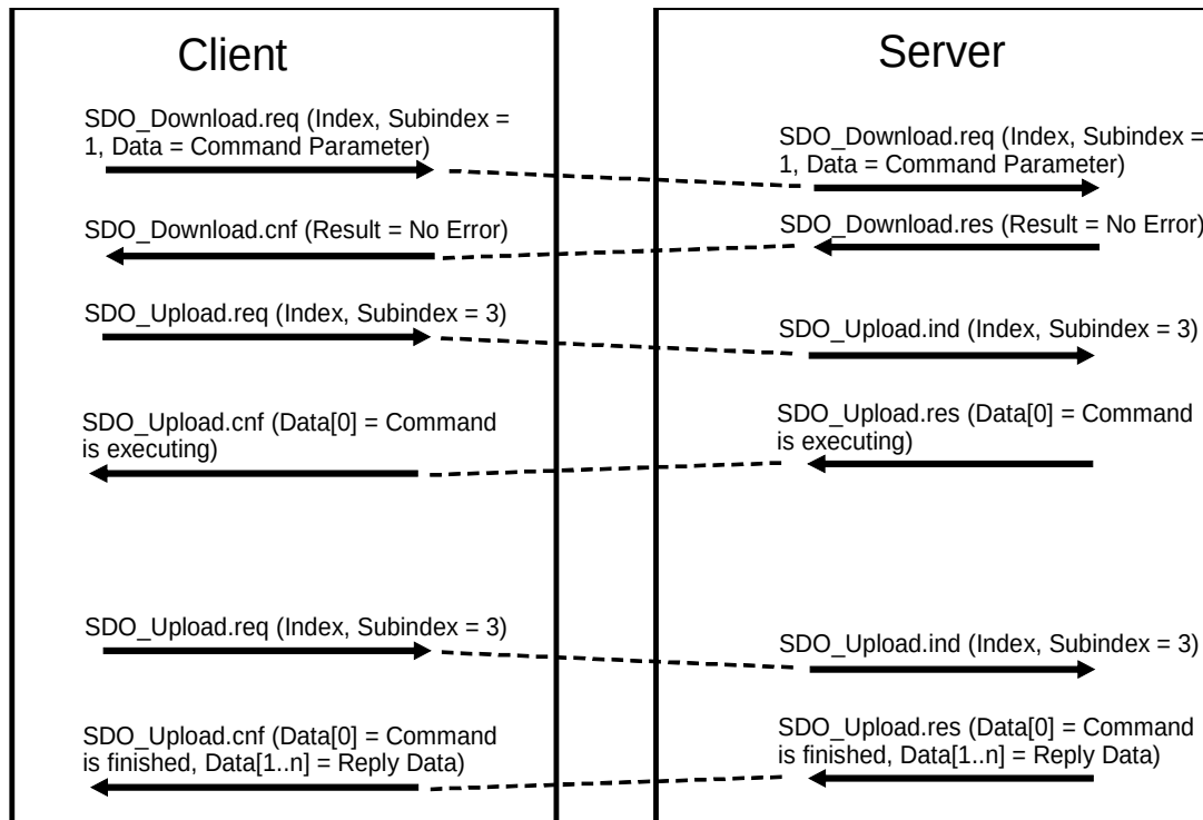
Figure 19 – Command sequence
