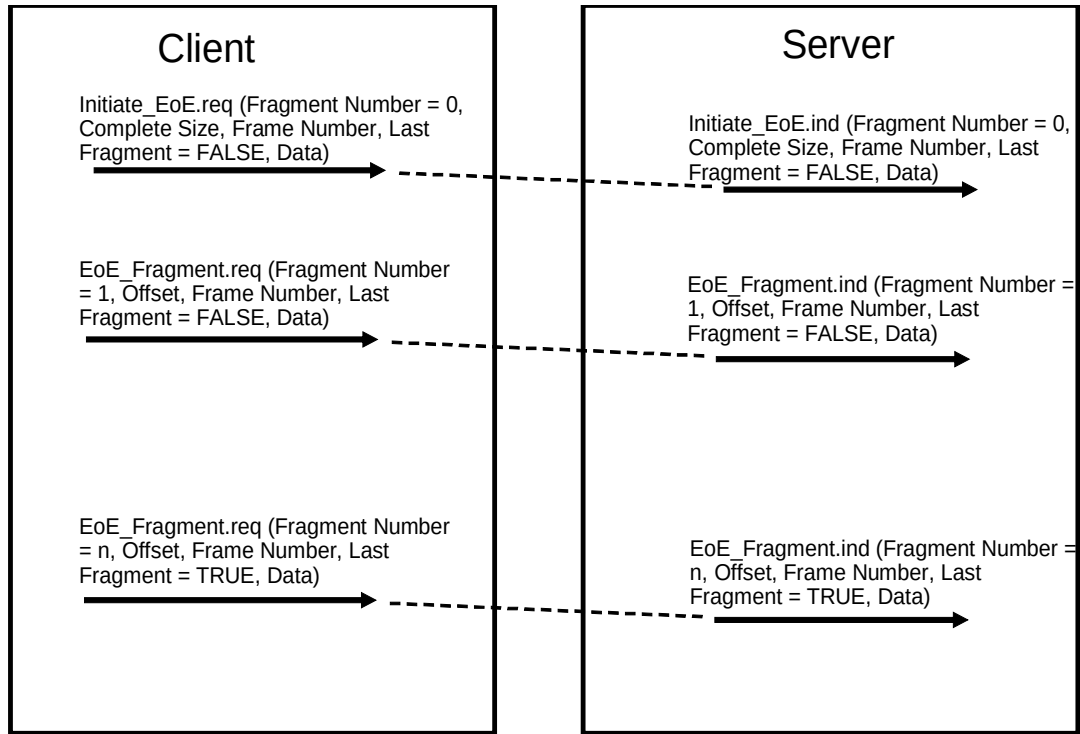
Figure 26 – EoE sequence
