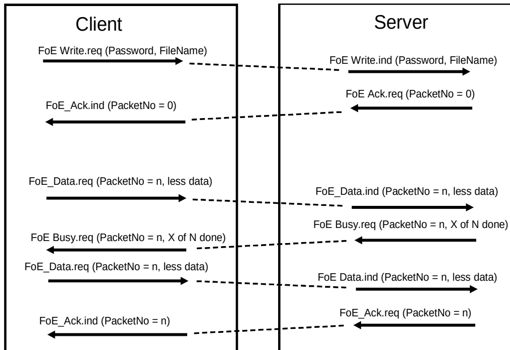
Figure 31 – FoE write sequence with busy
