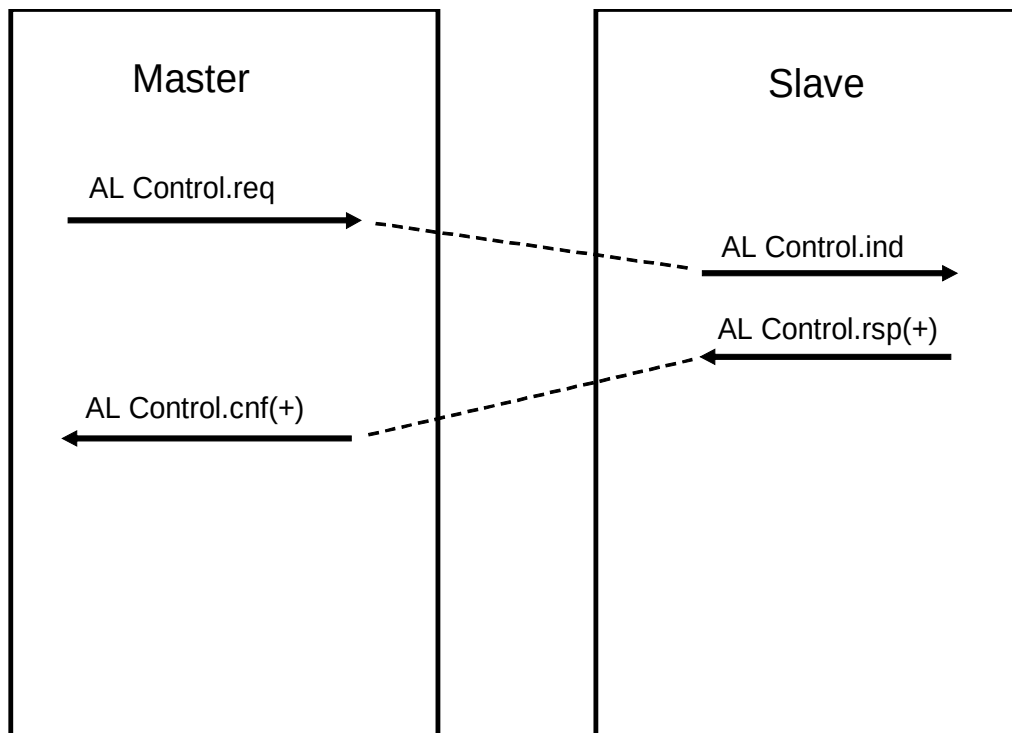
Figure 32 – Successful AL control sequence
