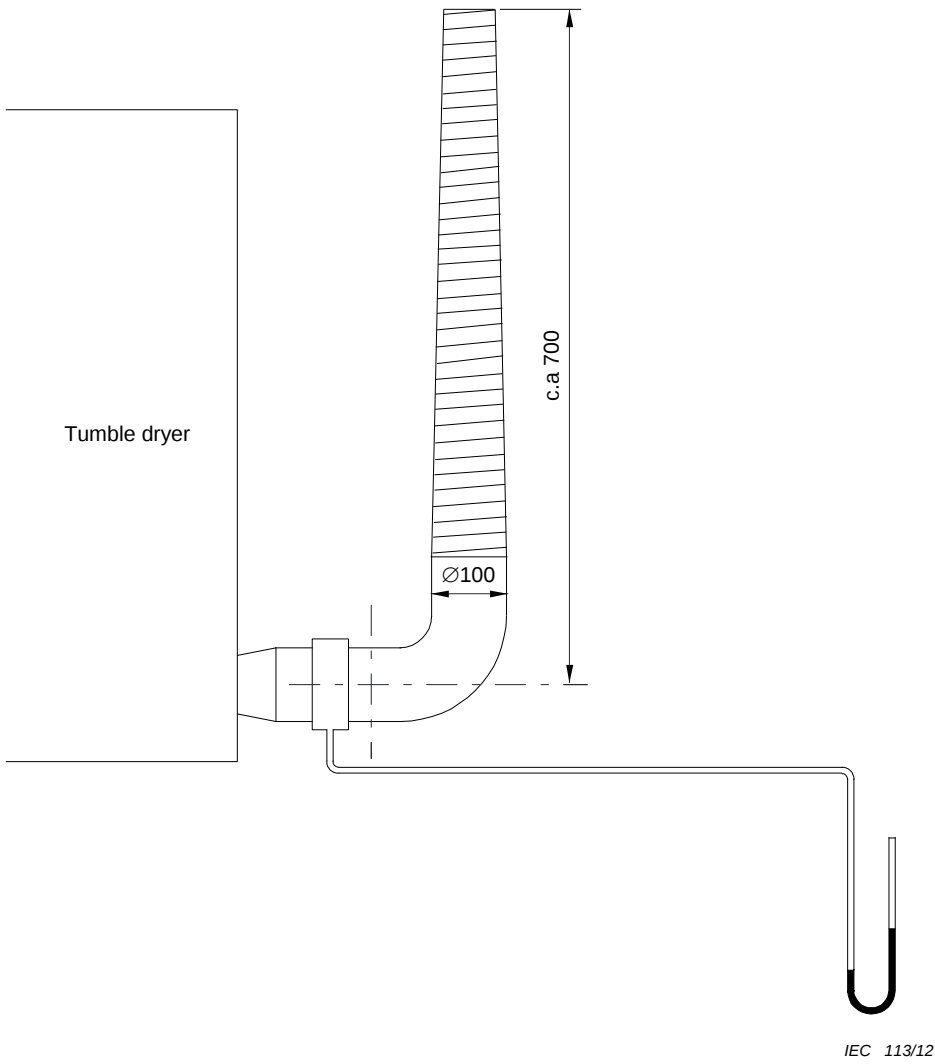
Figure B.3 – Standard exhaust simulator
