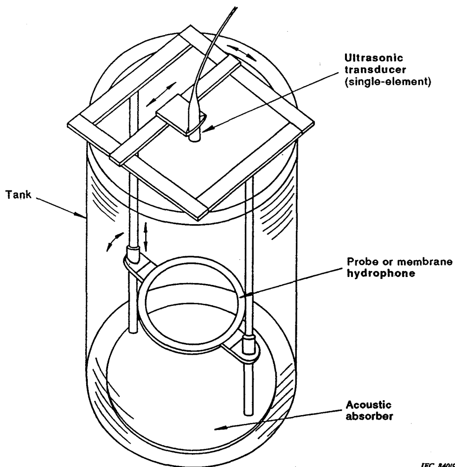
Figure 14 - Schematic diagram of an ultrasonic transducer and hydrophone mount, shown with a limited number of translation and rotation degrees of freedom.
