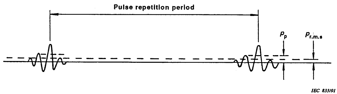
Figure 7 - Schematic diagram showing the pulse and r.m.s. acoustic pressure parameters.
