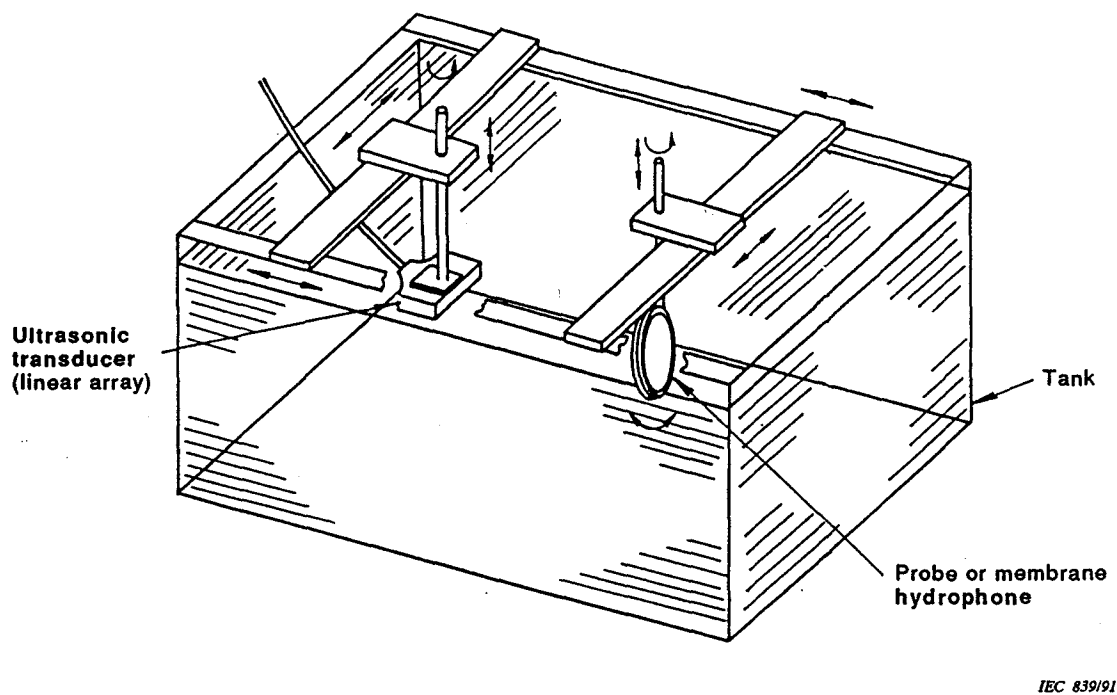
Figure 13 - Schematic diagram of an ultrasonic transducer and hydrophone mount, shown with a full range of degrees of freedom.
