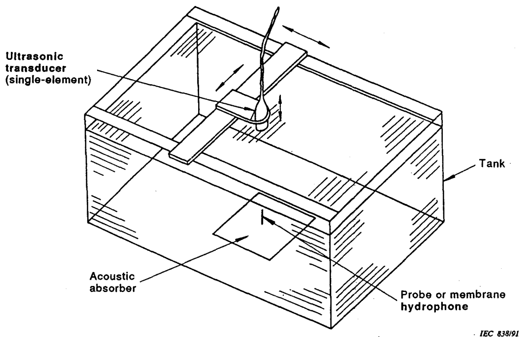
Figure 12 - Schematic diagram of an ultrasonic transducer and hydrophone mount, shown with a limited number of translation and rotation degrees of freedom.
