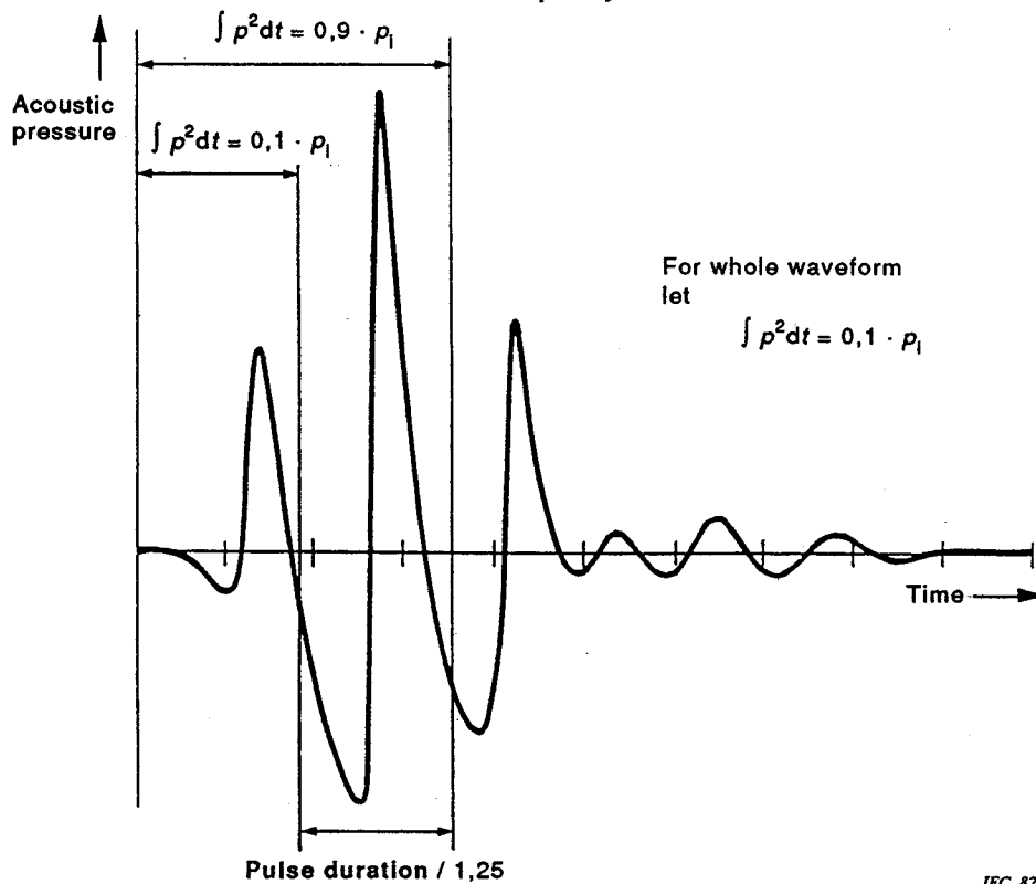
Figure 3 - Schematic diagram showing the method of determining the pulse duration.
