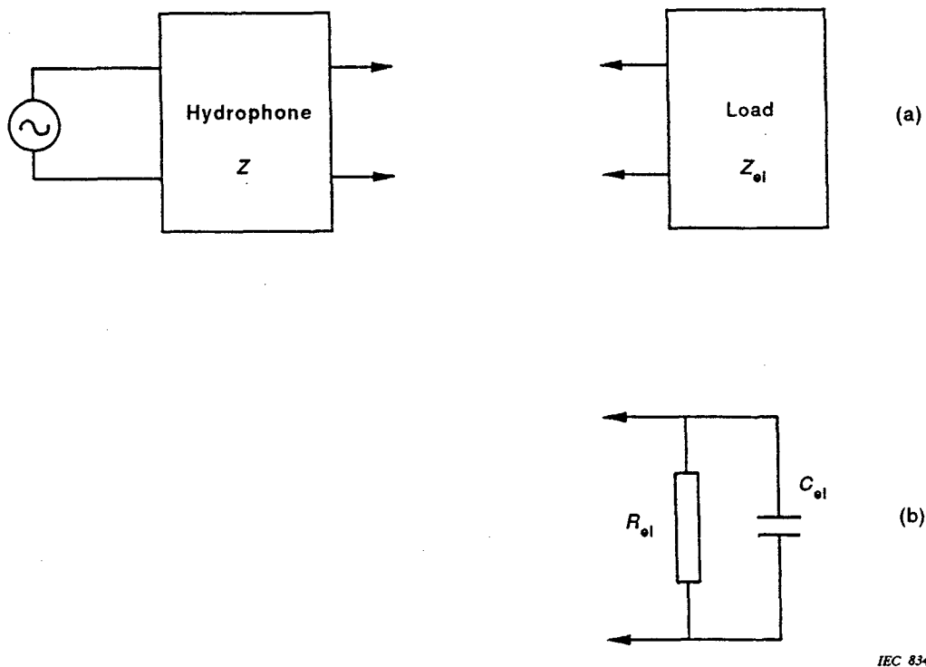
Figure 8 - (a) Simplified equivalent circuit of a hydrophone and electrical load of impedance Z and Z_{el} respectively,
