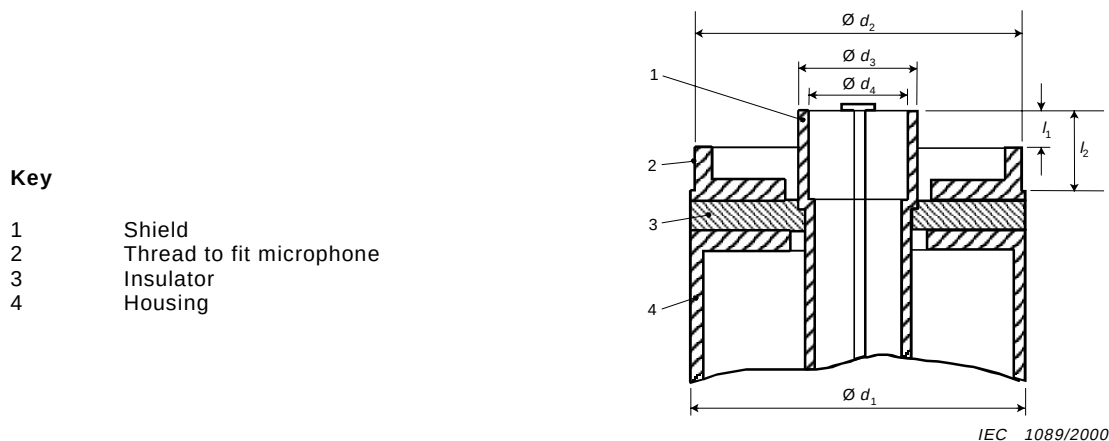
Figure 2 – Mechanical attachment to microphone, showing the ground-shield reference configuration
