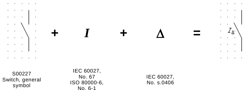
Figure A.10 – Example of a symbol for an RCD
