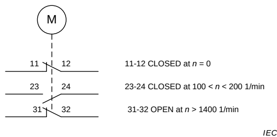
Figure 74 – Symbol of a pilot switch supplemented with a note
