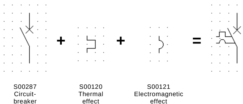
Figure A.6 – Miniature circuit-breaker shown with the symbol for a circuit-breaker qualified with the symbol for thermal and electromagnetic effects
