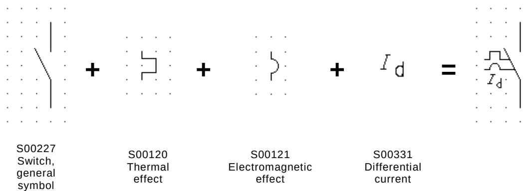
Figure A.8 – Symbol for a miniature circuit-breaker with an RCD, version 2
