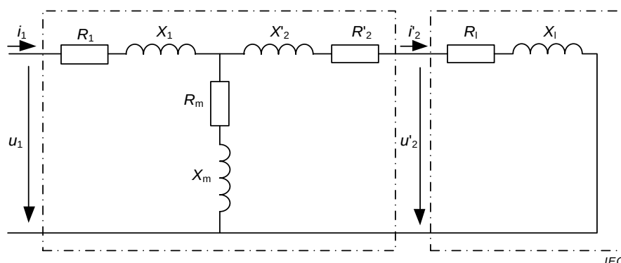
Figure 62 – Example of an equivalent-circuit diagram
