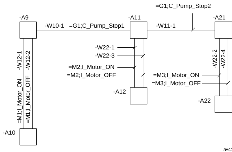
Figure 54 – Examples of reference and signal designations ass. with connecting lines
