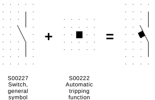
Figure A.3 – Miniature circuit-breaker shown with the general symbol for a switch qualified with the symbol for automatic tripping
