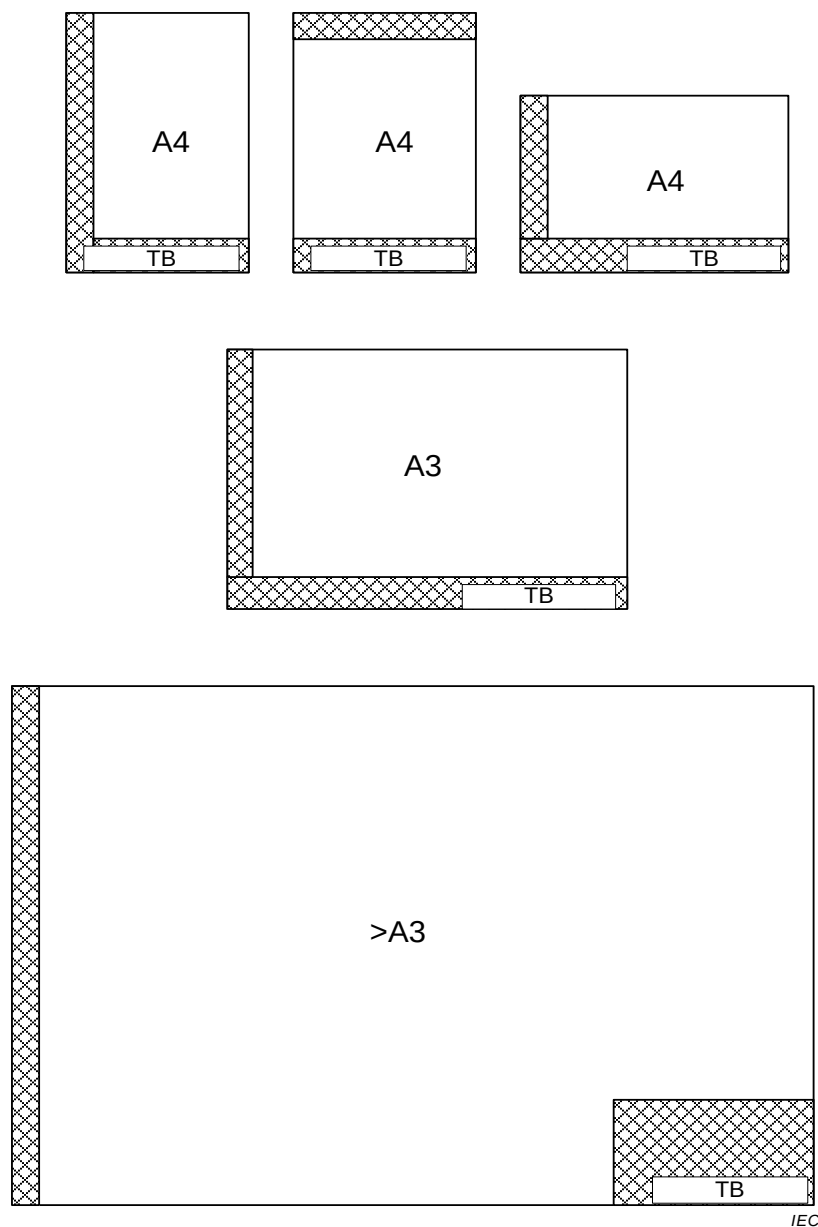
Figure B.3 – Examples of locations of identification areas and possible title blocks
