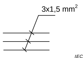
Figure 16 – Example of the use of leader lines to connecting lines
