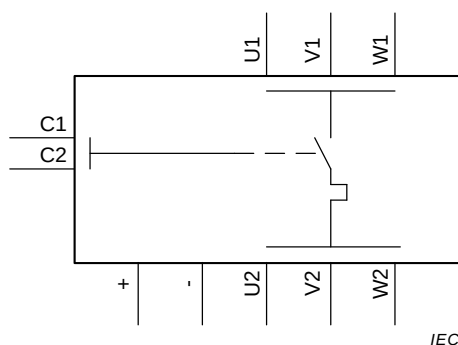
Figure 98 – A symbol for a motor starter
