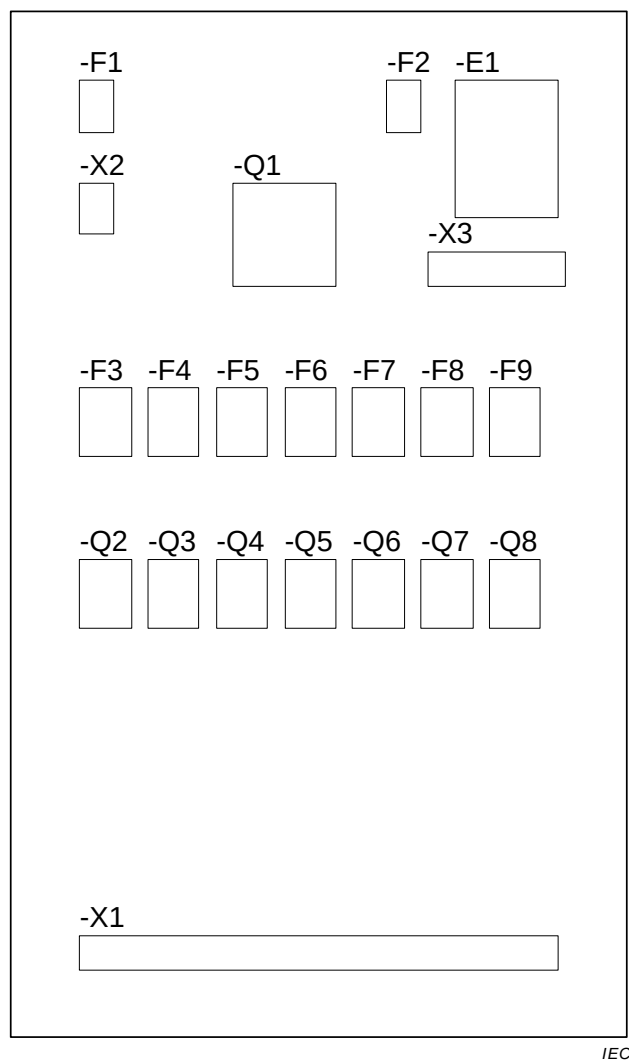
Figure 89 – An arrangement drawing the mounting panel of a cubicle
