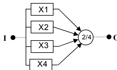
Figure 7 – 2/4 redundancy
