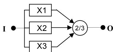
Figure 6 – 2/3 redundancy
