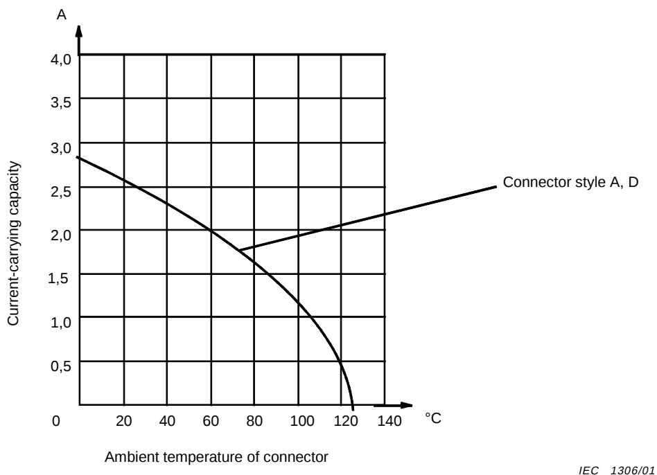
Figure 16 – Current-carrying capacity: derating curve
