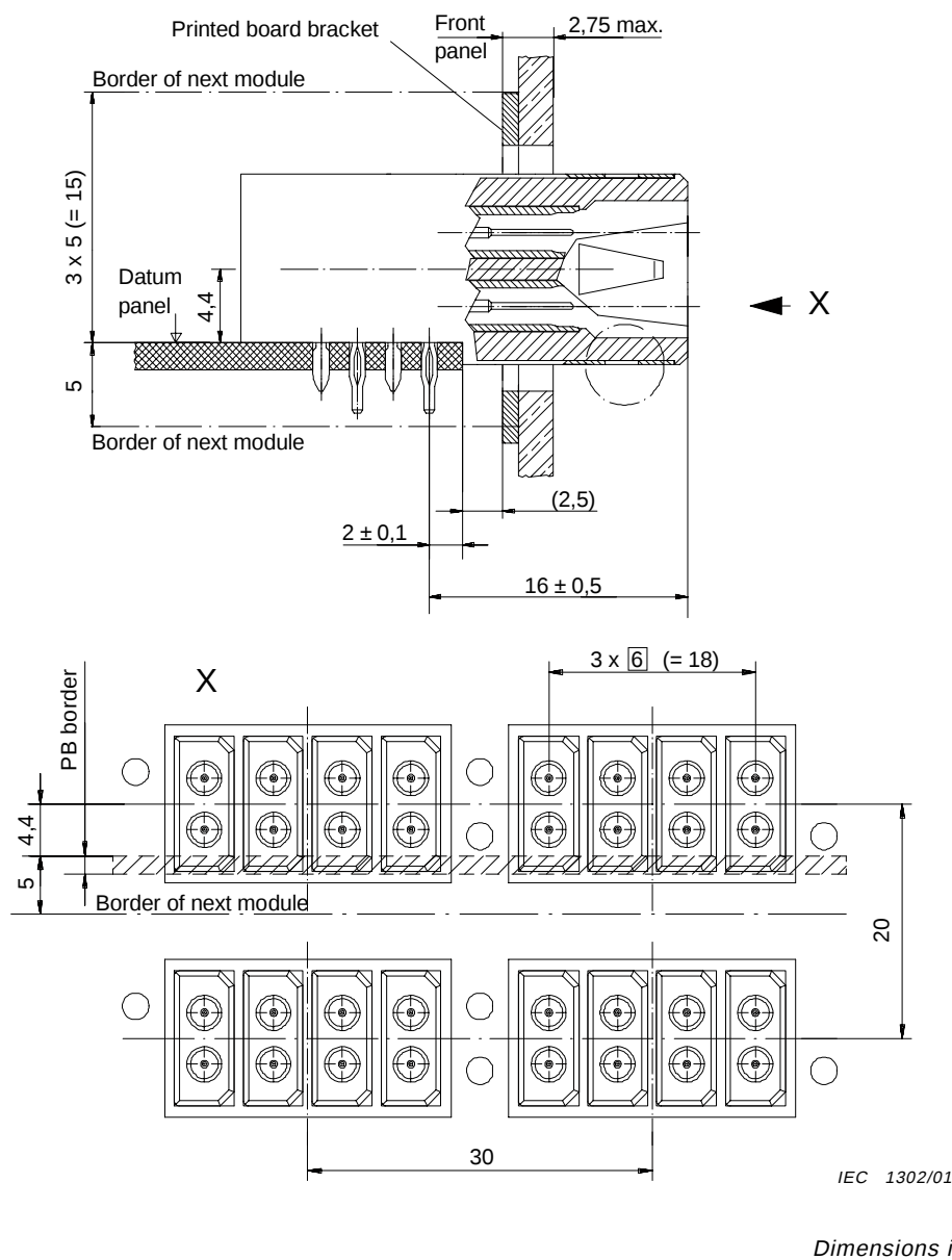
Figure 12 – Fixed board connector with coaxial contacts (style B) panel mounted, packaging information
