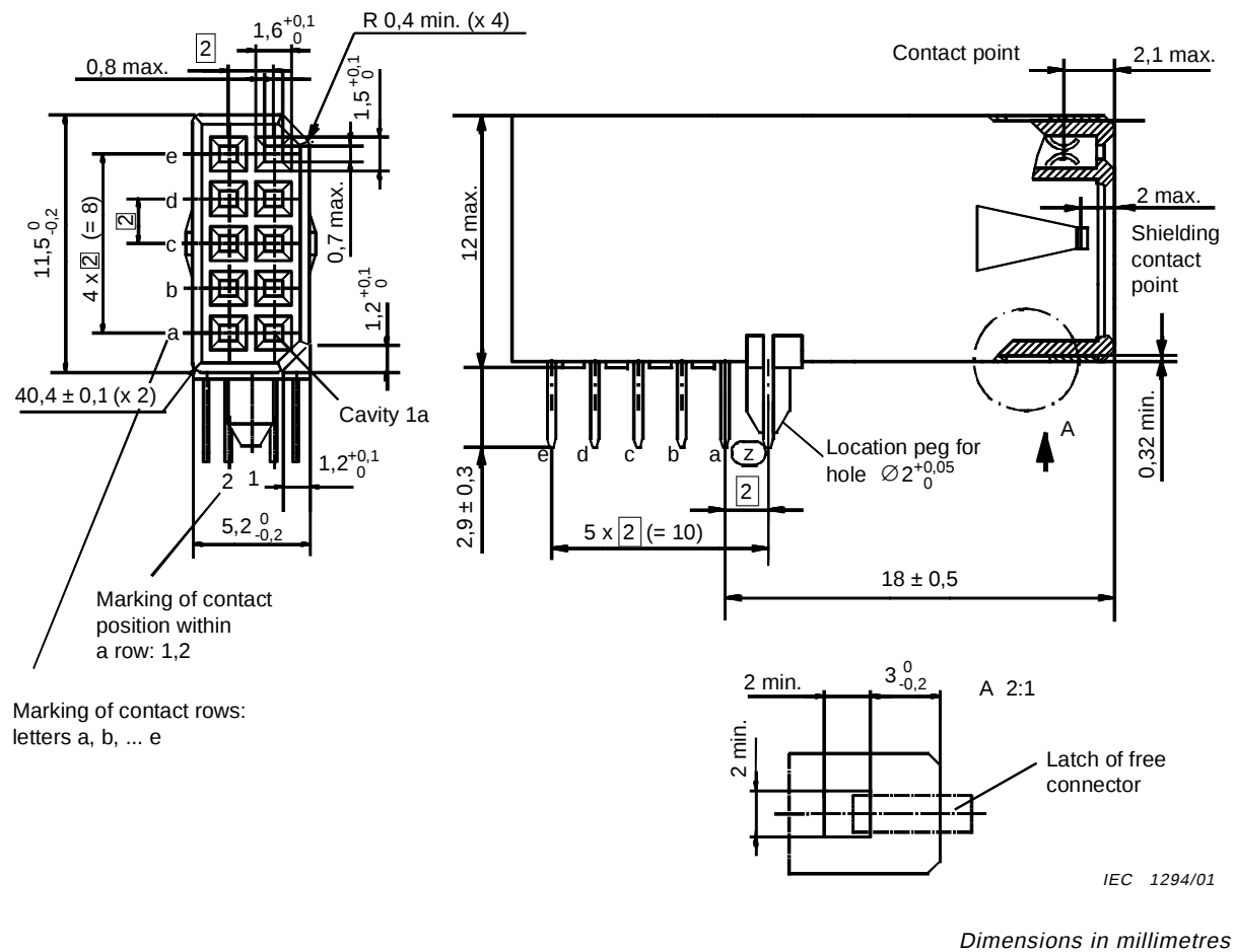
Figure 4 – Fixed board connector with standard contacts
