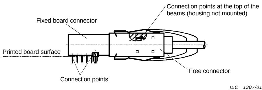
Figure 17 – Points of connection for contact resistance measurement
