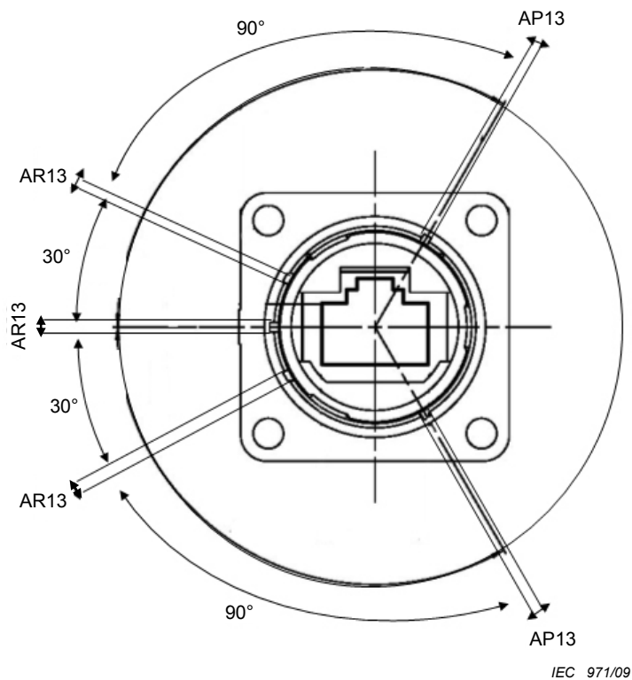
Figure 1 – Dimensions d'embase, variante 12
