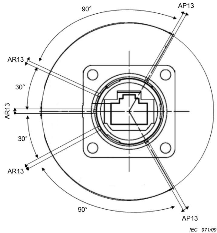
Figure 1 – Dimensions of fixed connector, variant 12
