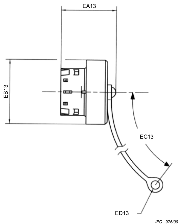
Figure 5 – Variant 12 cap for free connector
