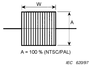
Figure 29 – S chrominance window test signal
