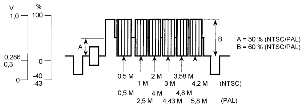
Figure 42 – Measurement of signal levels
