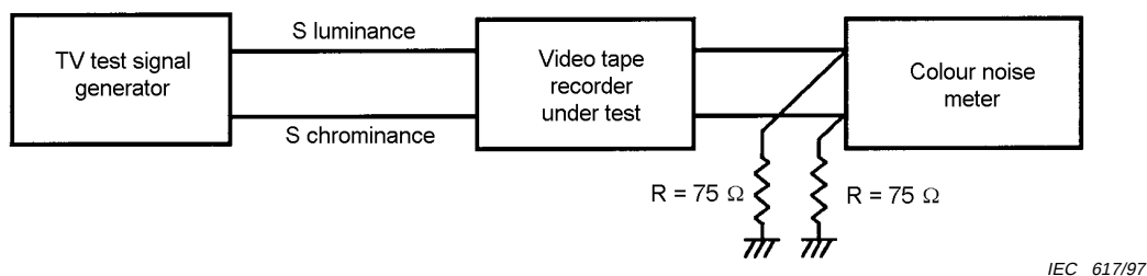
Figure 26 – Block diagram for S video input
