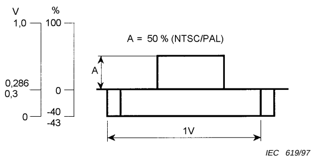
Figure 28 – S luminance window test signal
