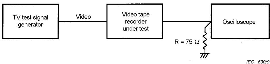
Figure 39 – Block diagram for measurement
