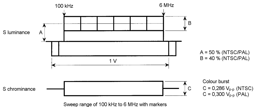
Figure 45 – Video frequency sweep test signal
