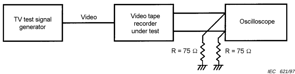
Figure 30 – Block diagram for composite video input
