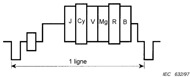
Figure 41 – Signal d'essai
