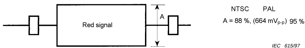
Figure 24 – S chrominance test signal
