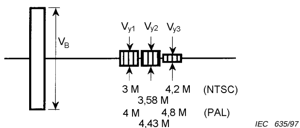
Figure 44 – Measurement of signal levels
