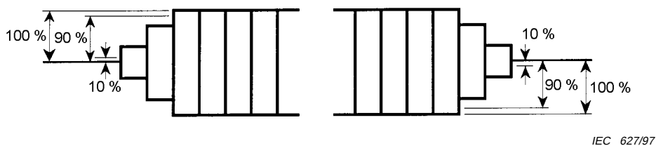
Figure 36 – Measurement of chrominance signal level
