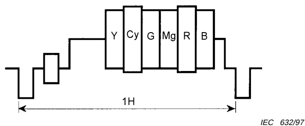
Figure 41 – Test signal
