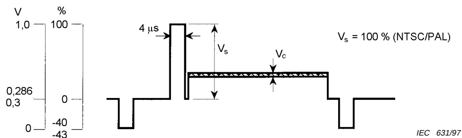
Figure 40 – Measurement of signal levels
