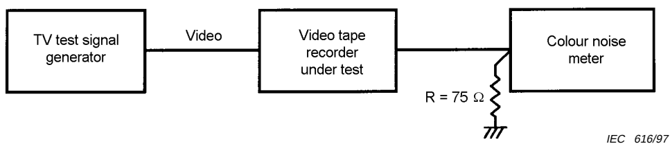
Figure 25 – Block diagram for composite video input
