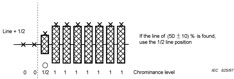
Figure 34 – Waveform of S chrominance signal at line +1/2 (example measurement 2)
