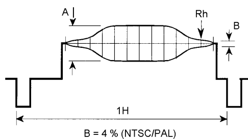
Figure 17 – Waveform for S video input
