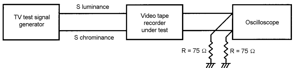
Figure 46 – Block diagram for measurement
