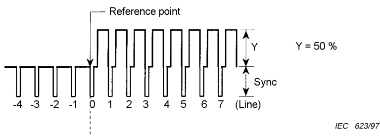
Figure 32 – Waveform of S luminance signal
