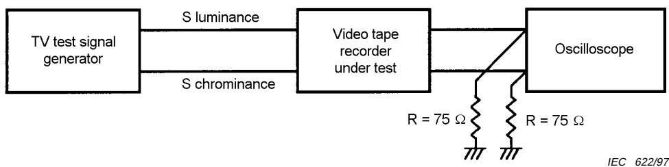
Figure 31 – Block diagram for S video input
