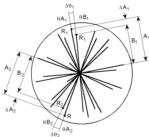
Figure 38 – Example of colour vector measurement
