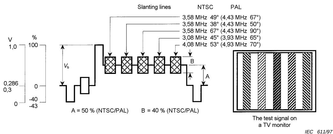
Figure 20 – Multiburst test signal
