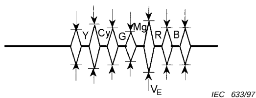
Figure 42 – Measurement of signal levels
