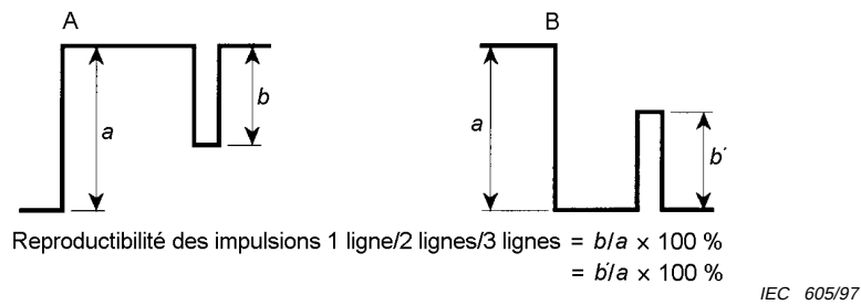
Figure 14a – Impulsion négative
