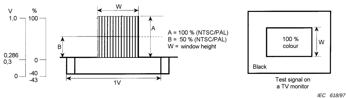
Figure 27 – Composite colour window test signal
