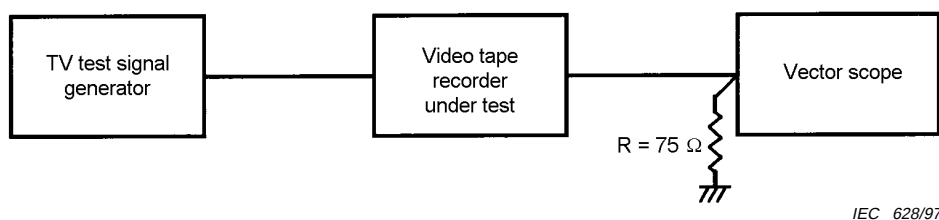
Figure 37 – Block diagram for measurement
