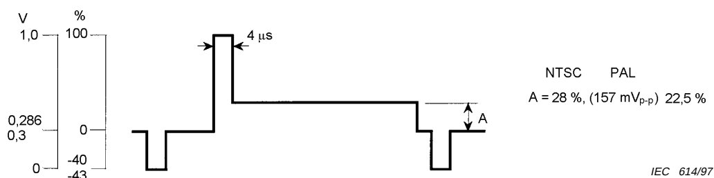
Figure 23 – S luminance test signal
