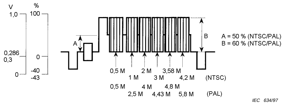
Figure 43 – Signal d'essai multibit
