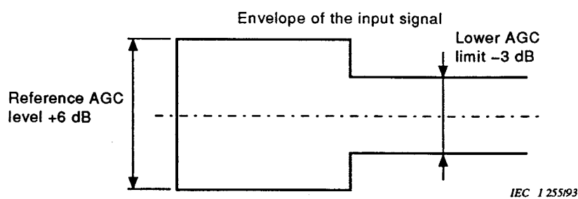
Figure 11a – Attack time and recovery time (2.9.4) test signal
