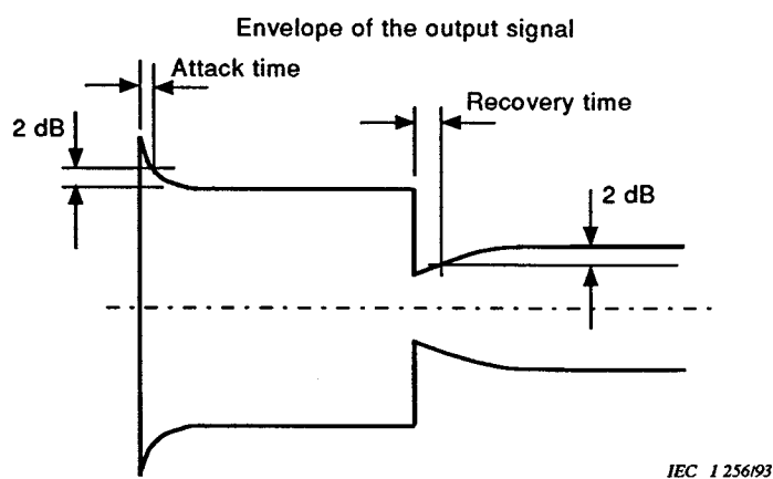
Figure 11b – Attack and recovery time (2.9.4) definition
