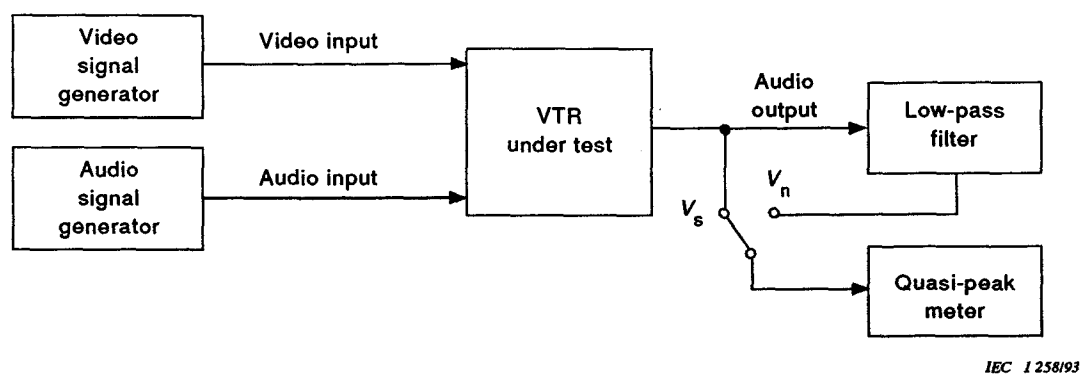
Figure 13 – Circuit arrangement: Switching noise (2.10)
