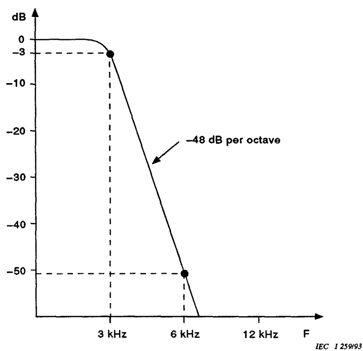
Figure 14 – Low-pass filter characteristics
