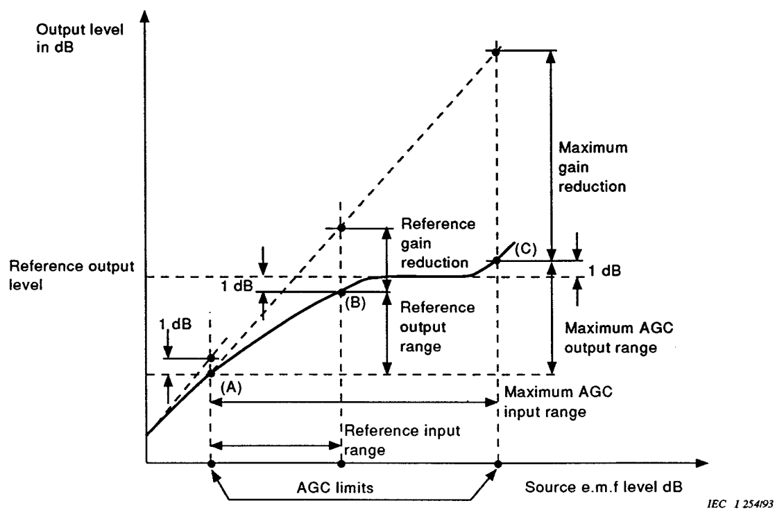
Figure 10 – Gain curve (2.9.3) (out/in response)
