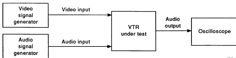
Figure 9 – Circuit arrangement:
