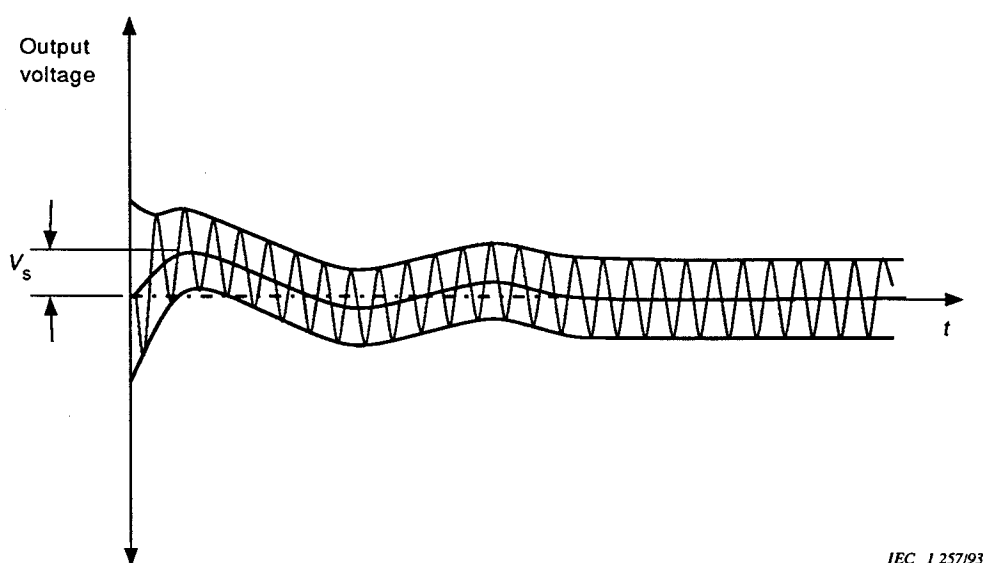
Figure 12 – Output signal (attack transient)
