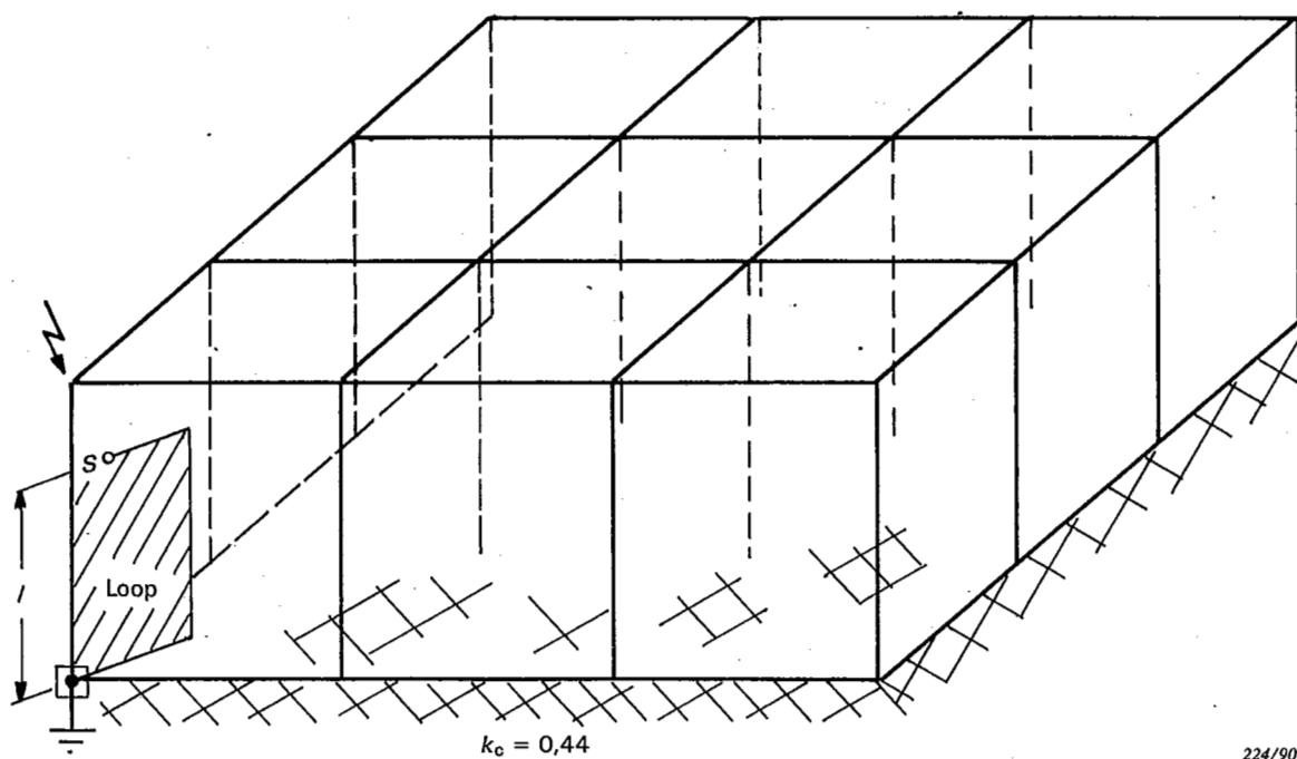
FIG. 5. – Proximity of installations to LPS.
