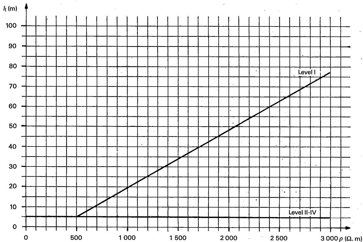
FIG. 2. - Minimum length l_1 of earth electrodes according to the protection levels (see Sub-clauses 2.3.2 and 2.3.3). Levels II to IV are independent of soil resistivity l .
