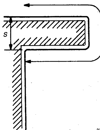
FIG. 1. - Loop in a down-conductor (see Sub-clause 2.2.4).
