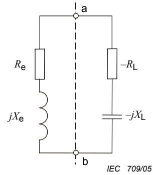
c) – Equivalent circuit
