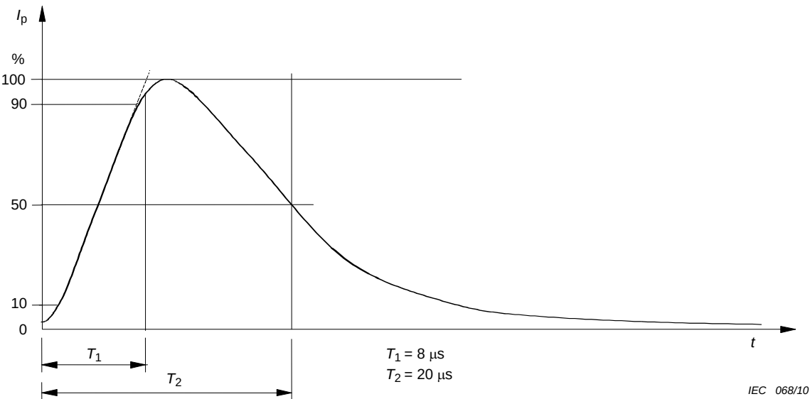
Figure 28 – Onde de courant 8/20 μs
