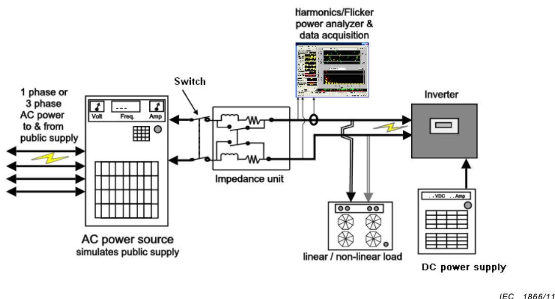
Figure 1 – General test setup for combined emission/immunity tests
