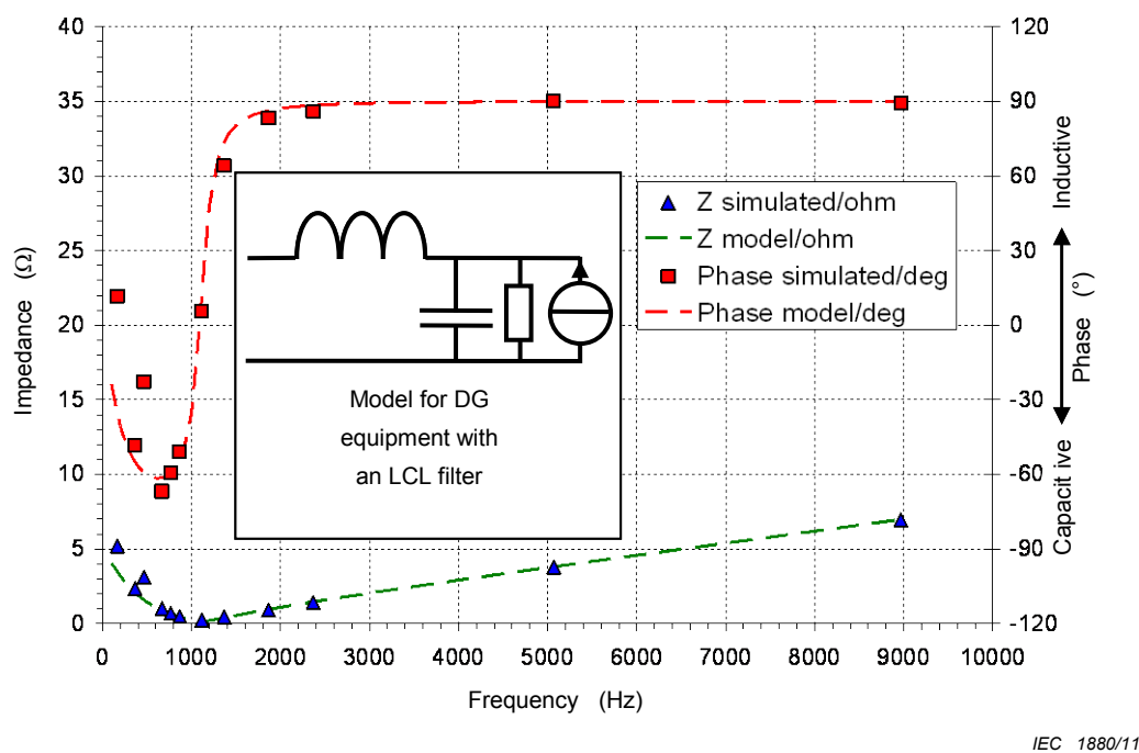
Figure A.4 – Impedance model for DG equipment with LCL filter
