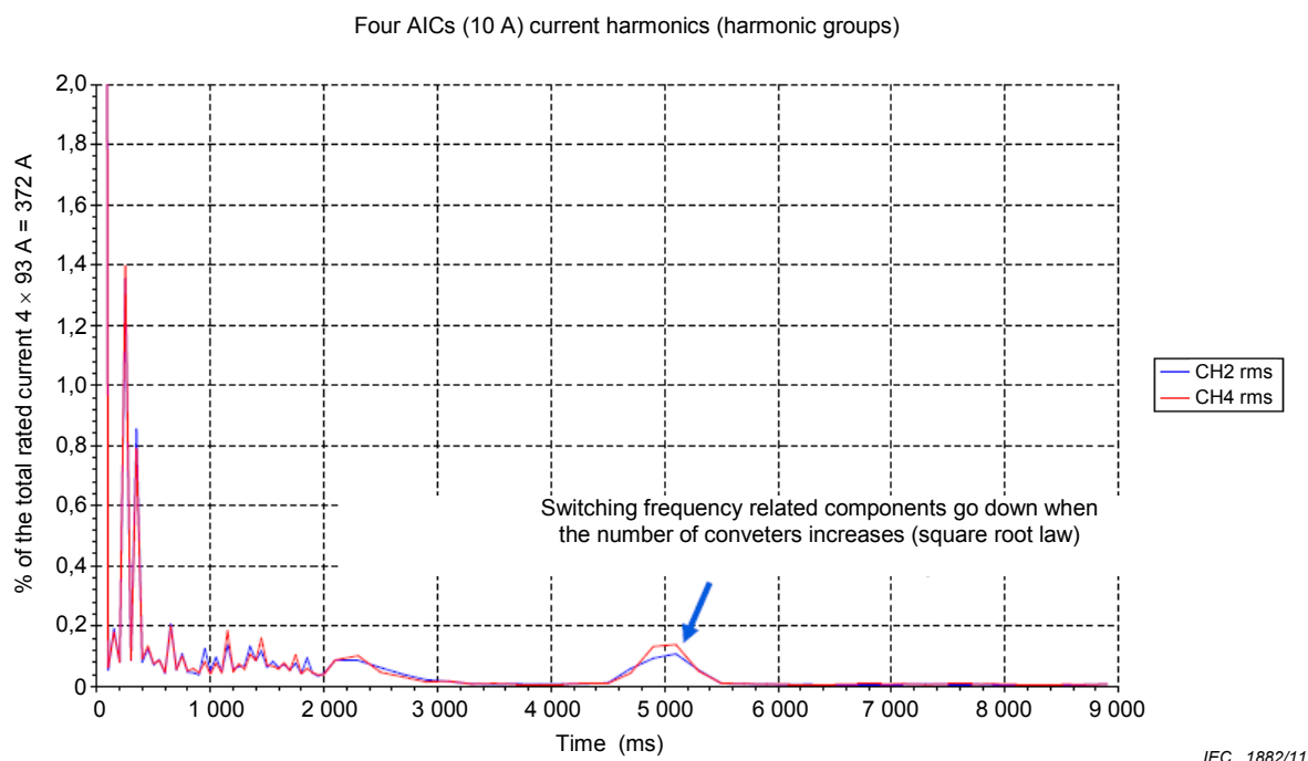
Figure A.6 – Current harmonics: four AICs at 10 A r.m.s. (0,11 I_N )
