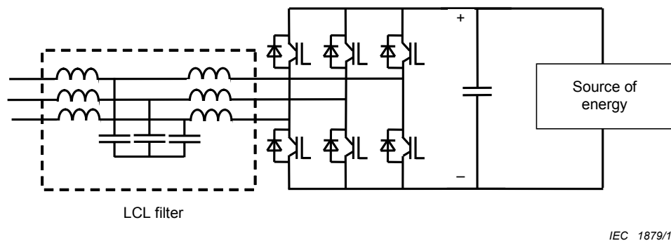
Figure A.3 – DG equipment with LCL filter
