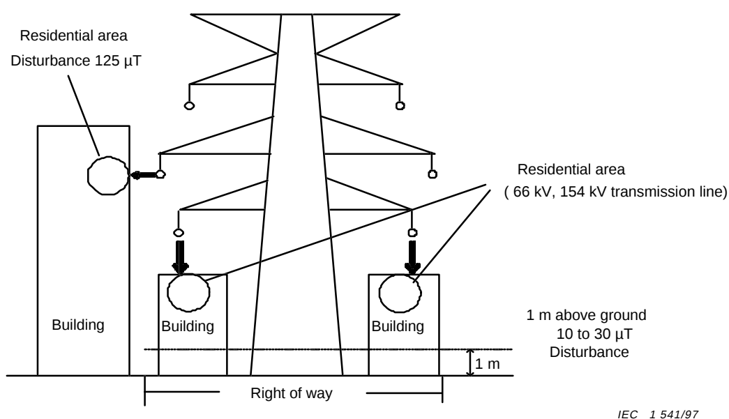
Figure 13 – Magnetic fields produced by HV lines adjacent to residential multi-storey buildings (In Japan, for example, there are buildings under 66 kV and 154 kV transmission lines.)
