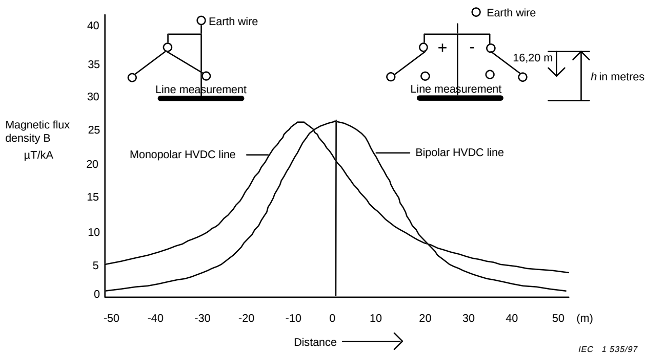
Figure 7 – Curve of the magnetic flux density per kA operating current in the vicinity of a high-voltage d.c. overhead line with an operating voltage of +450 kV or ±450 kV at a point 1 m above the ground
