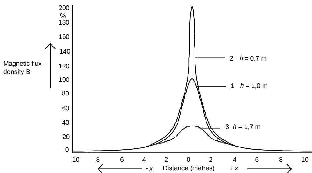
Figure 9 – Comparison of magnetic flux density characteristics of single core cables laid at depths of 0,7 m (curve 2), 1,7 m (curve 3), with a cable laid at a depth of 1 m (curve 1) Magnetic flux densities are expressed as a percentage of the maximum value associated with curve 1. The cable configuration is as figure 9 with dimensions corresponding to table 4, line 5.
