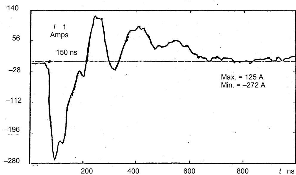
Figure 19 – Measured HEMP-induced current on power line directly above left end of locomotive
