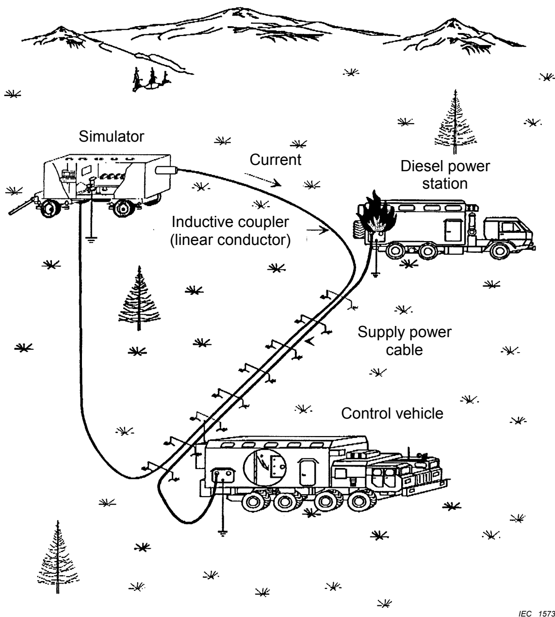
Figure 26 – Simulation of HEMP effects on a mobile diesel power station under operating voltage
