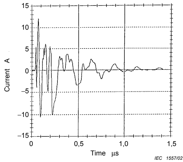
Figure 12 – Time response for a typical power cable coupled current measured at WRF
