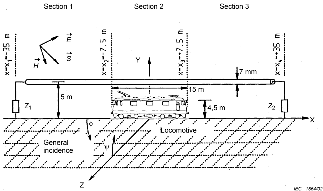
Figure 18 – Geometry for HEMP simulation test of locomotive with single power line
