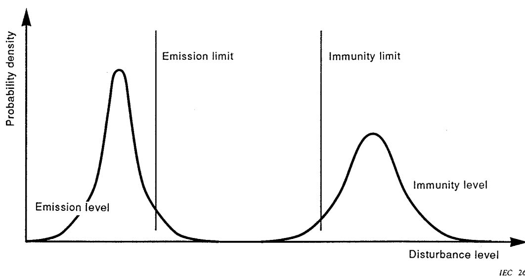
Figure 5 – Example of the probability densities for an emission level and an immunity level, at one single value of the independent variable
