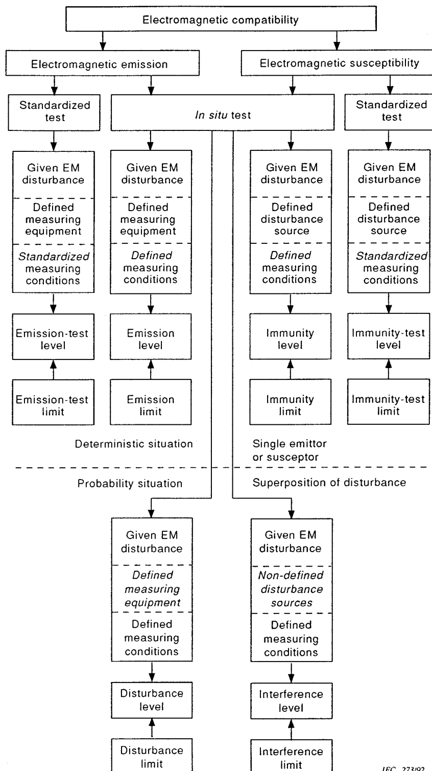
Figure A.3 – Overview of various EMC terms and measuring conditions
