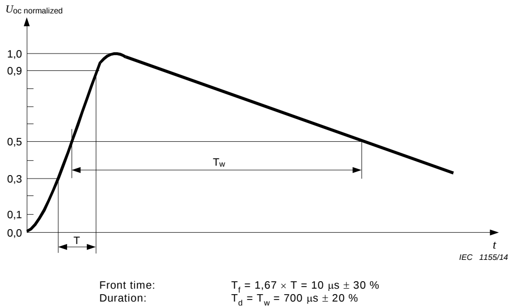
Figure A.2 – Waveform of open-circuit voltage (10/700 μs)
