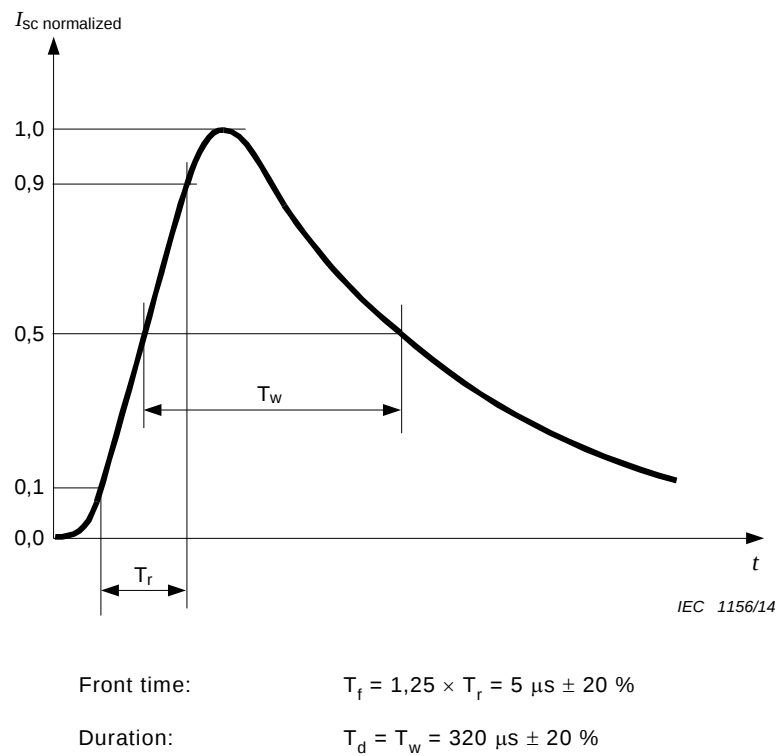
Figure A.3 – Waveform of the 5/320 μs short-circuit current waveform
