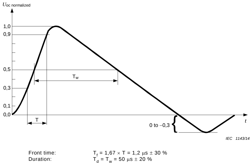
Figure 2 – Waveform of open-circuit voltage (1,2/50 μs) at the output of the generator with no CDN connected
