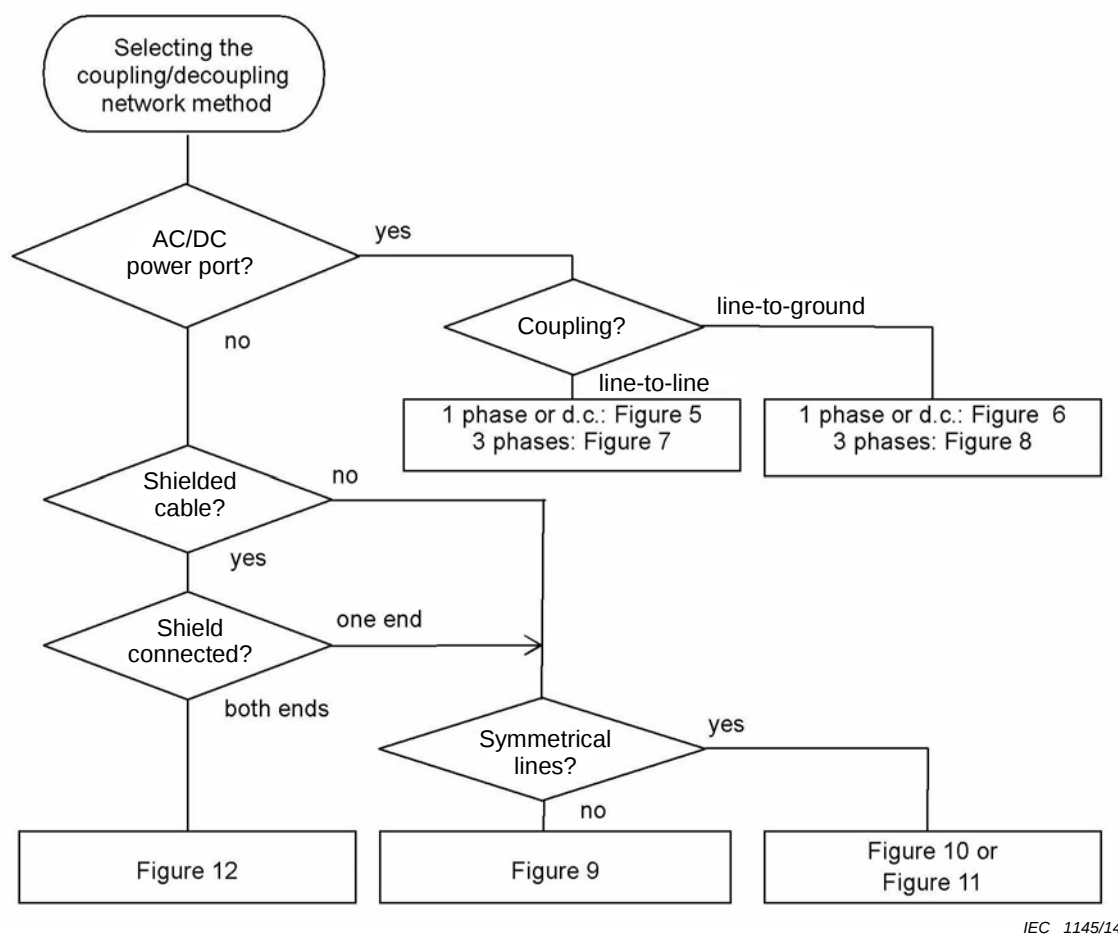
Figure 4 – Selection of coupling/decoupling method
