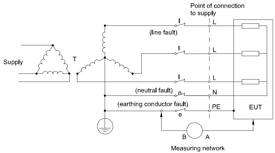
Figure 11 – Three-phase equipment on star TN or TT system
