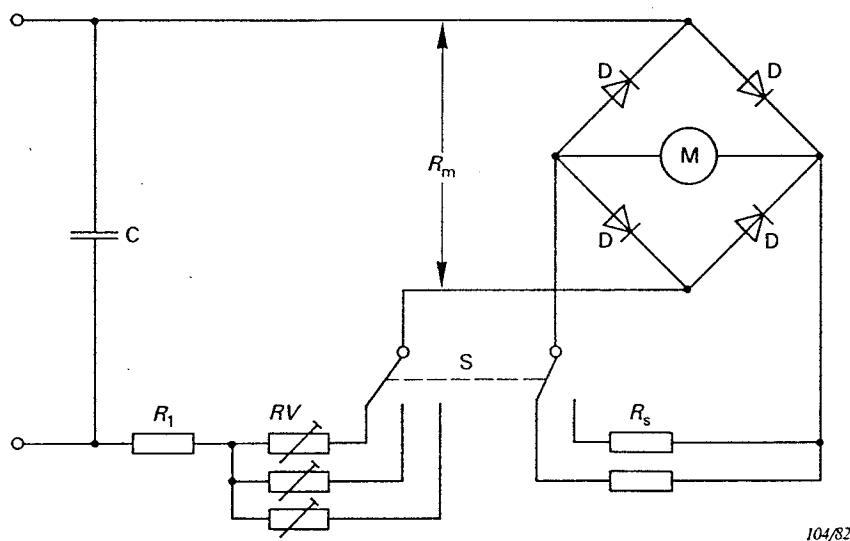
Figure C - Circuit for measuring leakage currents
