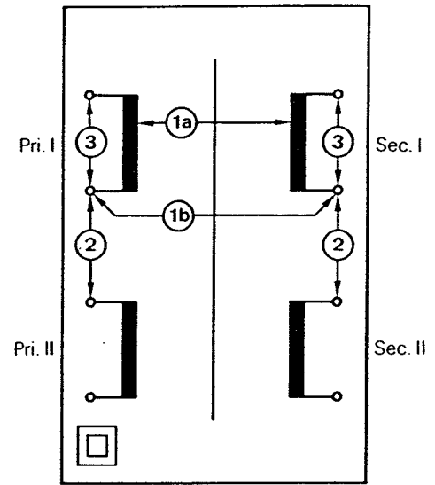
ii) Noyau isolé de la masse Core insulated from the body
