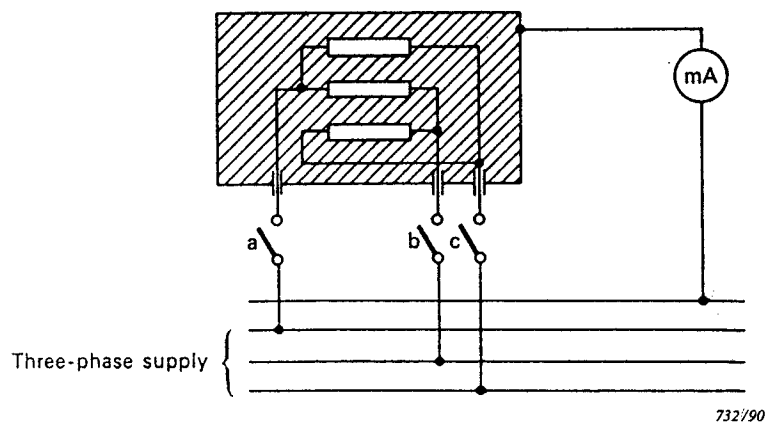
Figure B - Diagram for leakage current measurement at operating temperature for three-phase connection of appliances other than those of Class II.
