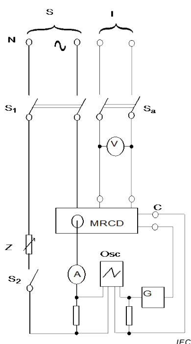
Figure M.3b) – MRCD with integral sensing means
