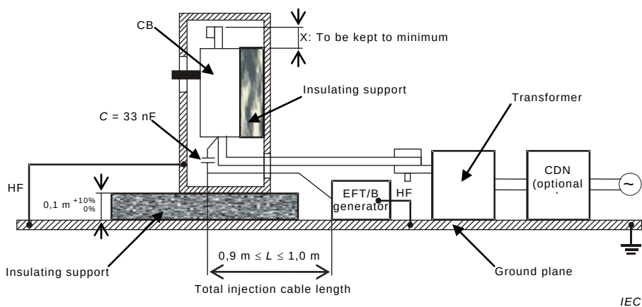
Figure F.17 – Test set-up for the verification of immunity to radiated RF electromagnetic fields
