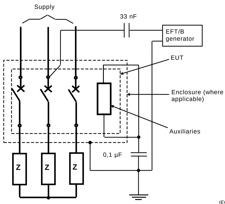
Figure F.7 – Circuit for electrical fast transients/bursts (EFT/B) immunity test in accordance with F.4.4 – Three phase poles in series
