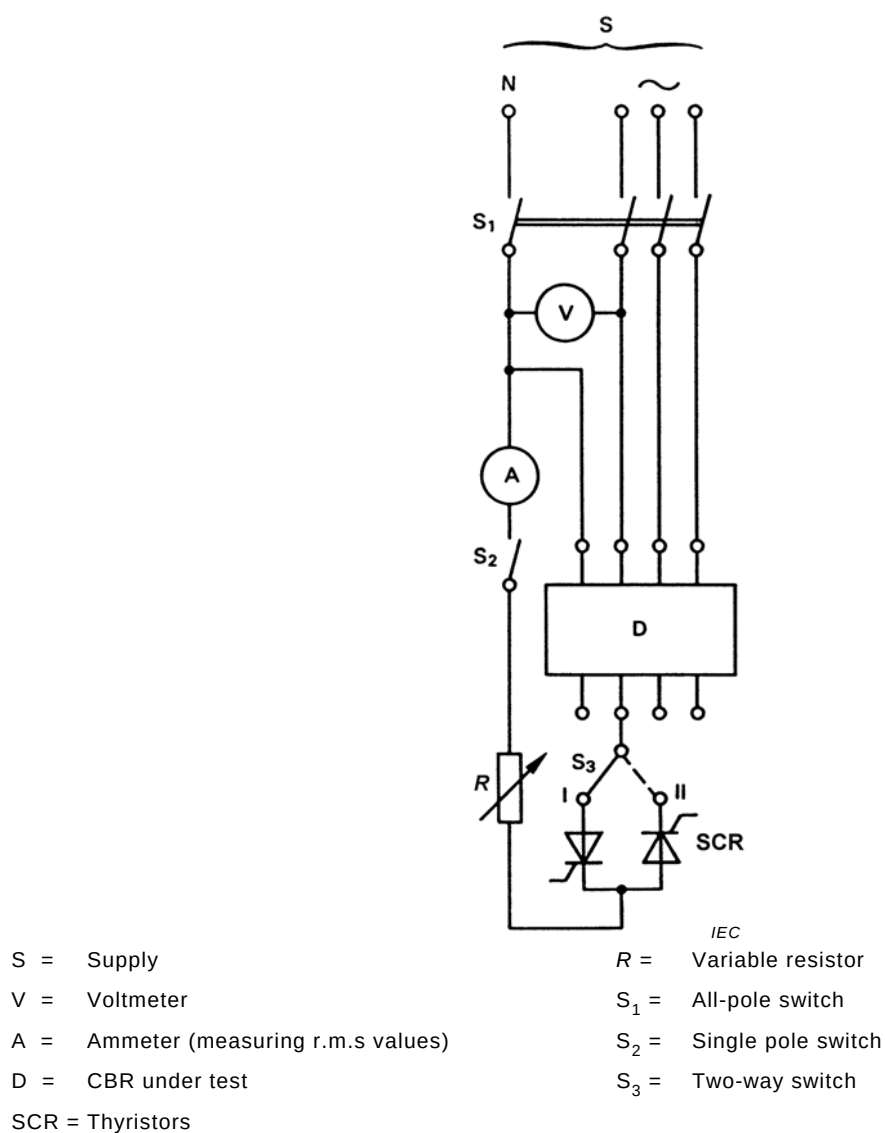
Figure B.8 – Test circuit for the verification of the correct operation of CBRs, in the case of residual pulsating direct currents (see B.8.7.2.1, B.8.7.2.2 and B.8.7.2.3)
