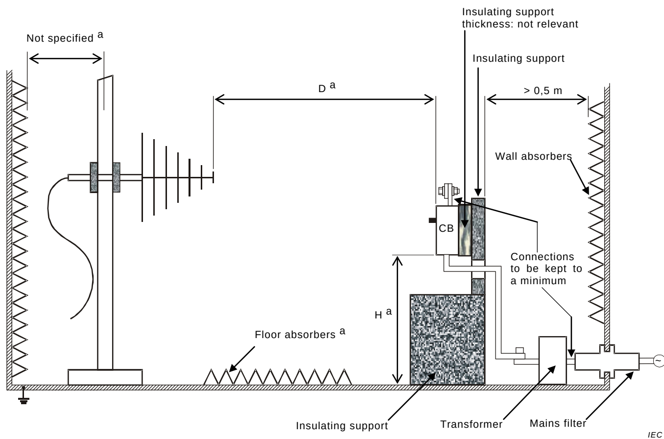
Figure F.16 – General test set-up for immunity tests
