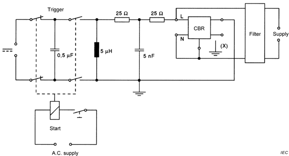
Figure B.4 – Current ring wave 0,5 μs/100 kHz
