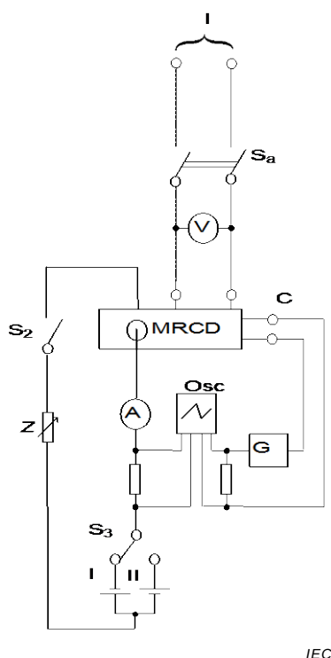
Figure M.12b) – MRCD with integral sensing means
