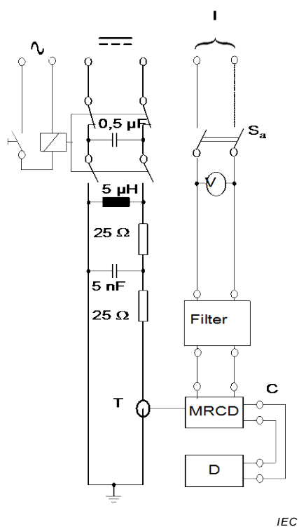
Figure M.5a) – MRCD with separate sensing means
