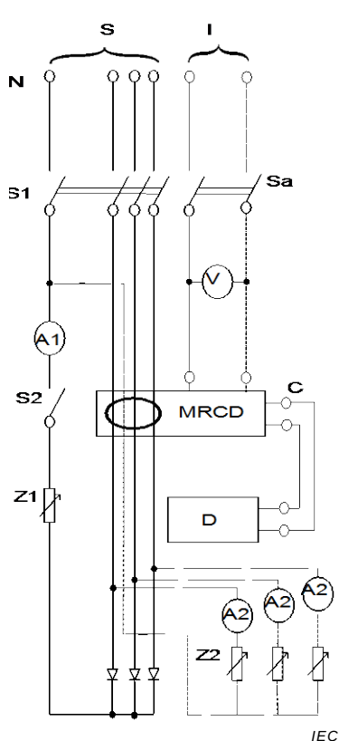
Figure M.14b) – MRCD with integral sensing means
