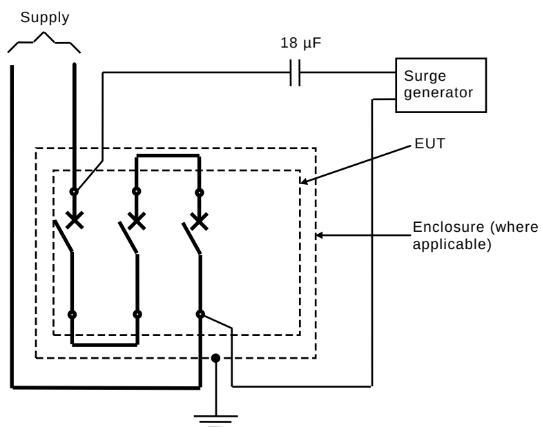
Figure F.13 – Test circuit for the verification of the influence of current surges in the main circuit in accordance with F.4.5 – Three phase poles in series
