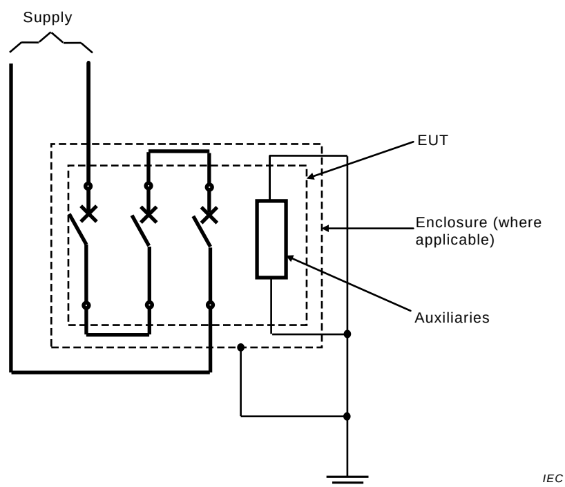
Figure F.3 – Test circuit for immunity and emission tests in accordance with F.4.1.3, F.4.2, F.4.3, F.4.6, F.4.7.1, F.5.4 and F.6.3 – Three phase poles in series
