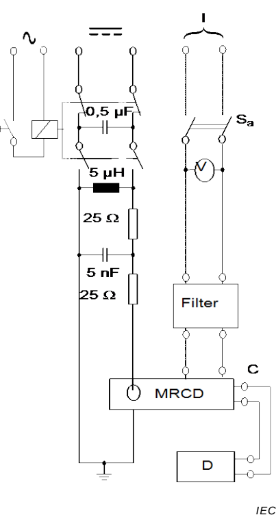
Figure M.5b) – MRCD with integral sensing means
