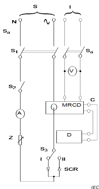
Figure M.7b) – MRCD with integral sensing means
