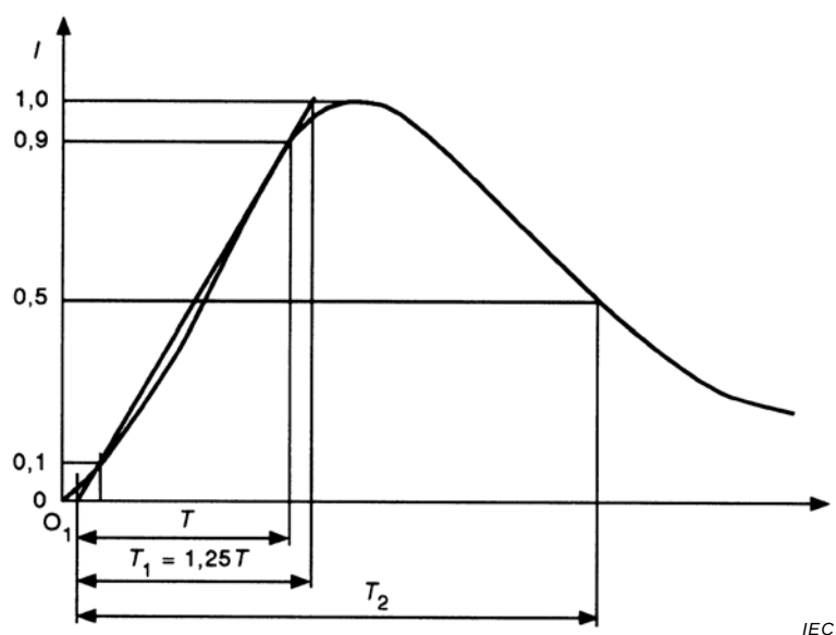
Figure B.6 – Onde de courant de choc 8/20 \mu s
