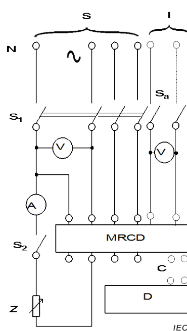
Figure M.1c) – Terminal type MRCD
