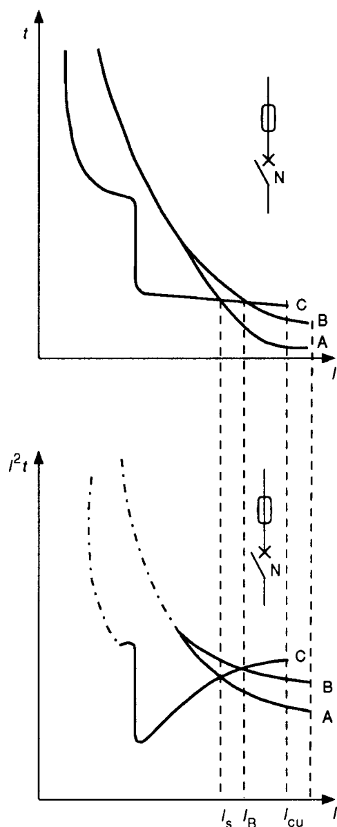
Figure A.1 – Over-current co-ordination between a circuit-breaker and a fuse or back-up protection by a fuse: operating characteristics
