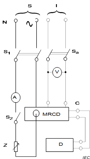
Figure M.1b) – MRCD with integral sensing means
