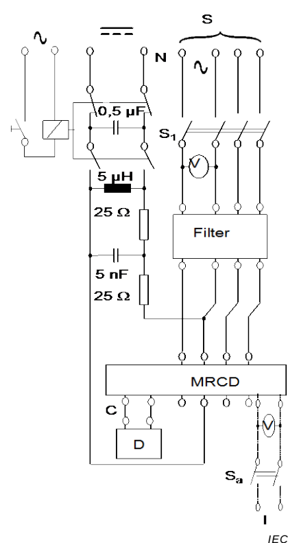
Figure M.5c) – Terminal type MRCD
