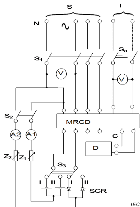
Figure M.10c) – Terminal type MRCD
