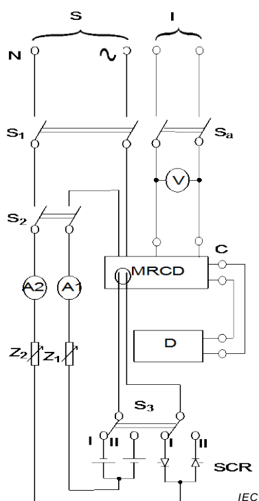
Figure M.10b) – MRCD with integral sensing means
