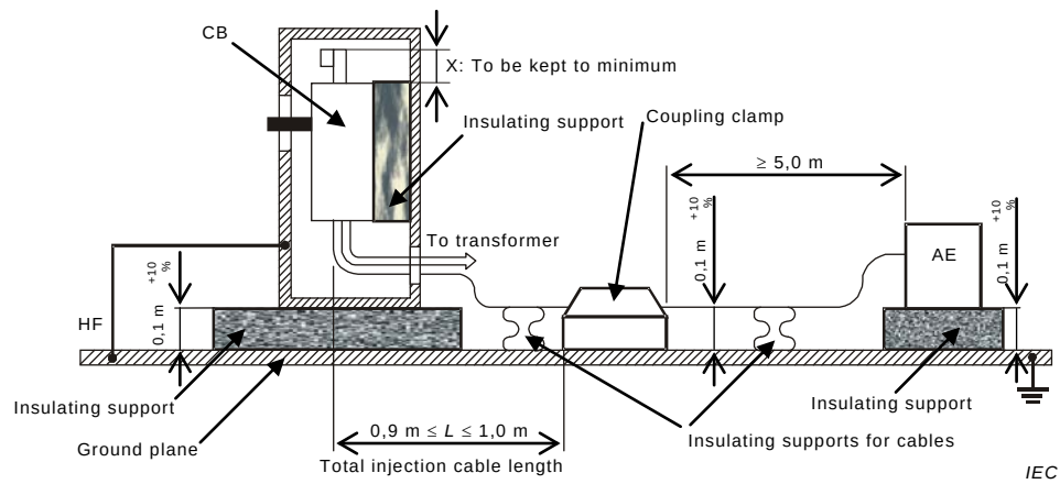
Figure F.18 – Test set-up for the verification of immunity to electrical fast transients/bursts (EFT/B) on power lines
