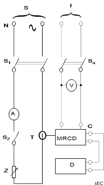
Figure M.1a) – MRCD with separate sensing means
