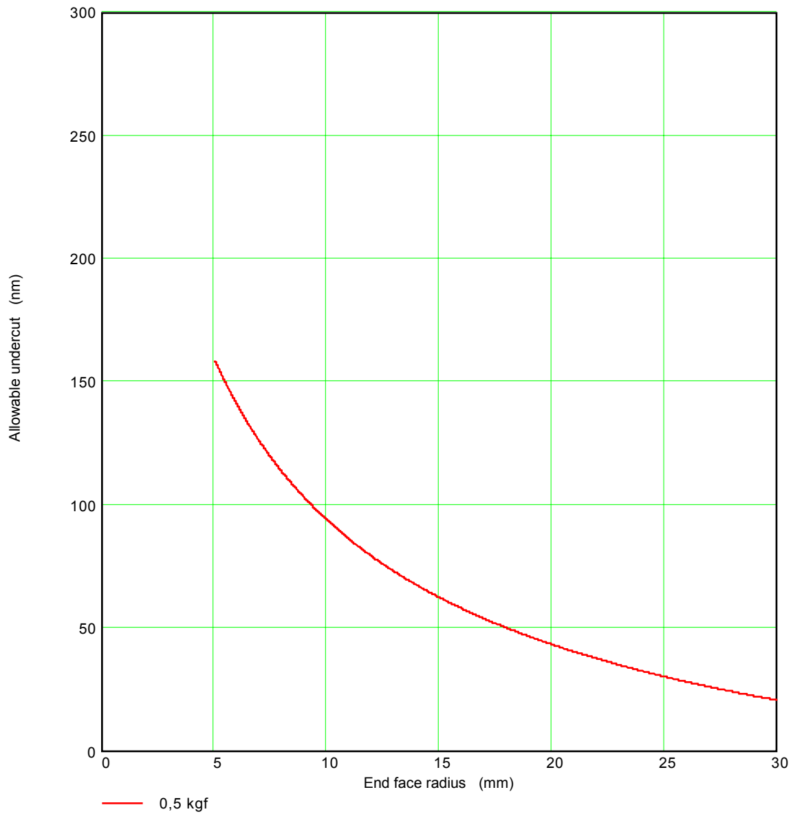
Allowable undercut for 0,5 kgf, and 62,5 µm Minimum contact diameter
