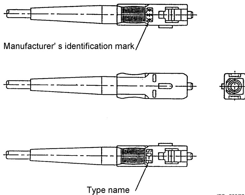
Figure 5 – Example of component marking
