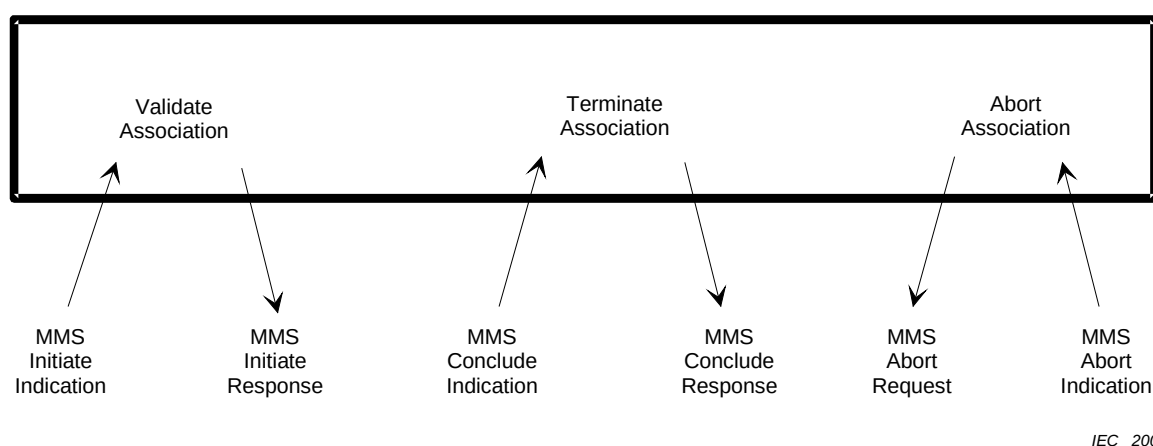
Figure 8 – TASE.2 Server association control elements
