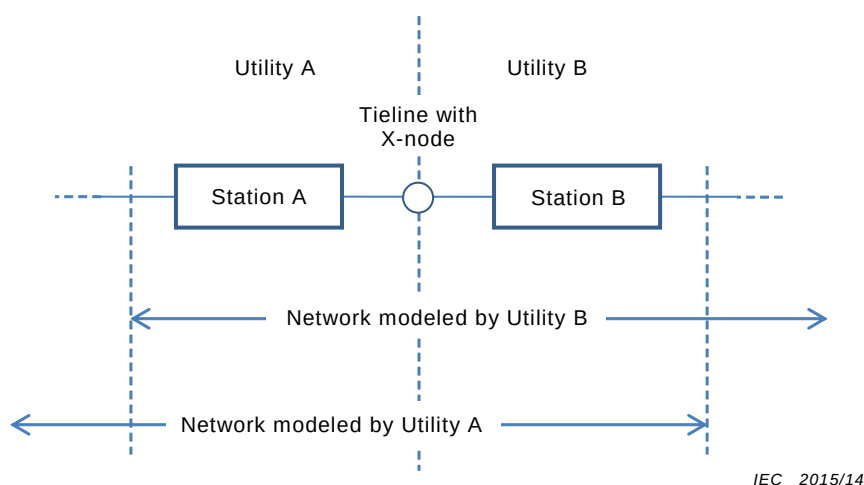
Figure 17 – Measurements and network models
