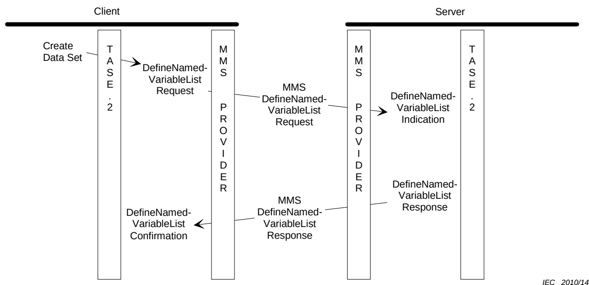
Figure 12 – Sequence of Create Data Set operation
