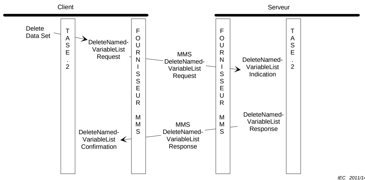
Figure 13 – Séquence de Delete Data Set
