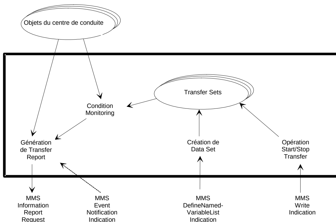
Figure 14 – Services Transfer Set (ensemble de transfert)
