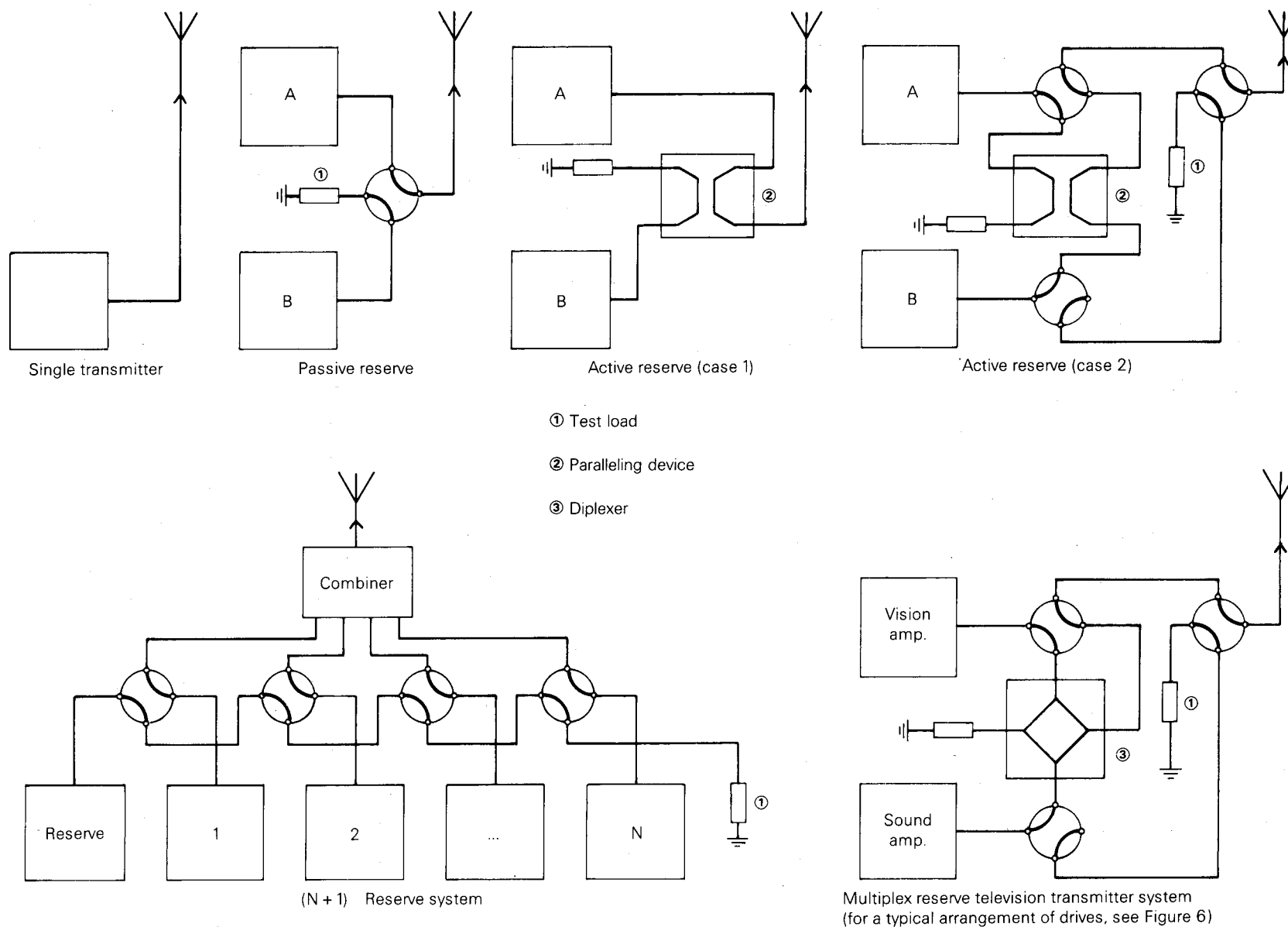
FIG. 3. — Simplified diagrams of commonly used transmitter systems.
