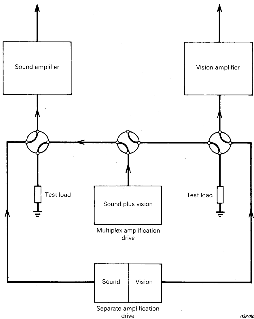
FIG. 6. — Typical arrangement of drives in a multiplex reserve television transmitter system.
