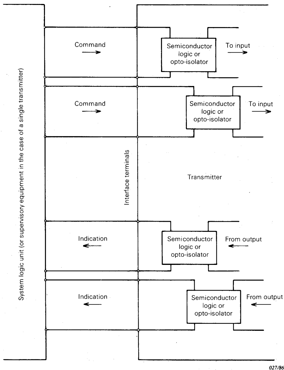
FIG. 5. — Principle of semiconductor logic and opto-isolator interface techniques.
