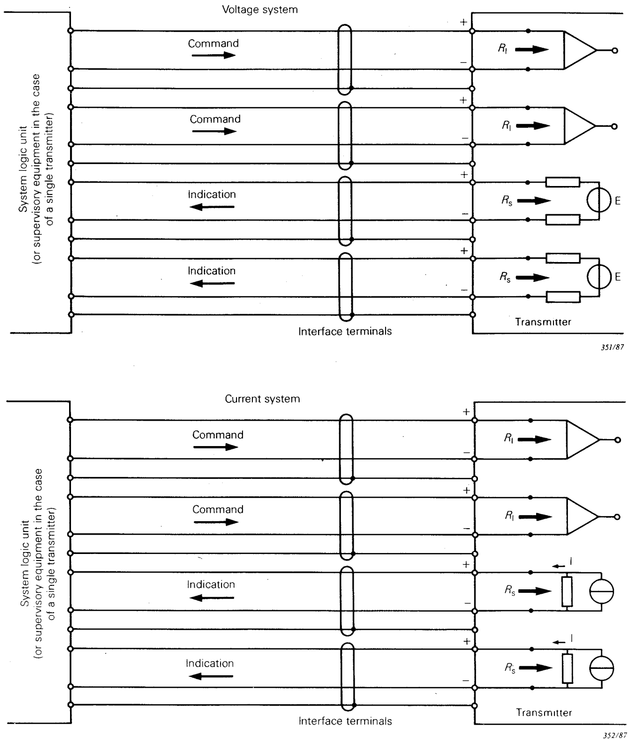
FIG. 7. — Example of analogue interface technique.
