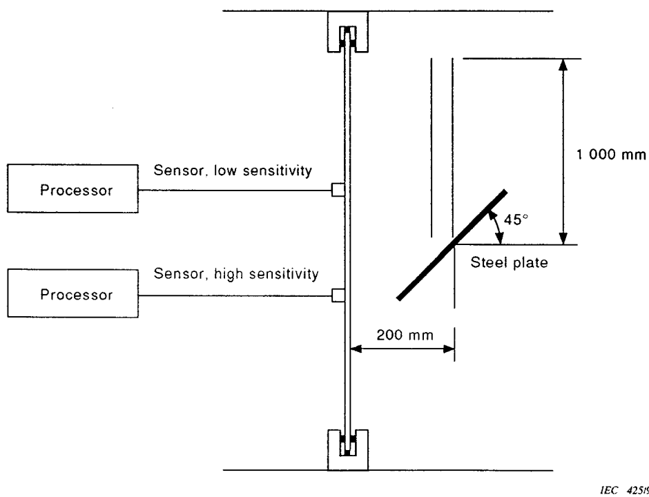
Figure 4 – Test arrangement for gravel impact
