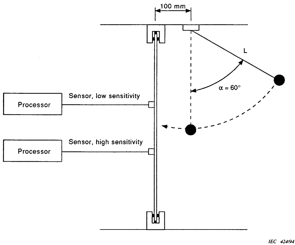
Figure 3 – Test arrangement for ball impact
