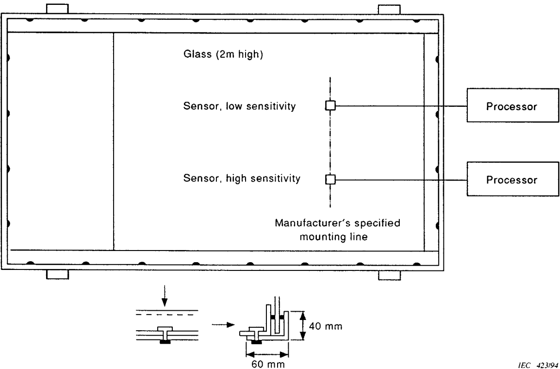
Figure 2 – Test arrangement for group 1 tests
