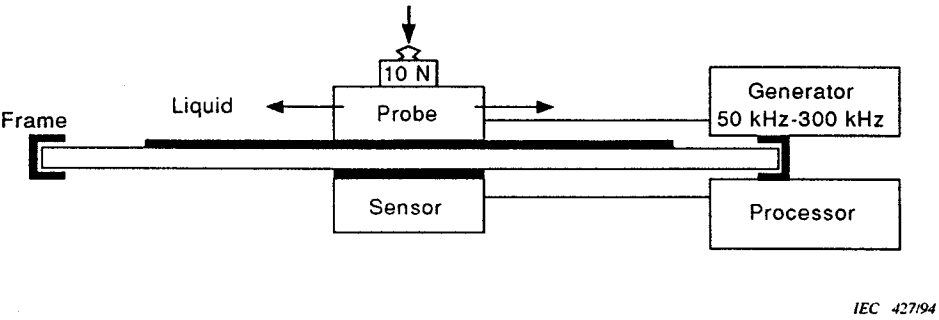
Figure 6 – Test arrangement for basic tests
