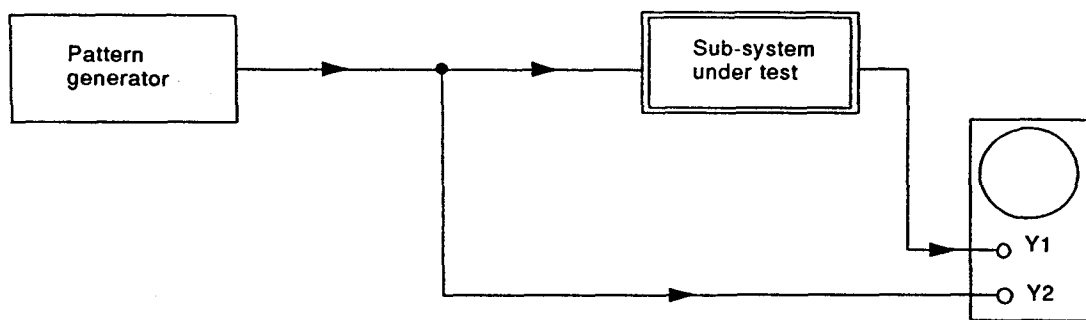
Figure 7a – Test arrangement for measuring the absolute delay time
