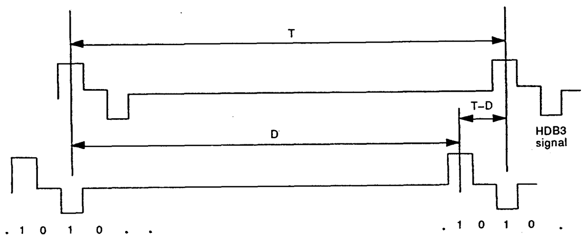
Figure 7b – Example of the pattern to be used in the evaluation of the absolute delay time
