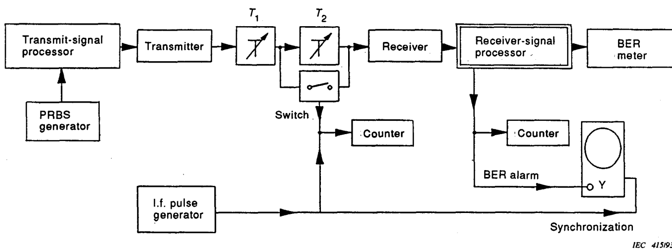
Figure 9 – Test arrangement for measuring the BER alarm characteristics
