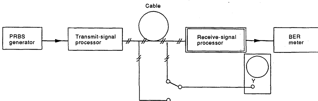
Figure 6 – Test arrangement for measuring the acceptability of the signal at the input of the receive-signal processor
