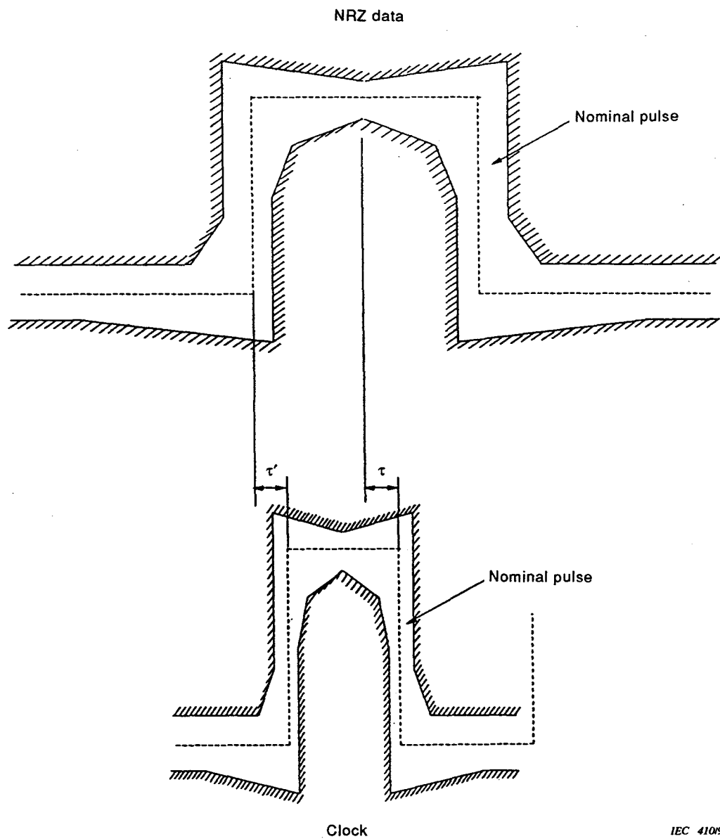
Figure 5 – Example of pulse masks in the case of NRZ data and CK (clock) signals
