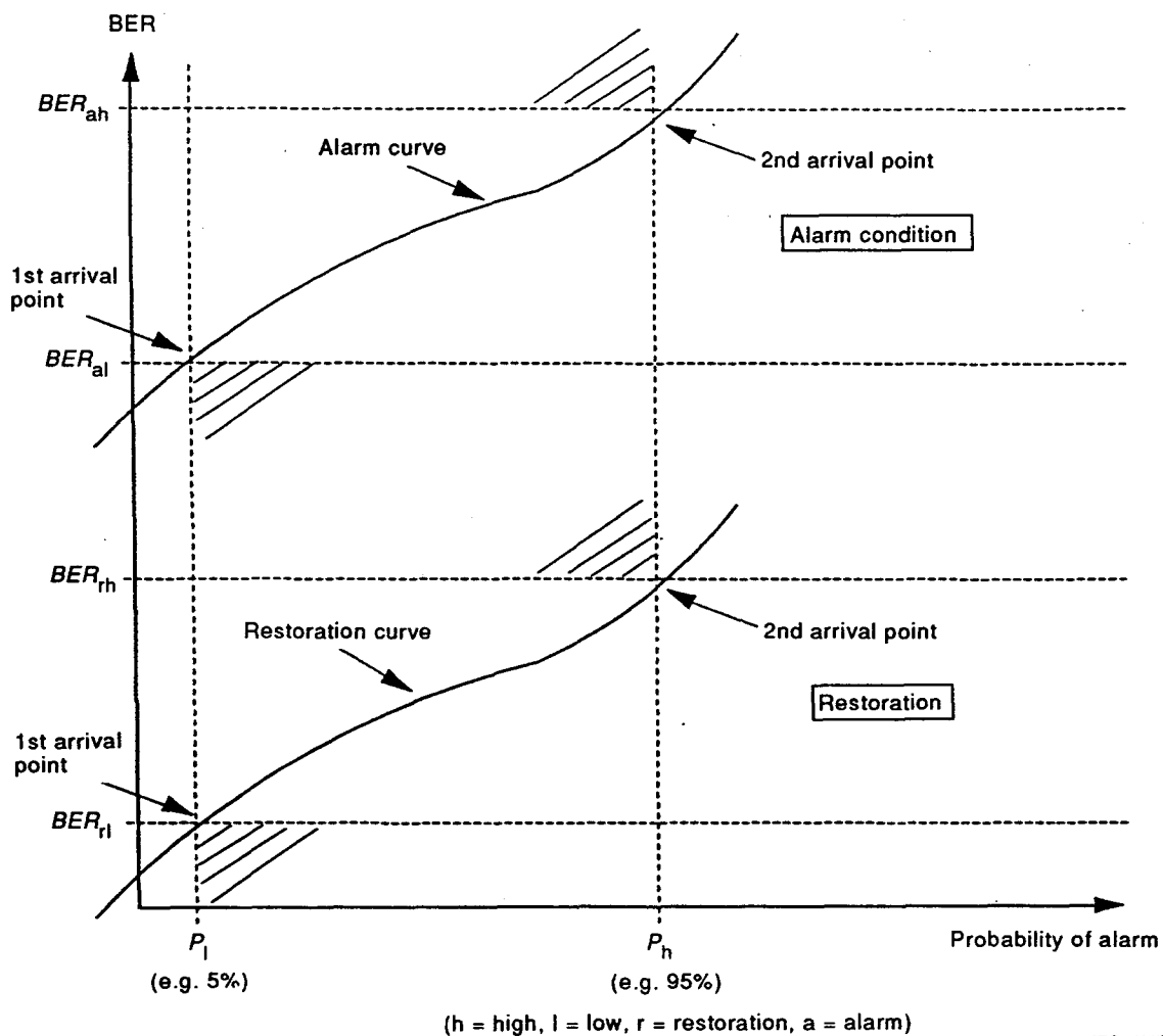
Figure 8 – Examples of curves for the evaluation of the BER alarm characteristics
