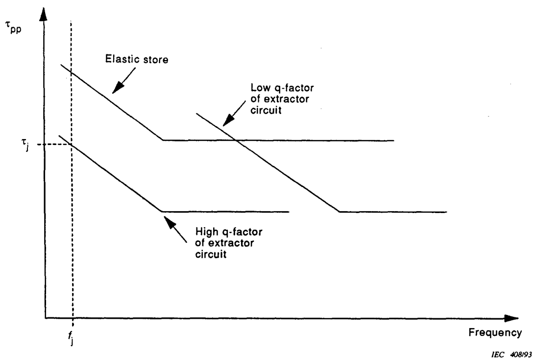
Figure 3 – Comparison of the tolerable input jitter characteristics between the clock extractor and the input of the sub-system under test
