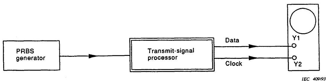
Figure 4 – Test arrangement for measuring the level and shape of the output signal of the transmit-signal processor
