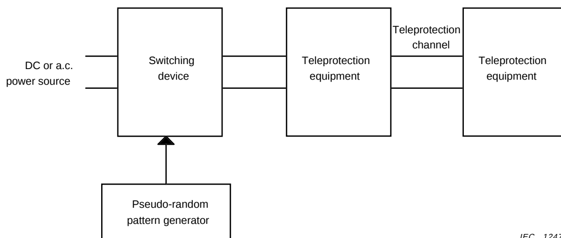
Figure 7 – Test circuit for testing power supply interruptions
