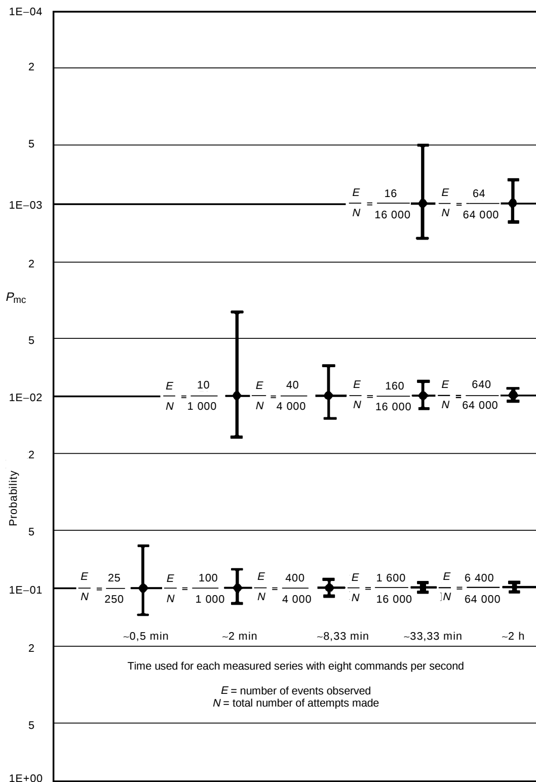
Figure A.1 – Graph showing the uncertainty of probability for a confidence level of 95 % for various values of E and N
