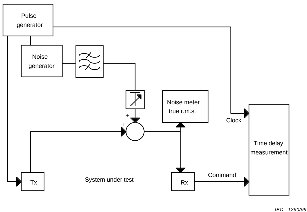
Figure 20 – Test set-up for recovery time measurement for analogue teleprotection
