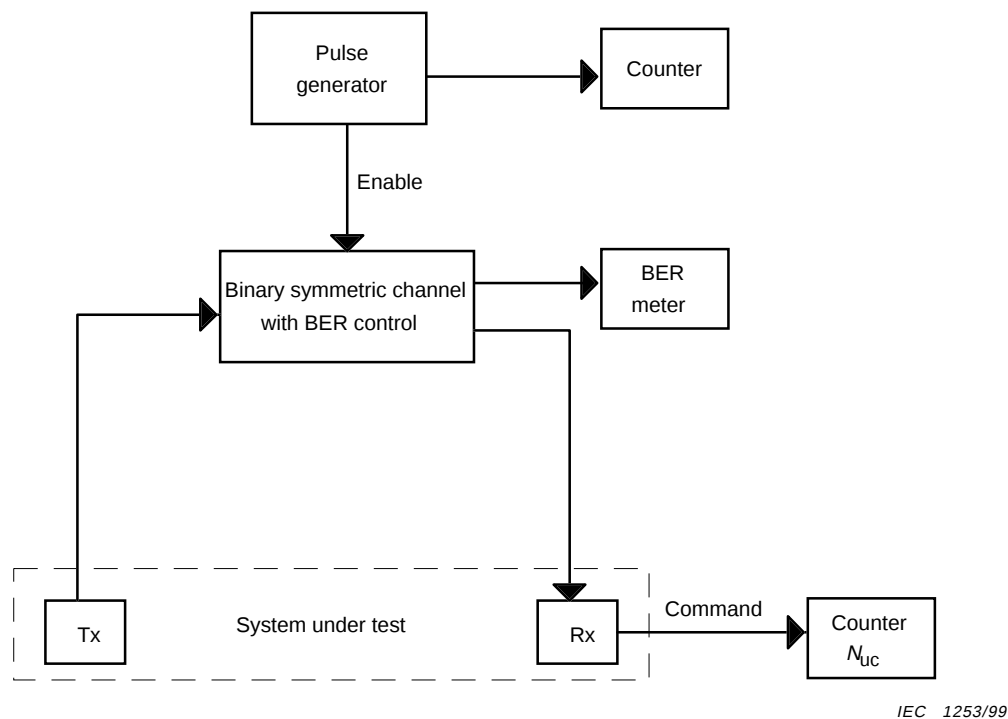
Figure 13 – Test set-up for security measurement (digital teleprotection)
