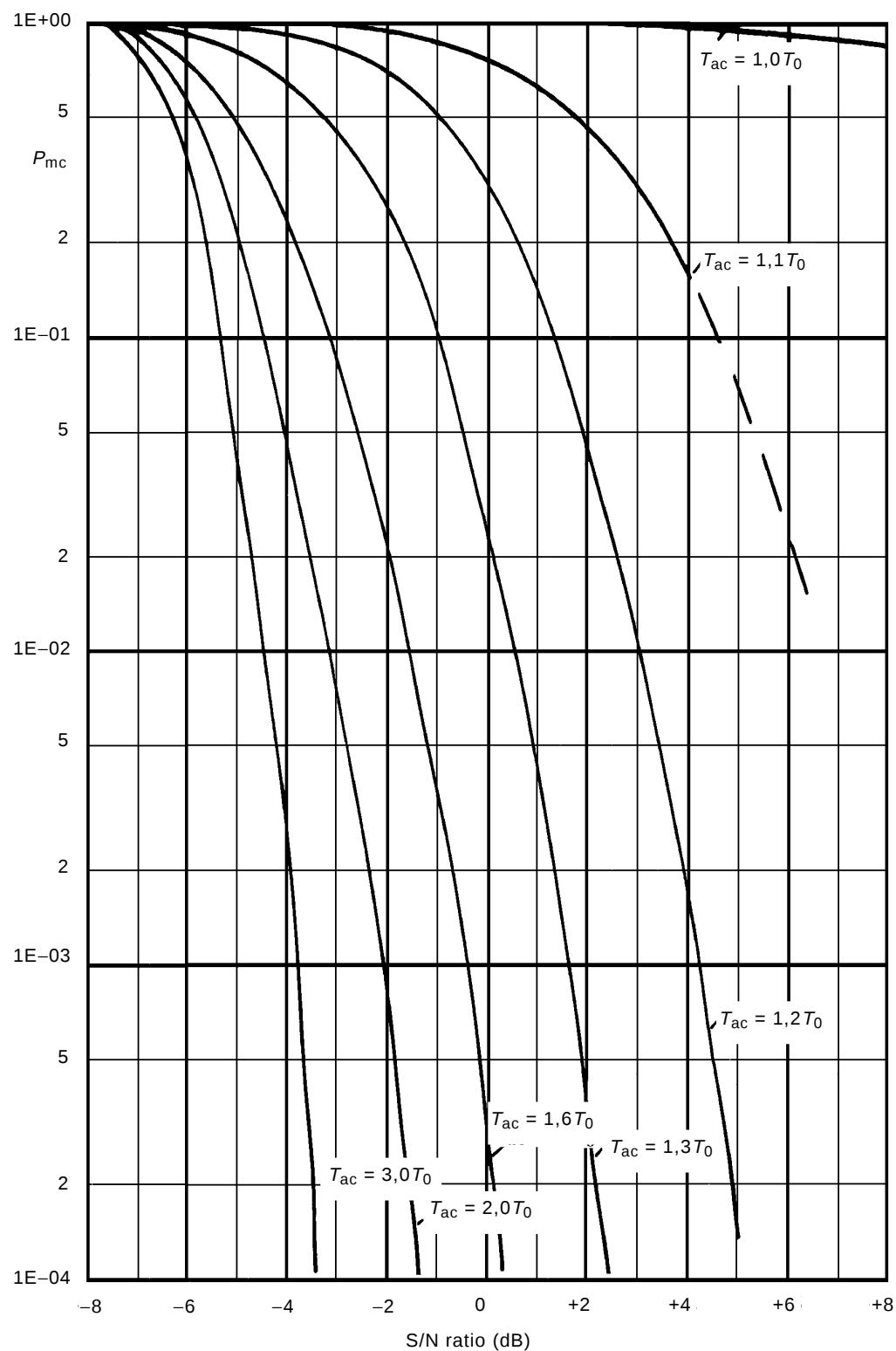
Figure 9 – Examples of the probability of missing command versus signal-to-noise ratio
