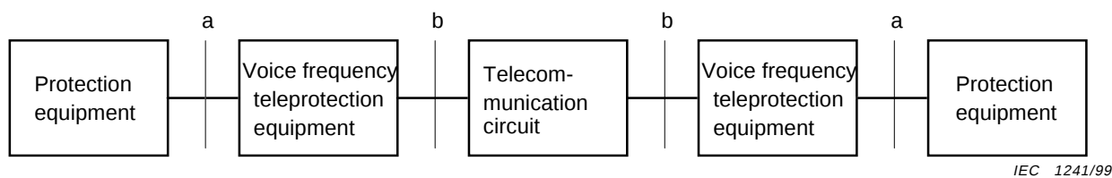
Figure 1 – Voice frequency configuration
