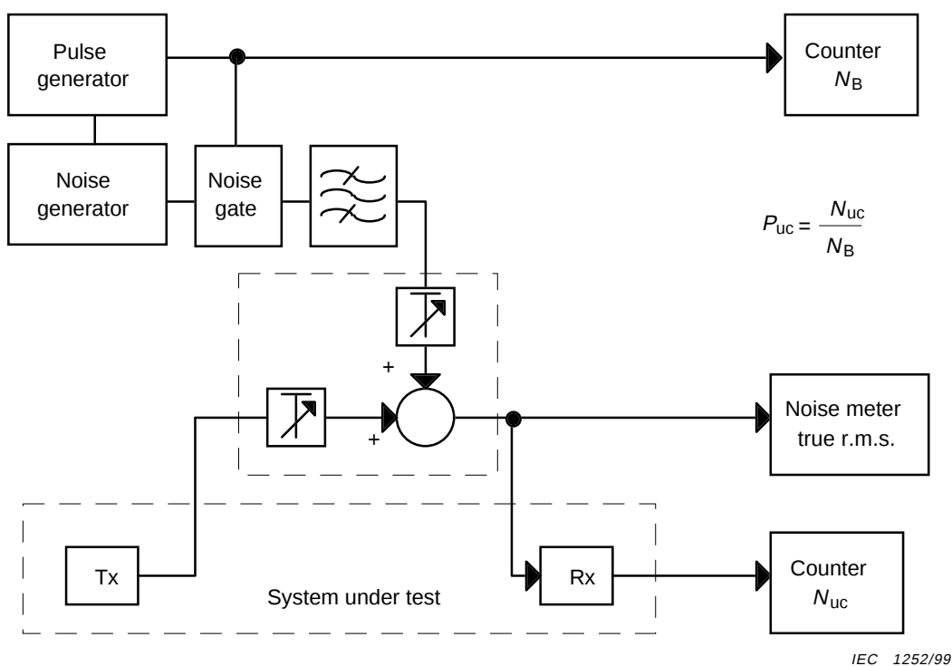
Figure 12 – Test set-up for security measurement (analogue teleprotection)
