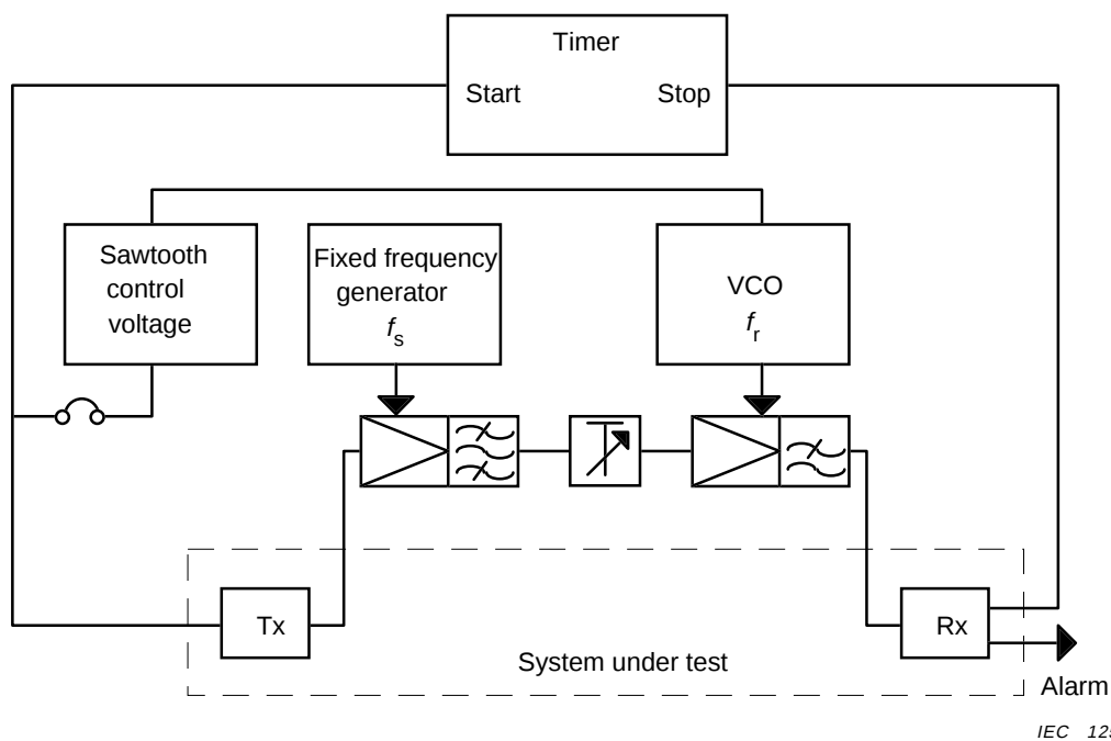
Figure 17 – Test set-up for measuring interference by frequency deviation
