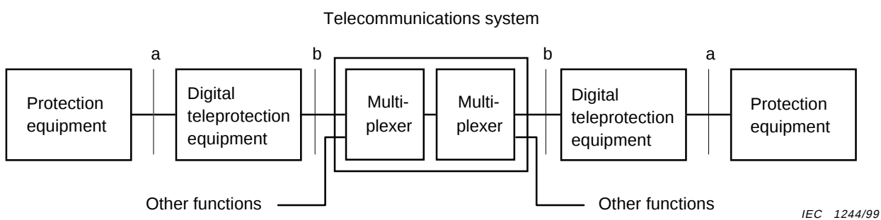
Figure 4 – Digital teleprotection connected via a multiplexed communication system
