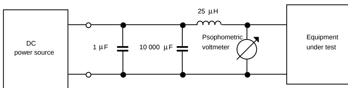
Figure 8 – Test circuit for LF disturbance emission measurement
