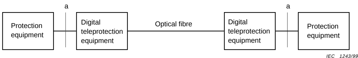
Figure 3 – Directly connected digital teleprotection (example)
