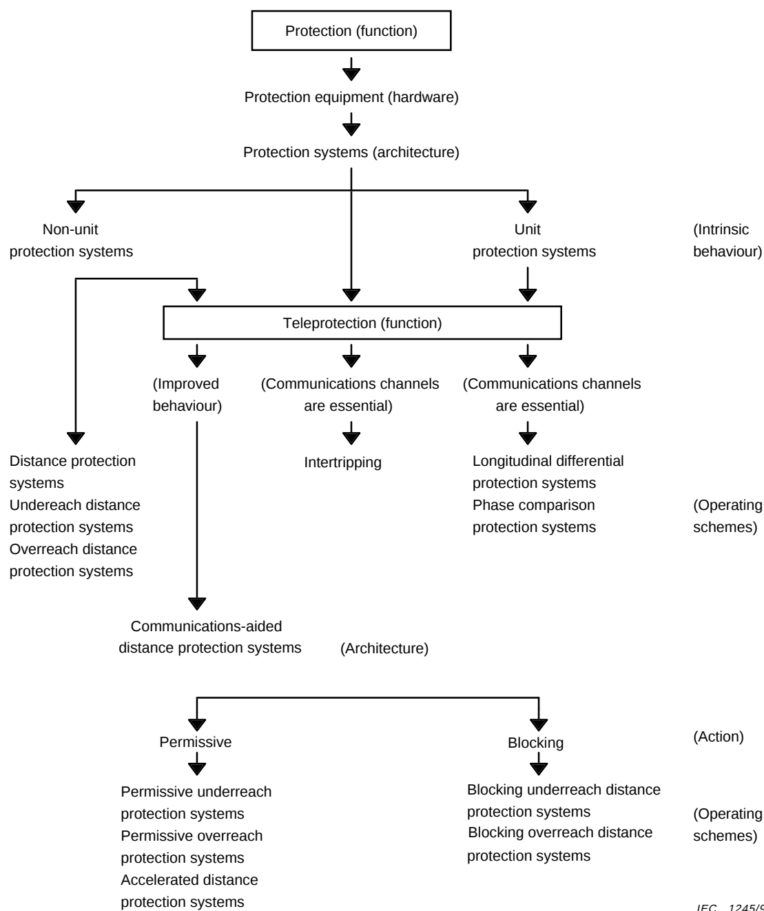
Figure 5 – Fundamental terms on protection and teleprotection
