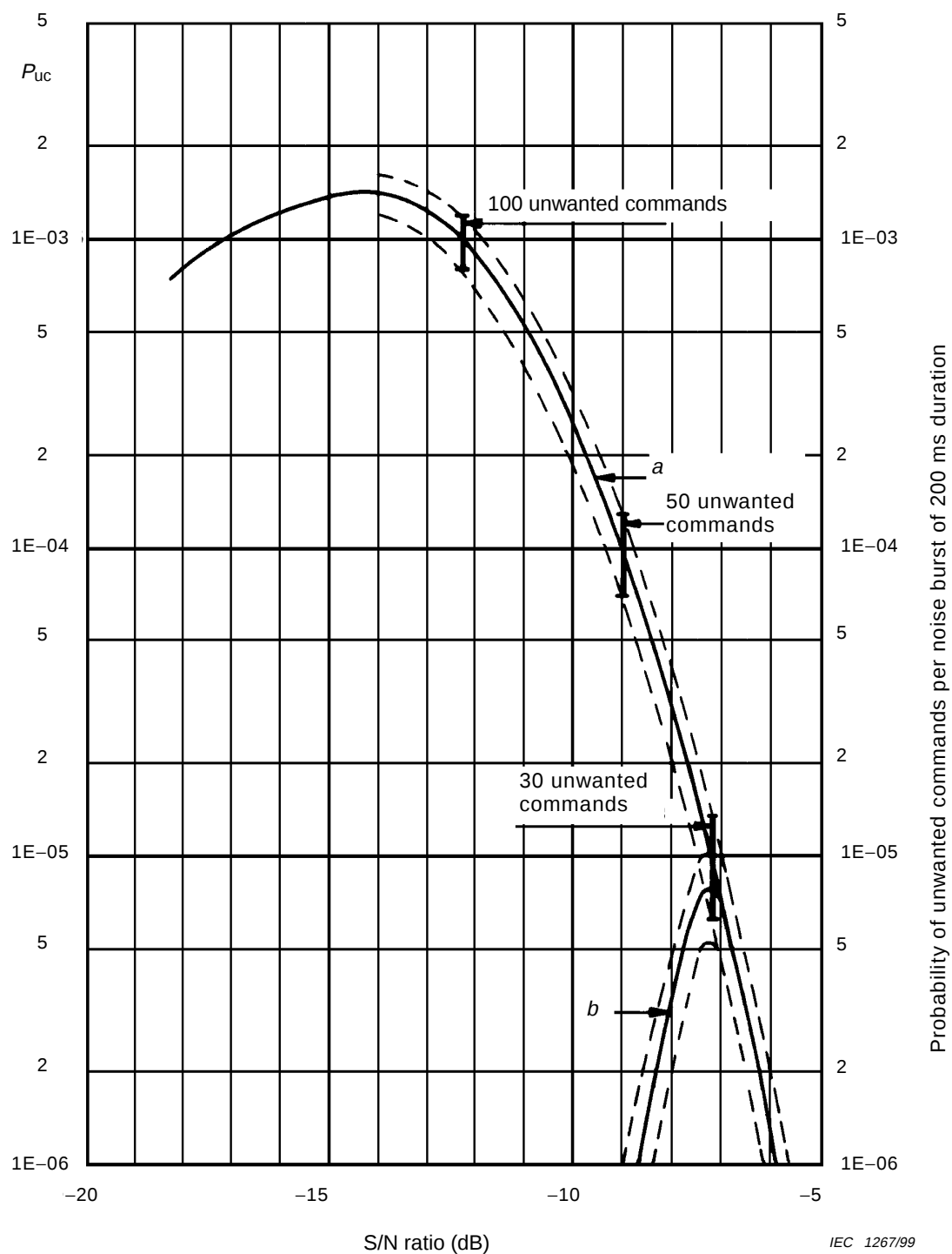
Figure A.2 – Examples of probability of unwanted commands versus signal-to-noise ratio for a 200 Bd channel
