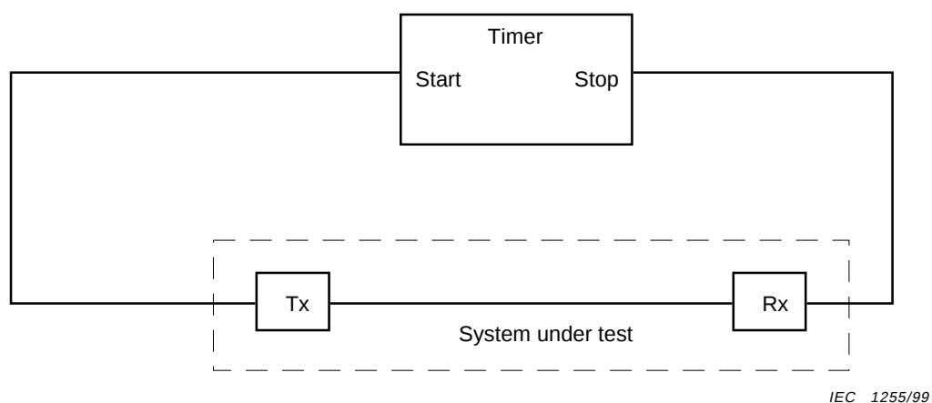
Figure 15 – Test set-up for measuring transmission time
