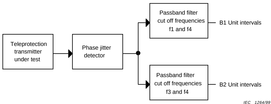
Figure 24 – Test set-up for measuring jitter at the output of a digital teleprotection transmitter
