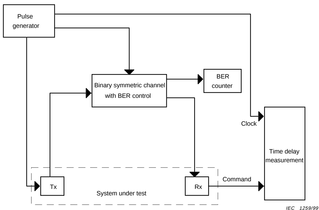
Figure 19 – Test set-up for recovery time measurement for digital teleprotection
