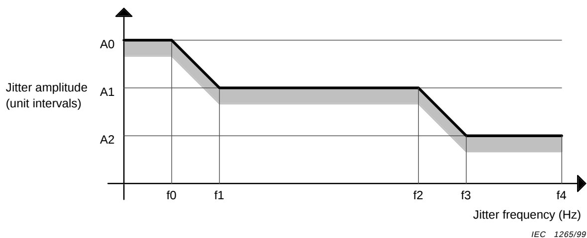
Figure 25 – Jitter mask for testing jitter at the input of a digital teleprotection receiver
