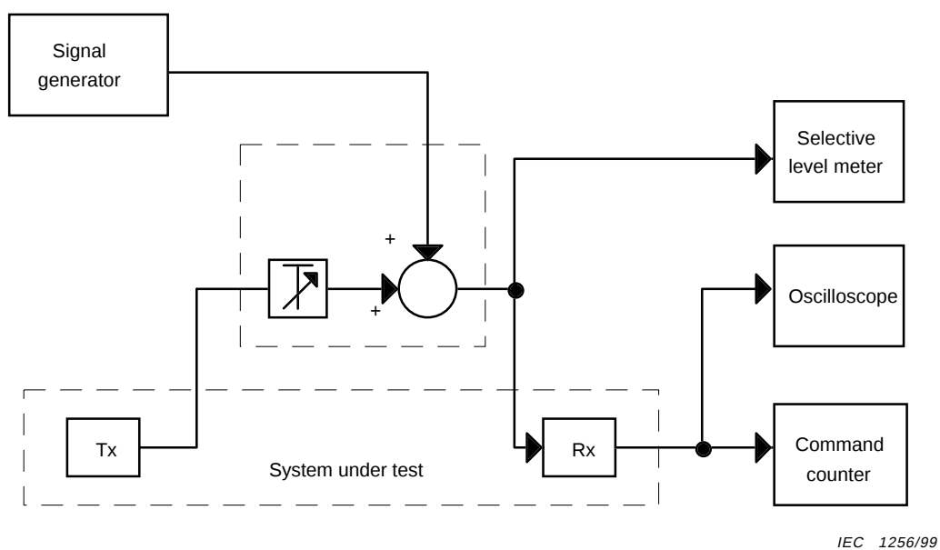
Figure 16 – Test set-up for measuring interference by discrete frequencies
