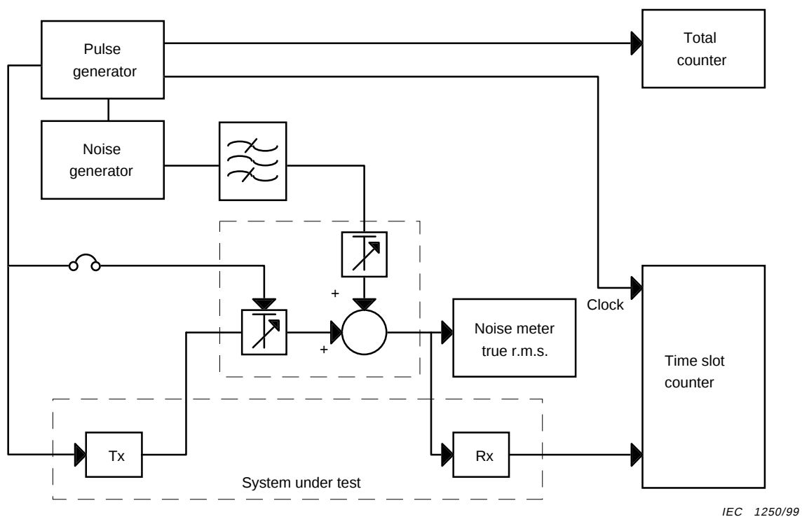
Figure 10 – Test set-up for dependability measurement (analogue teleprotection)
