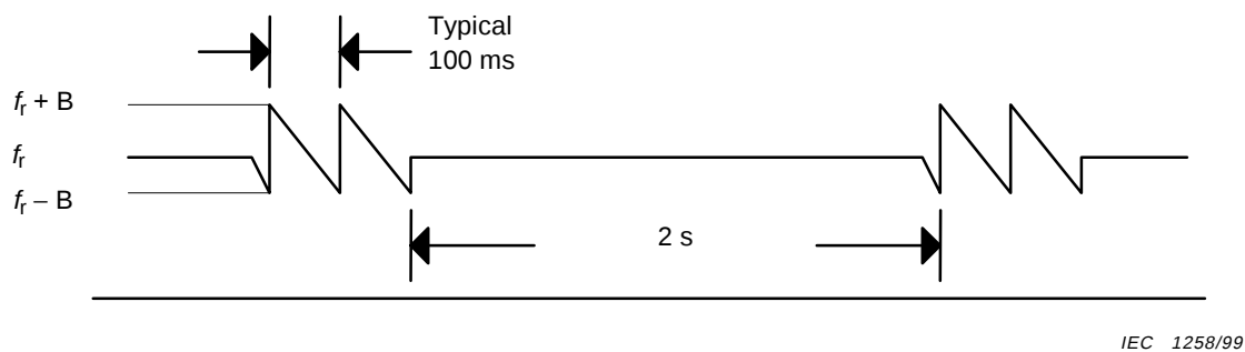
Figure 18 – Frequency deviation versus time for test set-up in figure 17
