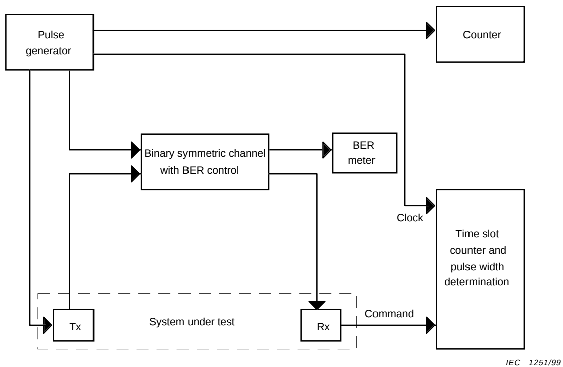
Figure 11 – Test set-up for dependability measurement (digital teleprotection)
