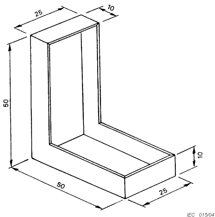
Figure 1 – Angle box with two rectangular cases
