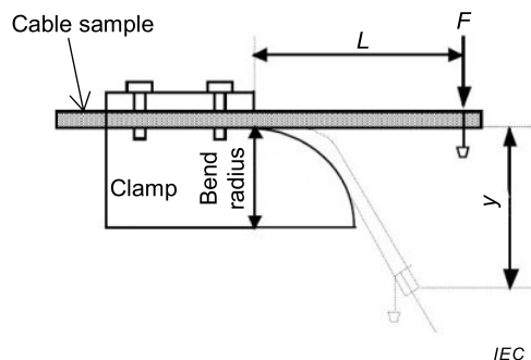
Figure 21b – Apparatus with control of radius
