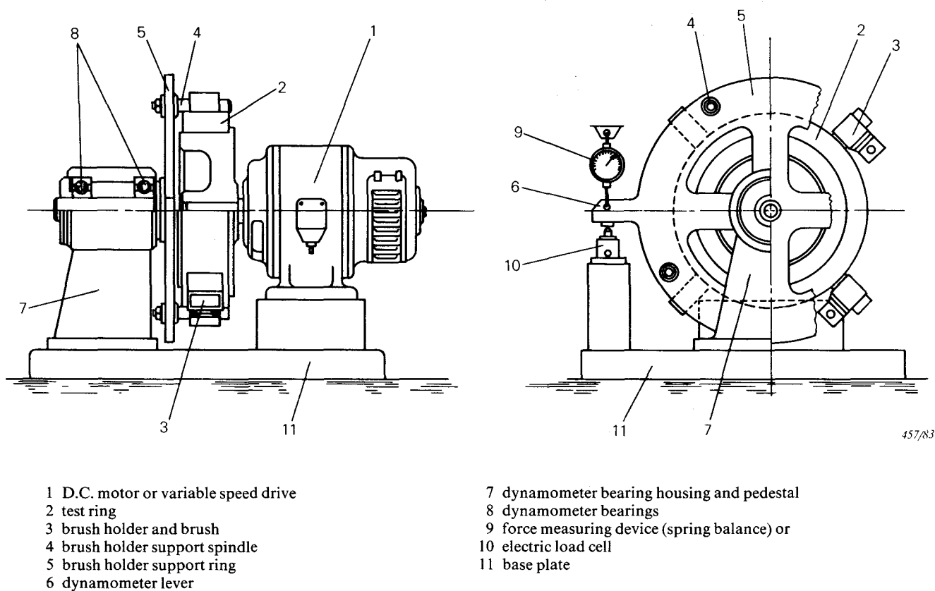
FIG. C1. - Brush test machine (dynamometer).
