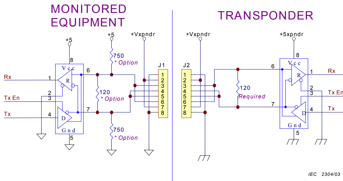
Figure 3 – Sample PSTIB RS-485 interface
