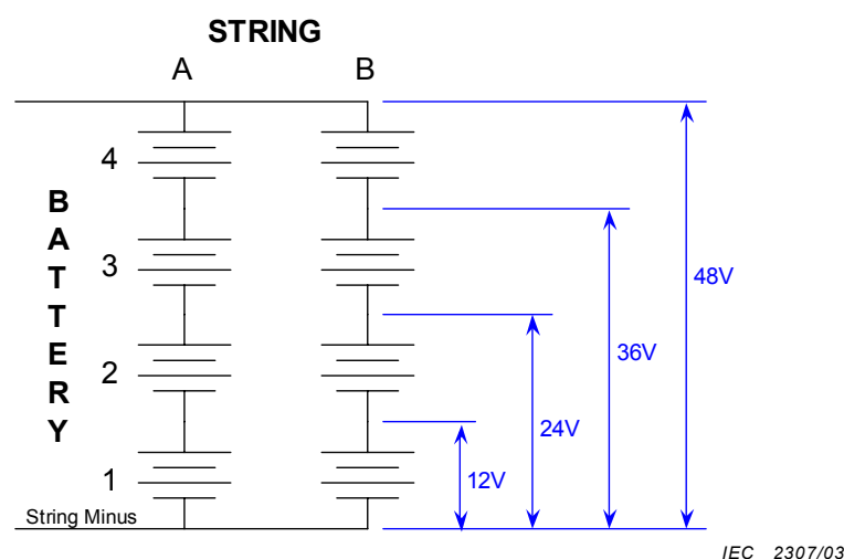
Figure 7 – Battery string naming conventions
