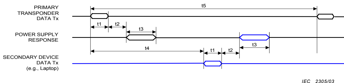
Figure 5 – PSTIB data and timing diagram
