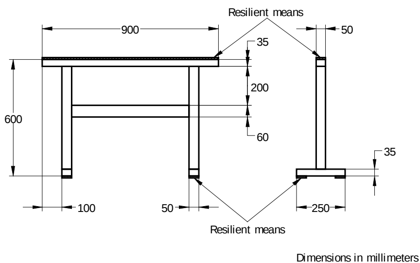
Figure 102 – Example of standard stand
